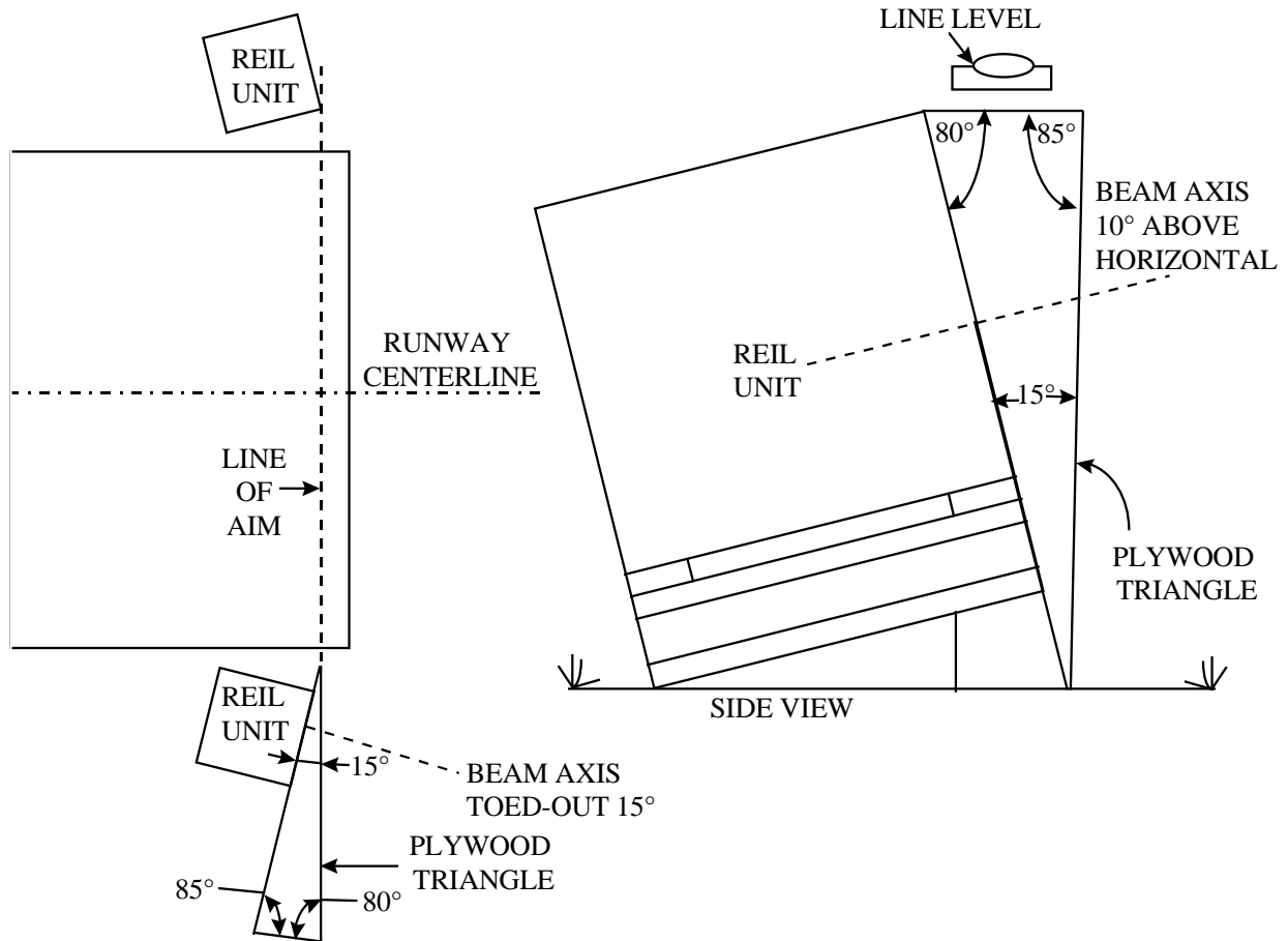
Figure 5-5. REIL Aiming
