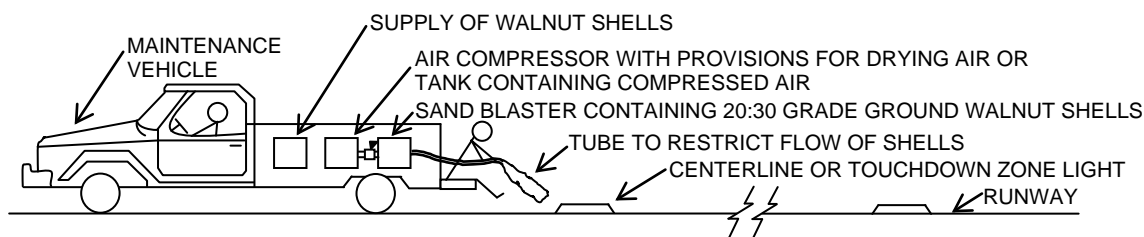
Figure 5-2 Cleaning Runway Centerline and Touchdown Zone Lights.
