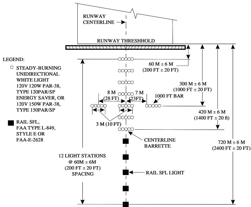
Figure 5-6. MALSR Configuration
