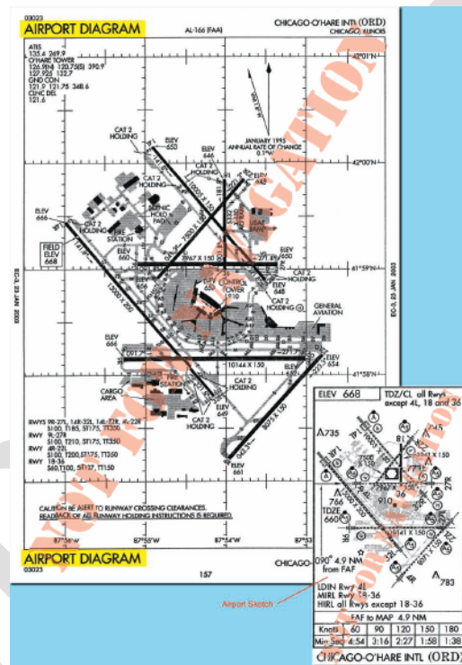
Figure 2-23. Paper chart.
