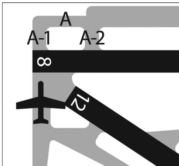
FIG 3-9-12 Runway/Taxiway Proximity
