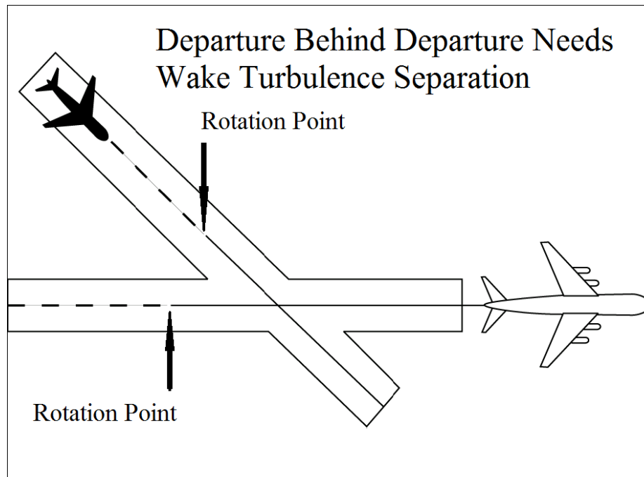
FIG 3-9-12 Departure Behind Departure on Intersecting Runway
