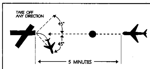
Separation Minima
