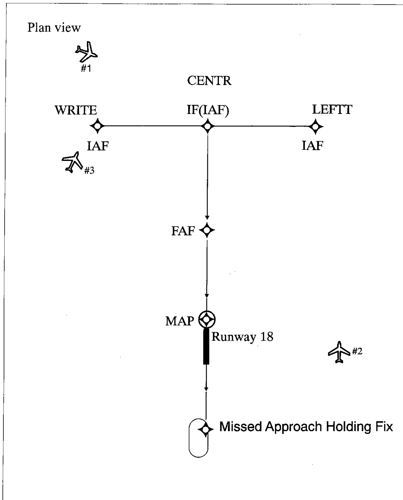
FIG 5-9-5 Basic "T" Design
