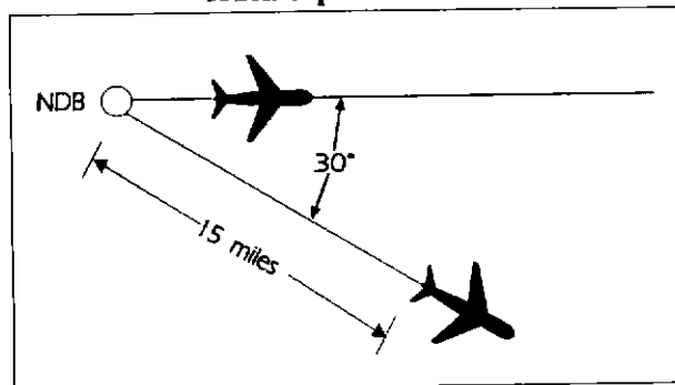
Track Separation NDB
