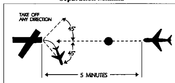
FIG 6-3-2 Separation Minima
