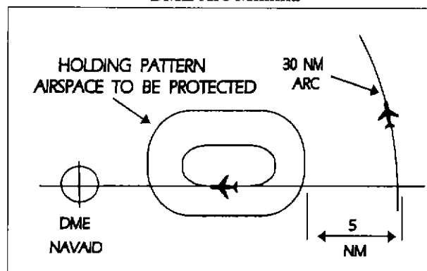
DME Arc Minima
