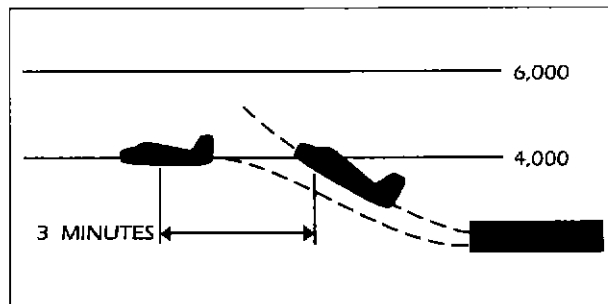
FIG 6-2-8 Minima on Same Course
