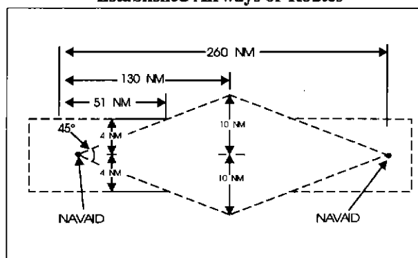
Minima Along Other Than Established Airways or Routes
