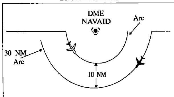
FIG 6-5-2 DME Arc Minima
