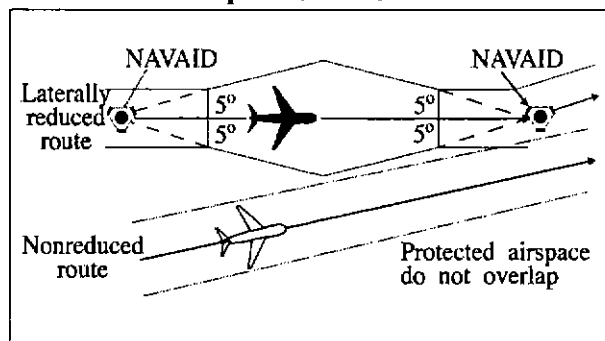
FIG 8-4-2 Separation Methods
