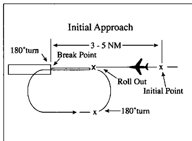
FIG 3-10-13 Overhead Maneuver
