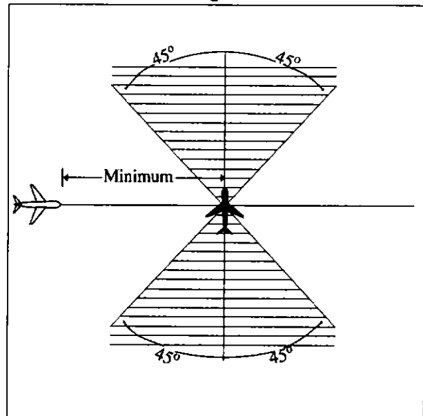
Crossing Courses
