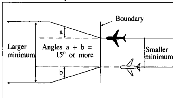
FIG 8-4-3 Separation Methods
