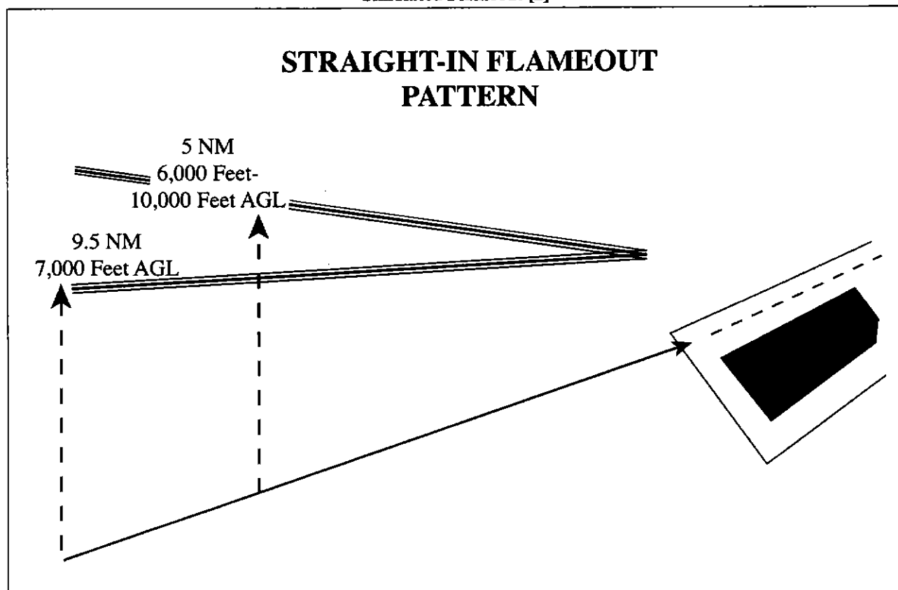
FIG 3-10-15 Simulated Flameout [2]
