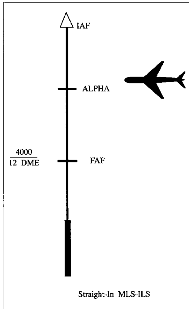
FIG 5-9-2 Arrival Instructions
