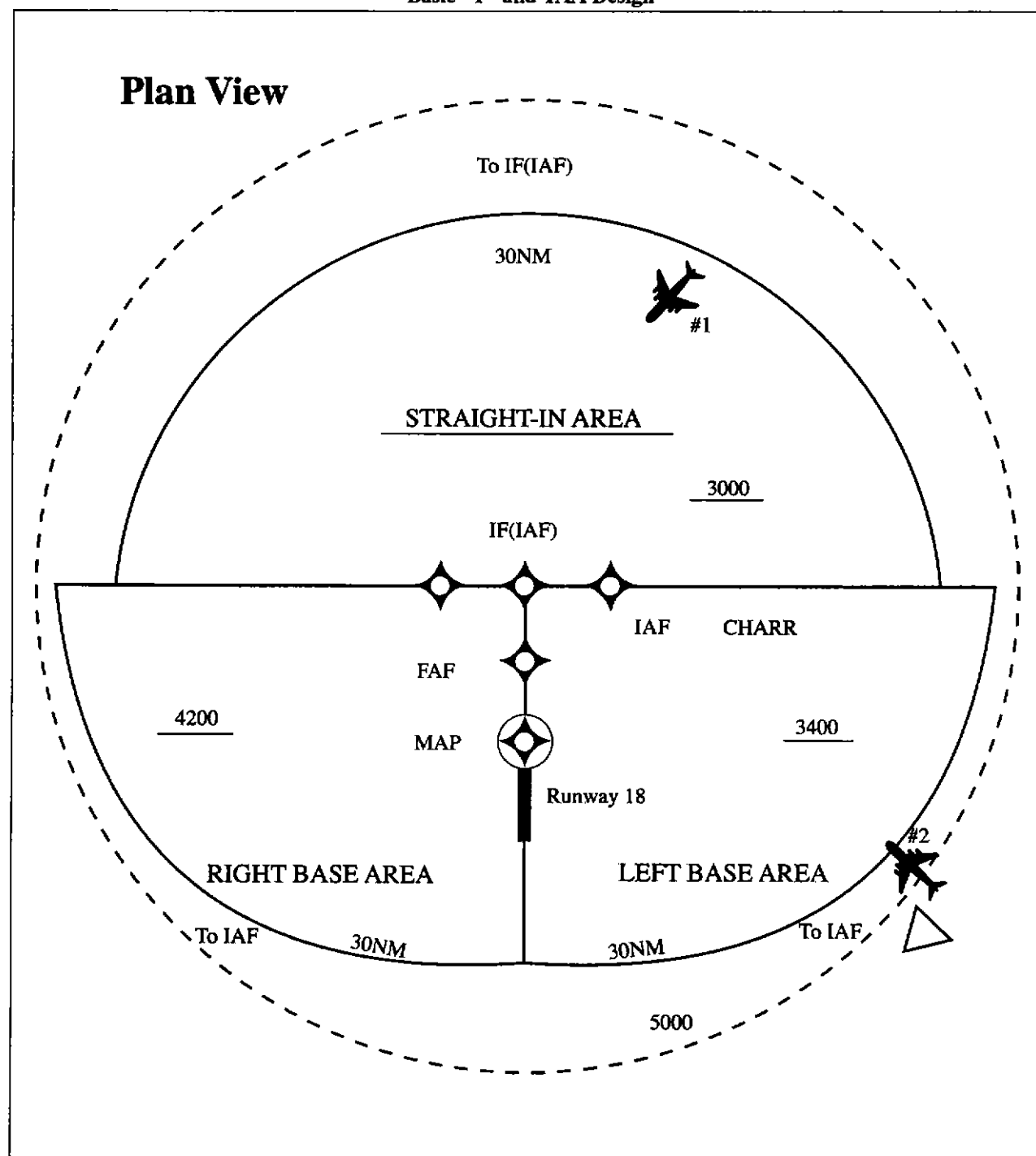
FIG 4-8-2 Basic "T" and TAA Design
