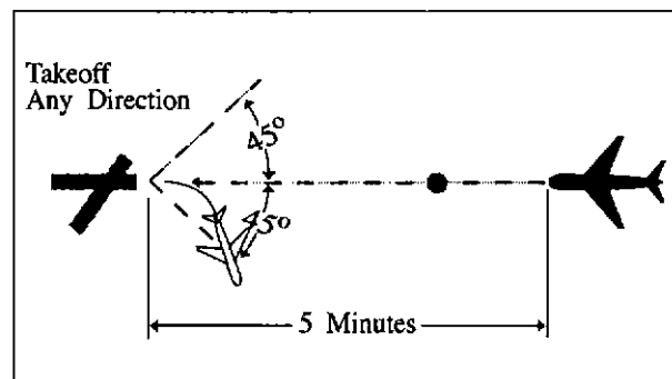
FIG 6-3-2 Separation Minima
