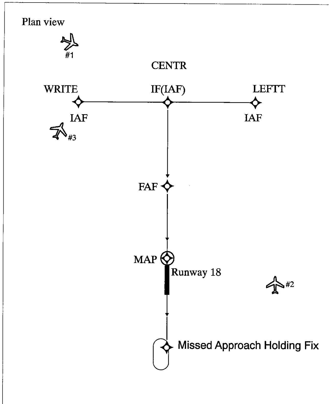
FIG 5-9-5 Basic "T" Design
