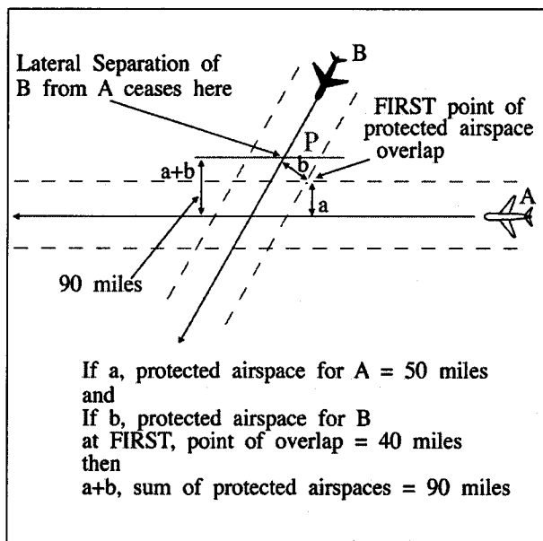
FIG 8-4-6 Separation Methods
