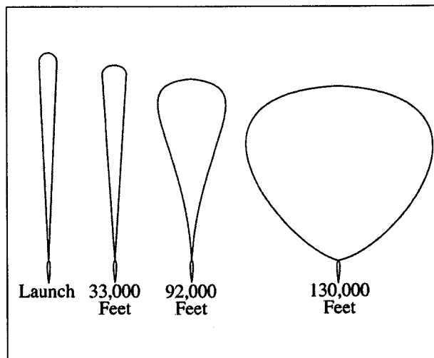
FIG 9-7-1 Shapes of 11 Million Cubic Feet Balloon at Various Altitudes
