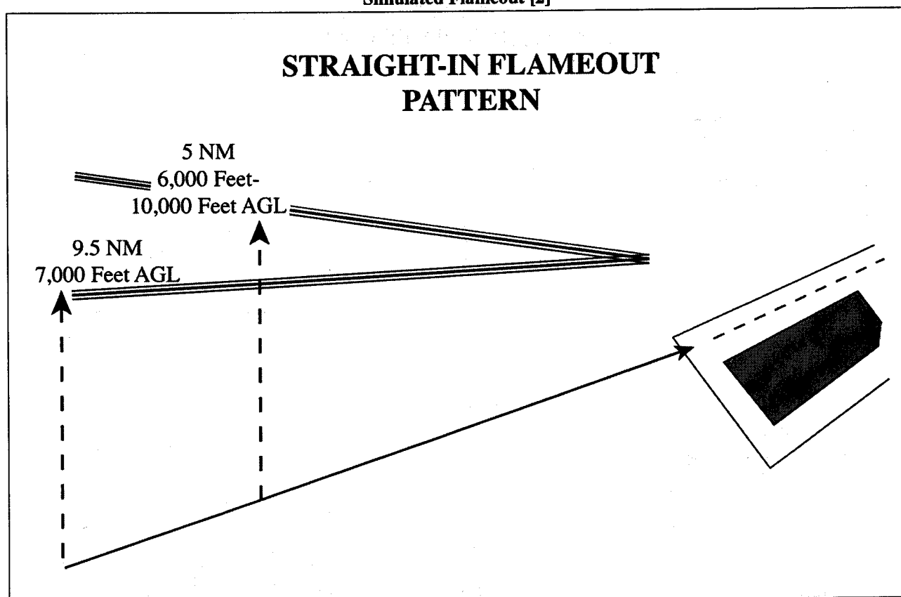
FIG 3-10-15 Simulated Flameout [2]
