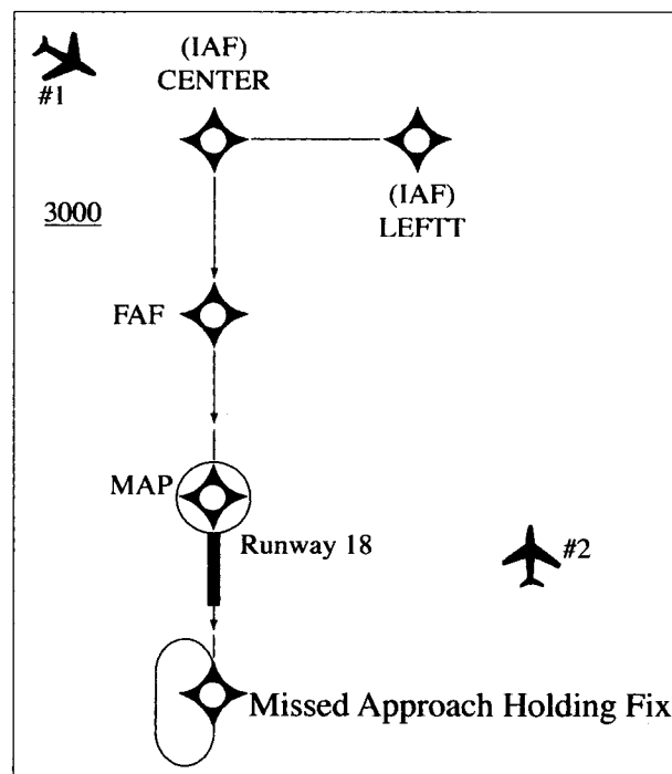
FIG 4-8-2 Approach Clearance Example For RNAV Aircraft
