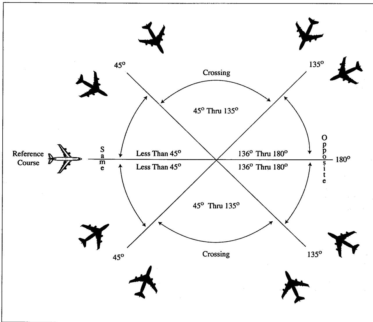
FIG 1-2-1 Divergence
