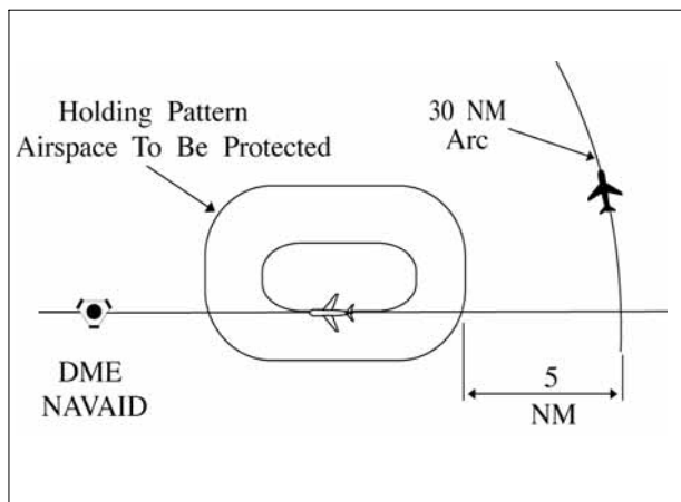
FIG 6-5-3 DME Arc Minima
