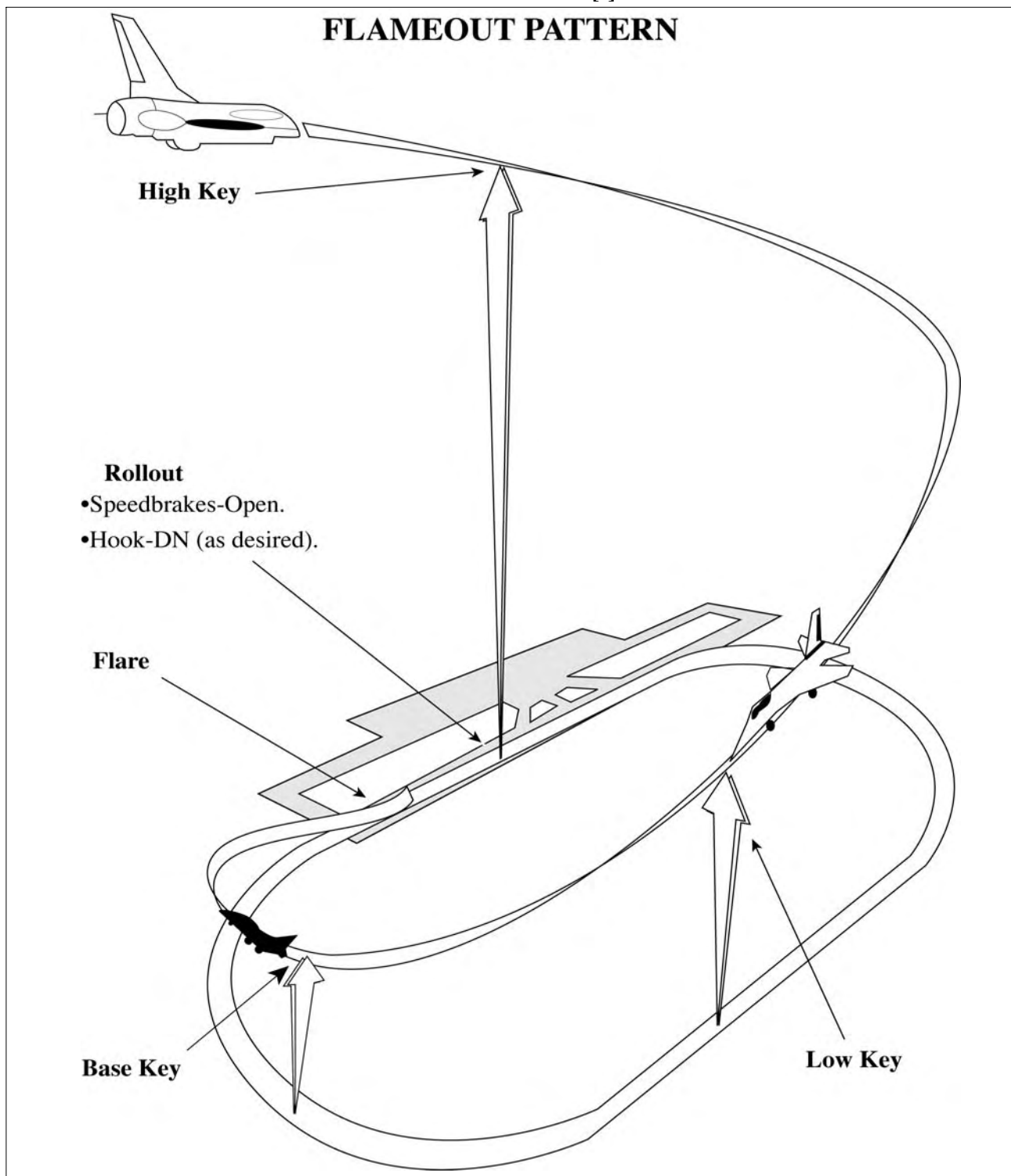
FIG 3-10-14 Simulated Flameout [1]
