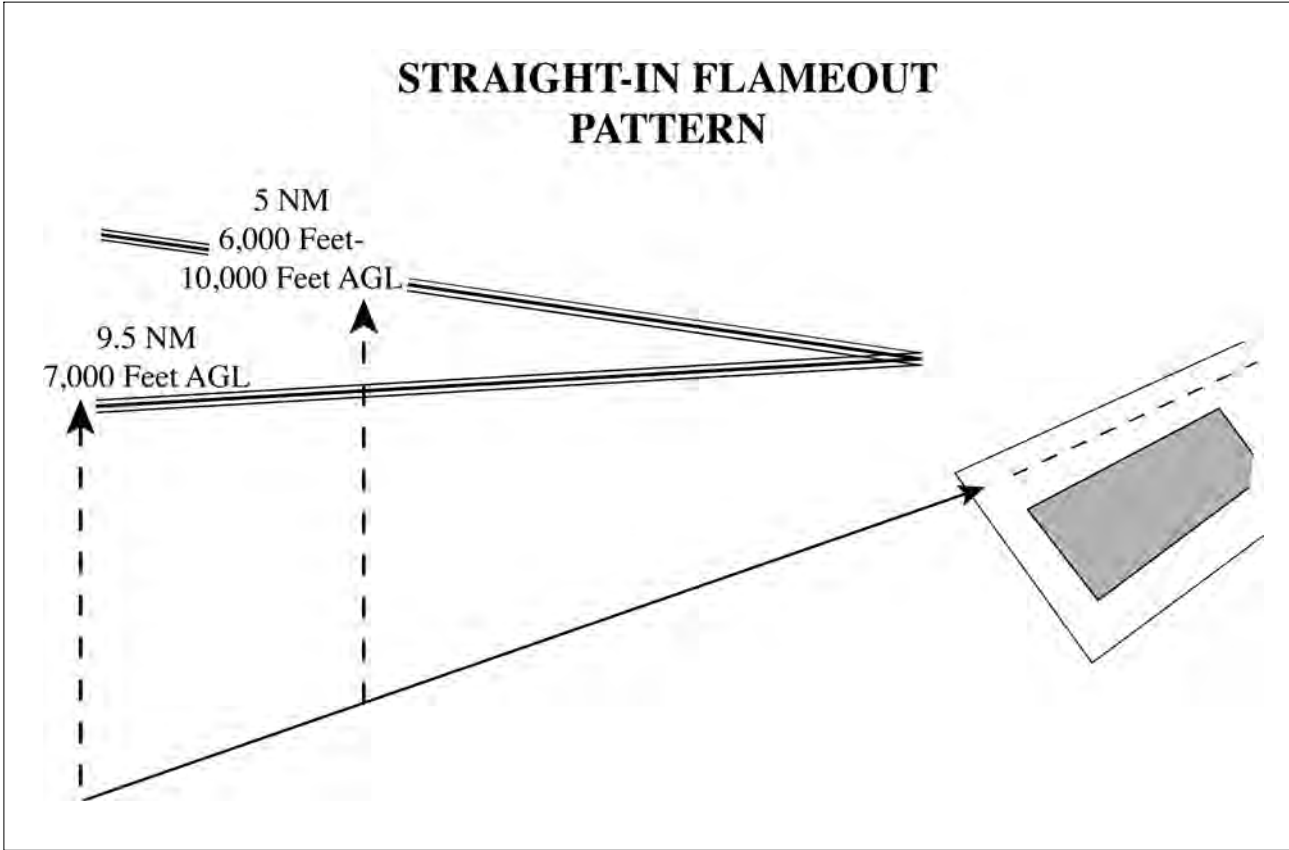
FIG 3-10-15 Simulated Flameout [2]
