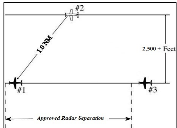
FIG 5-9-7 Simultaneous Dependent Approaches
