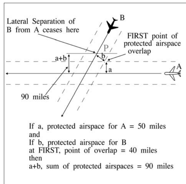
FIG 8-4-6 Separation Methods
