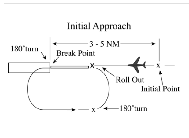
FIG 3-10-13 Overhead Maneuver
