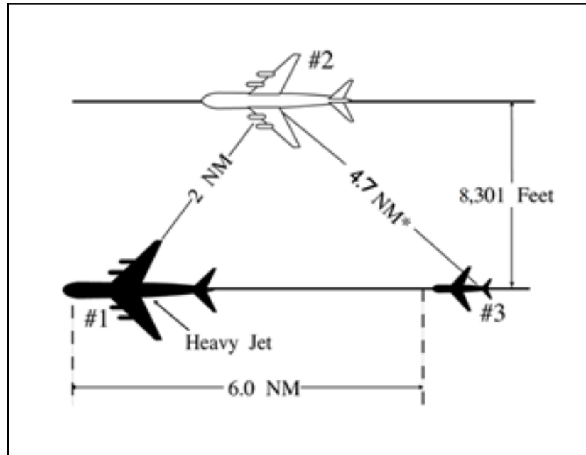
FIG 5-9-6 Simultaneous Dependent Approaches
