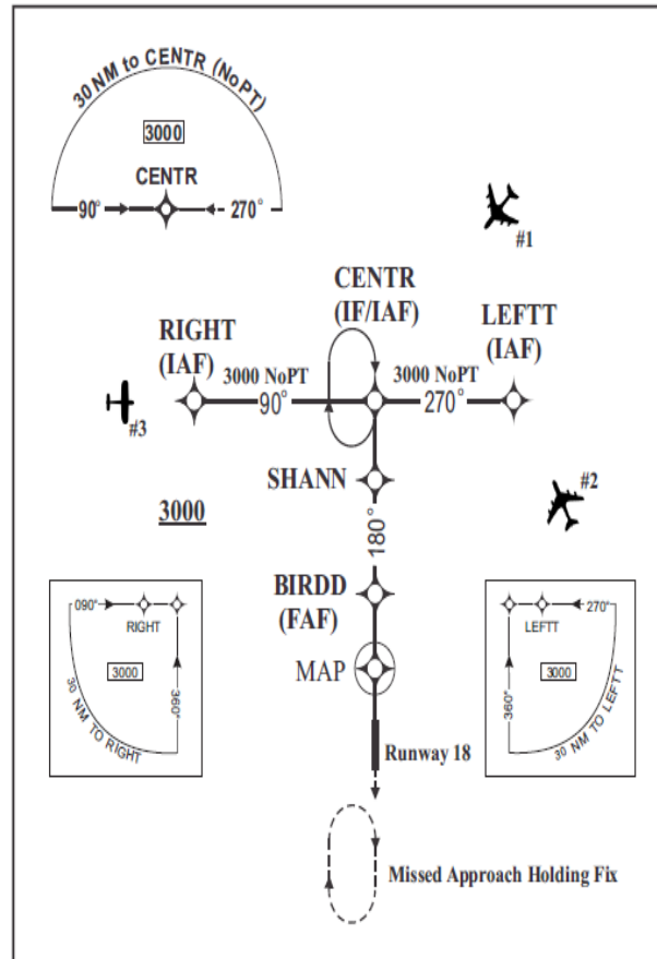
FIG 5-9-3 Basic “T” Design
