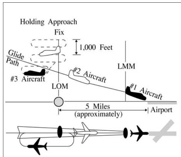
Timed Approach Procedures Using ILS and Longitudinal Separation Only
