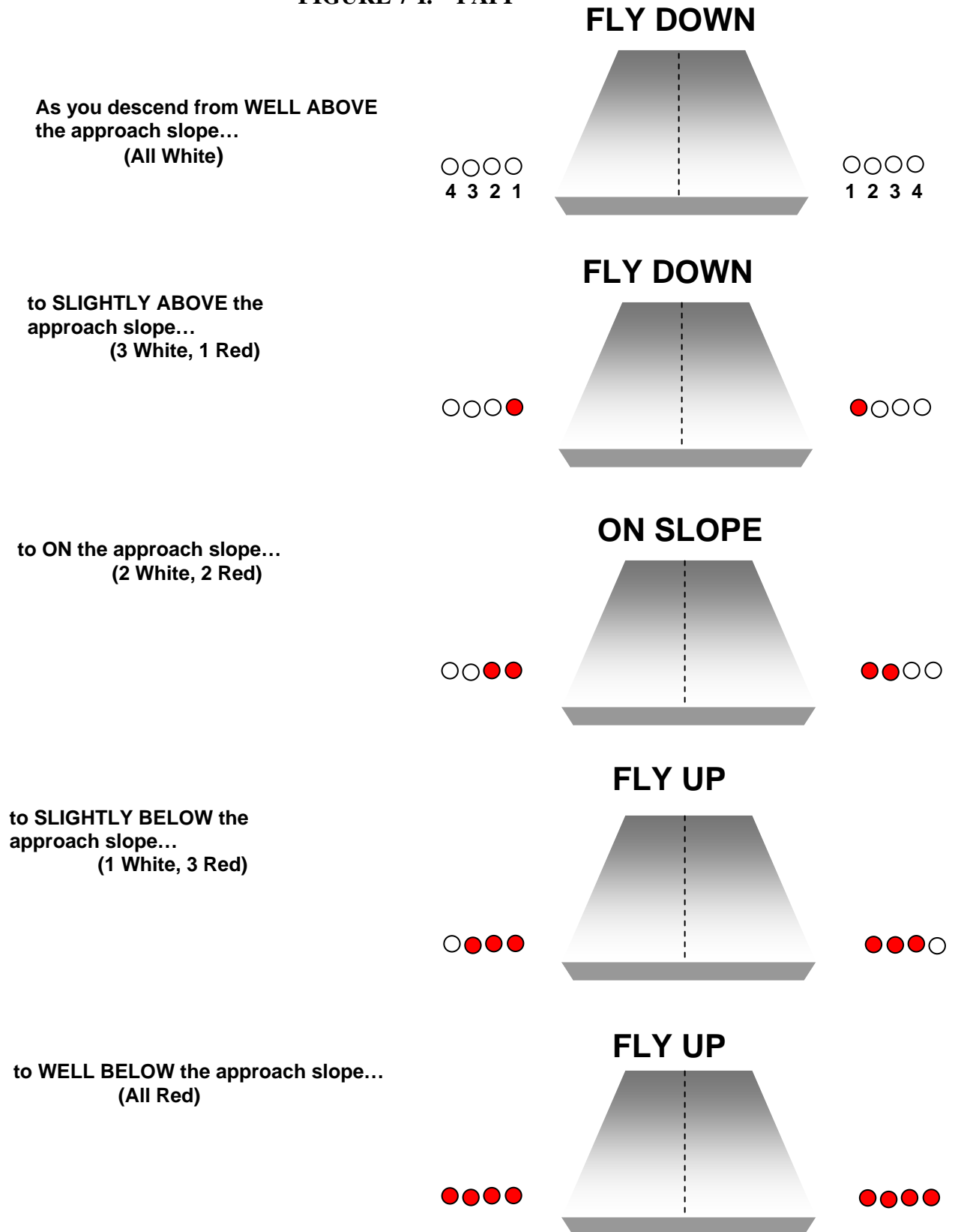
FIGURE 7-I. PAPI
