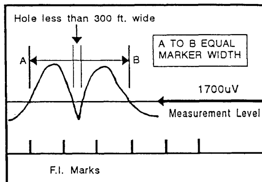
Figure 15-8B 75 MHz Marker Width Measurement A to B Equals Width (includes the hole)
