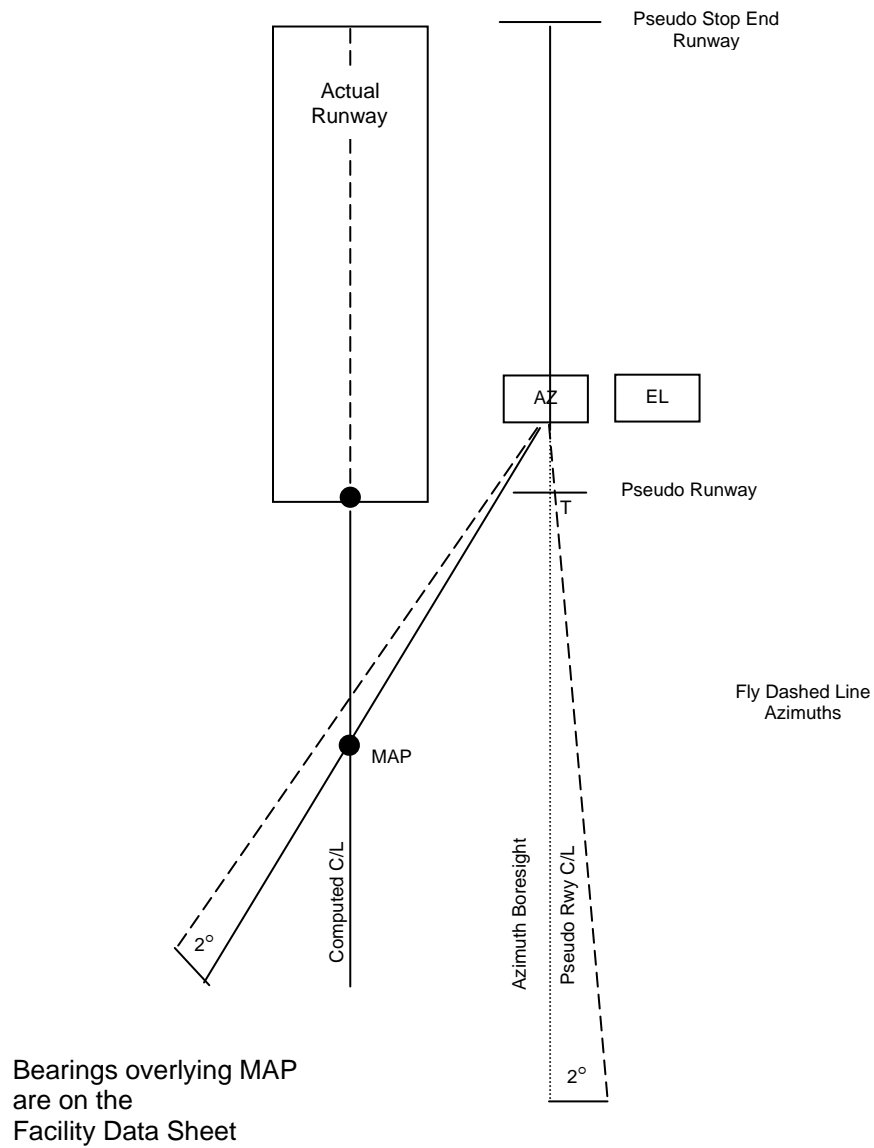
Figure 16-8 AZIMUTHS FOR COVERAGE BELOW PATH (COMPUTED CENTERLINE FACILITIES)
