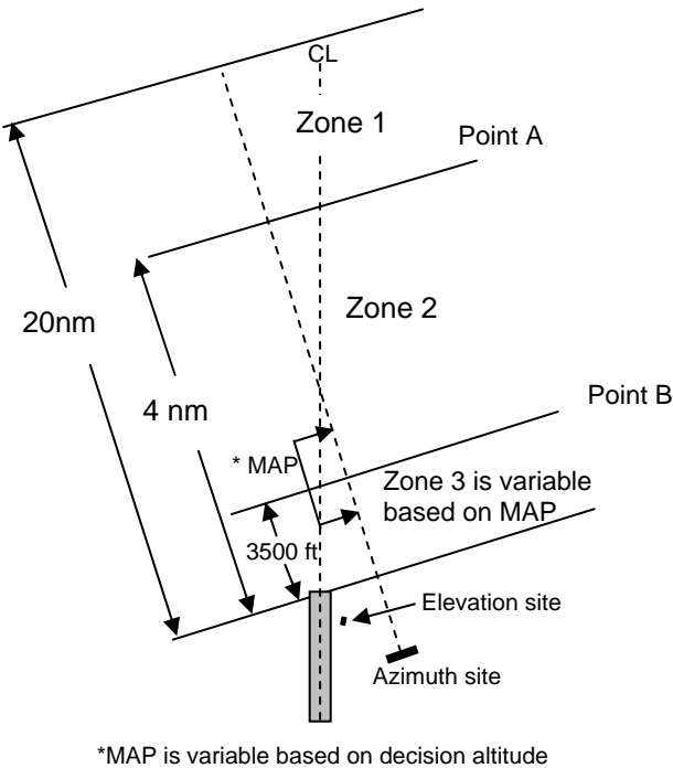
Figure 16-4 OFFSET MLS
