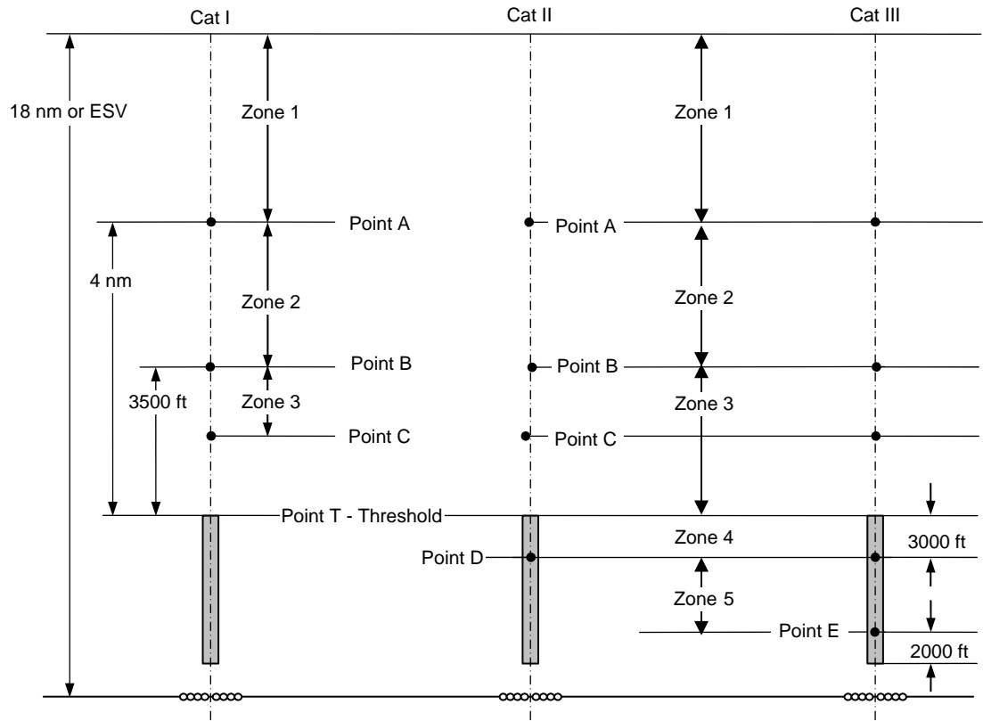
Figure 15-1A(2) TYPICAL OFFSET ILS
