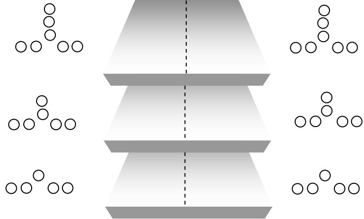
FIGURE 7-K T-VASI's FLY DOWN
