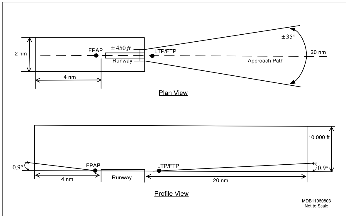
Figure 17-4 Approach Coverage Requirements
