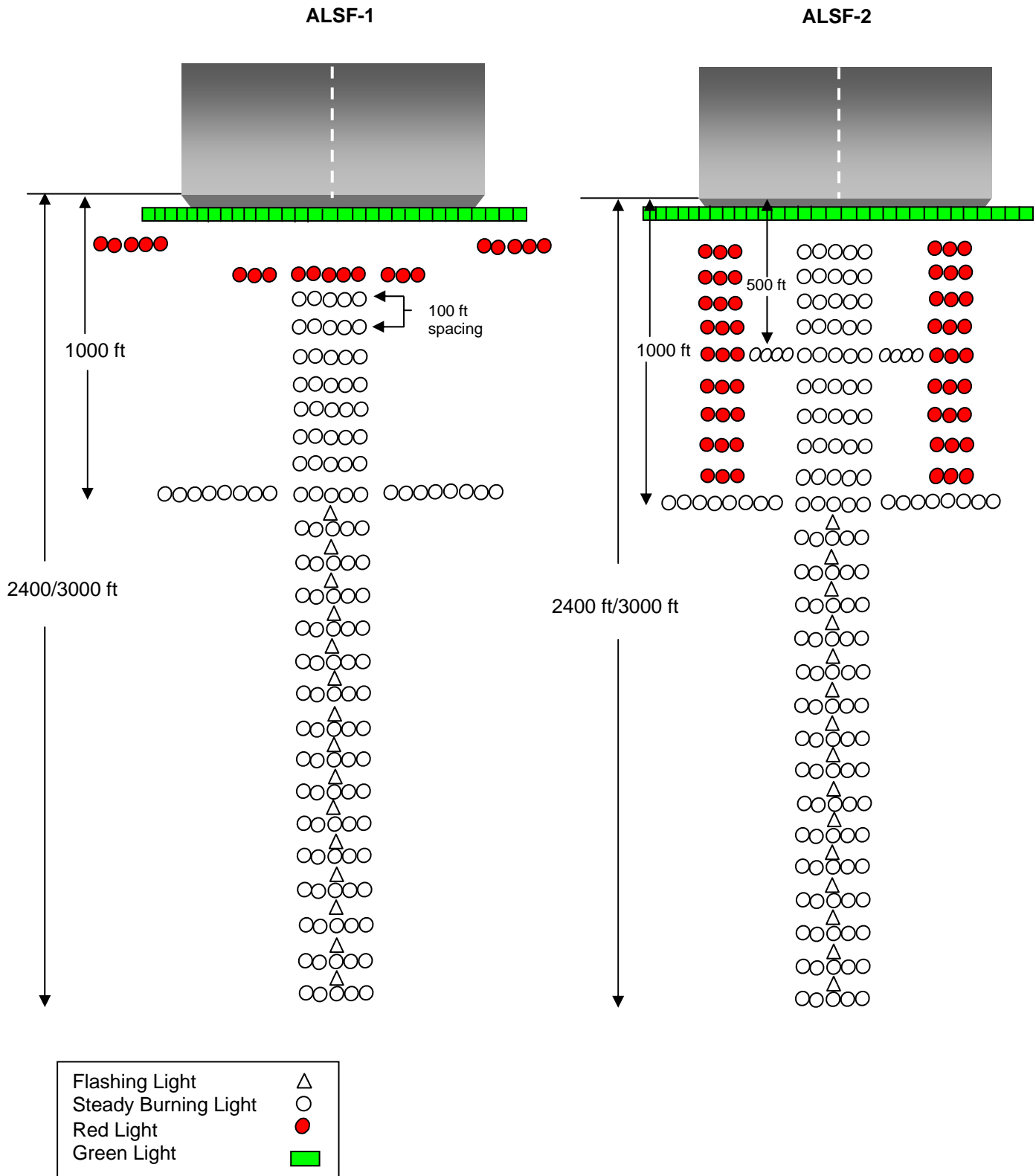
Figure 7-O LIGHTING SYSTEM CONFIGURATIONS
