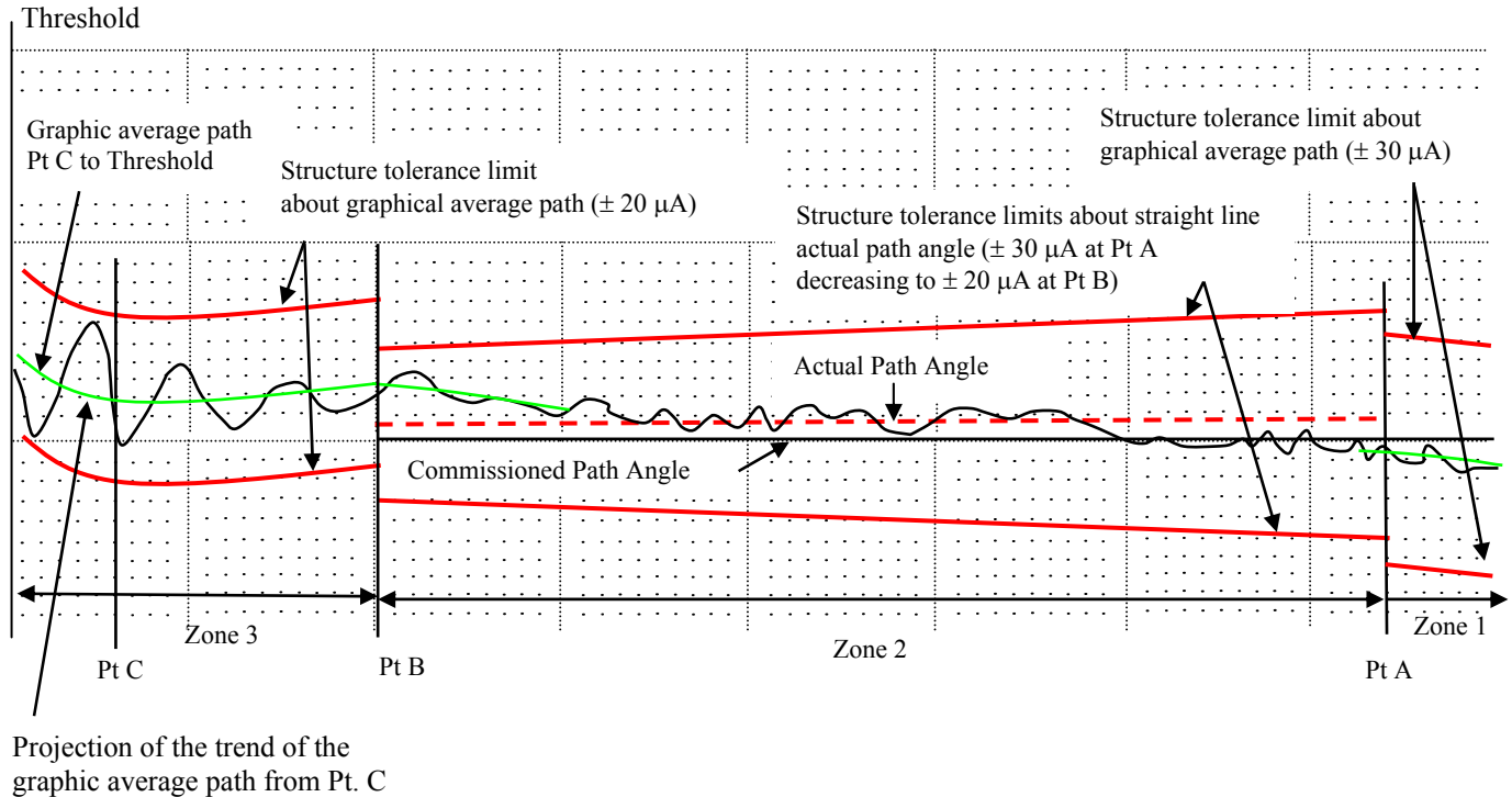
Figure 15-10 RATE OF CHANGE/REVERSAL IN THE SLOPE OF THE GLIDE PATH
