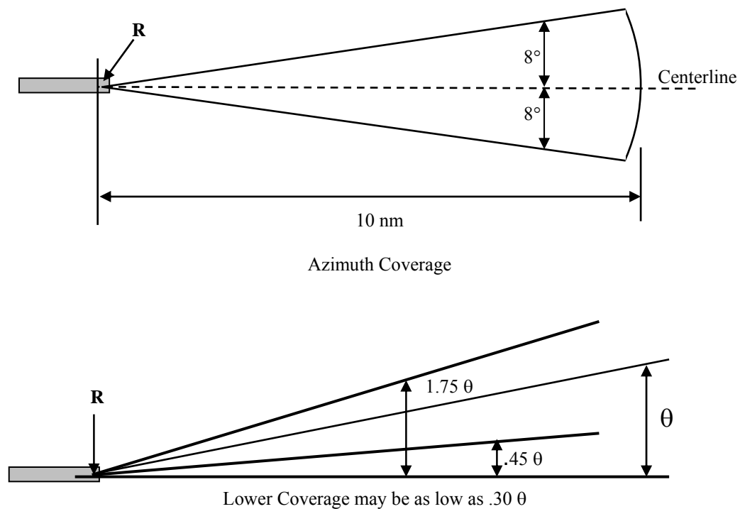
Figure 15-12 GLIDE SLOPE STANDARD SERVICE VOLUME
