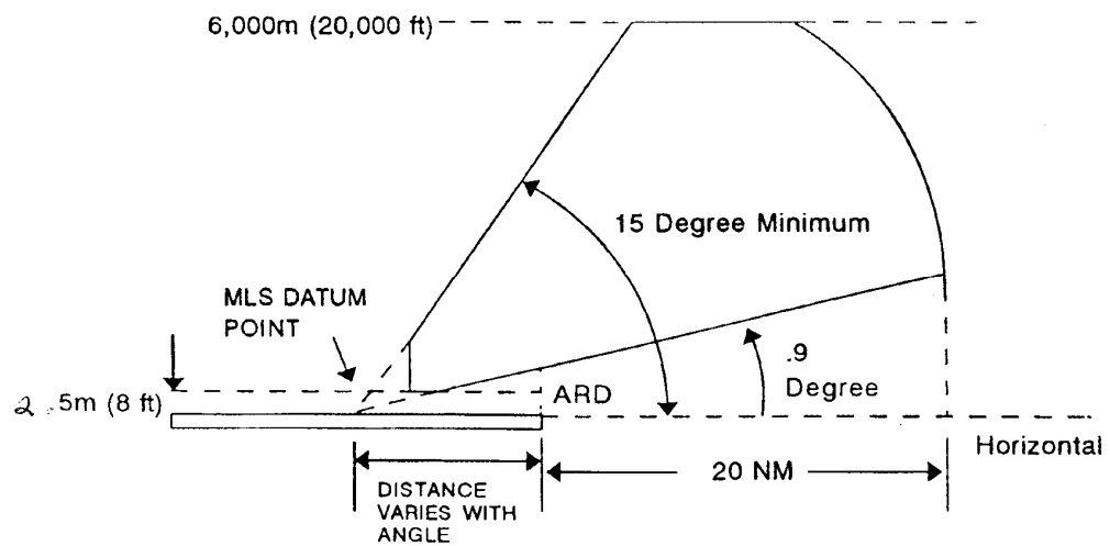
VERTICAL COVERAGE
