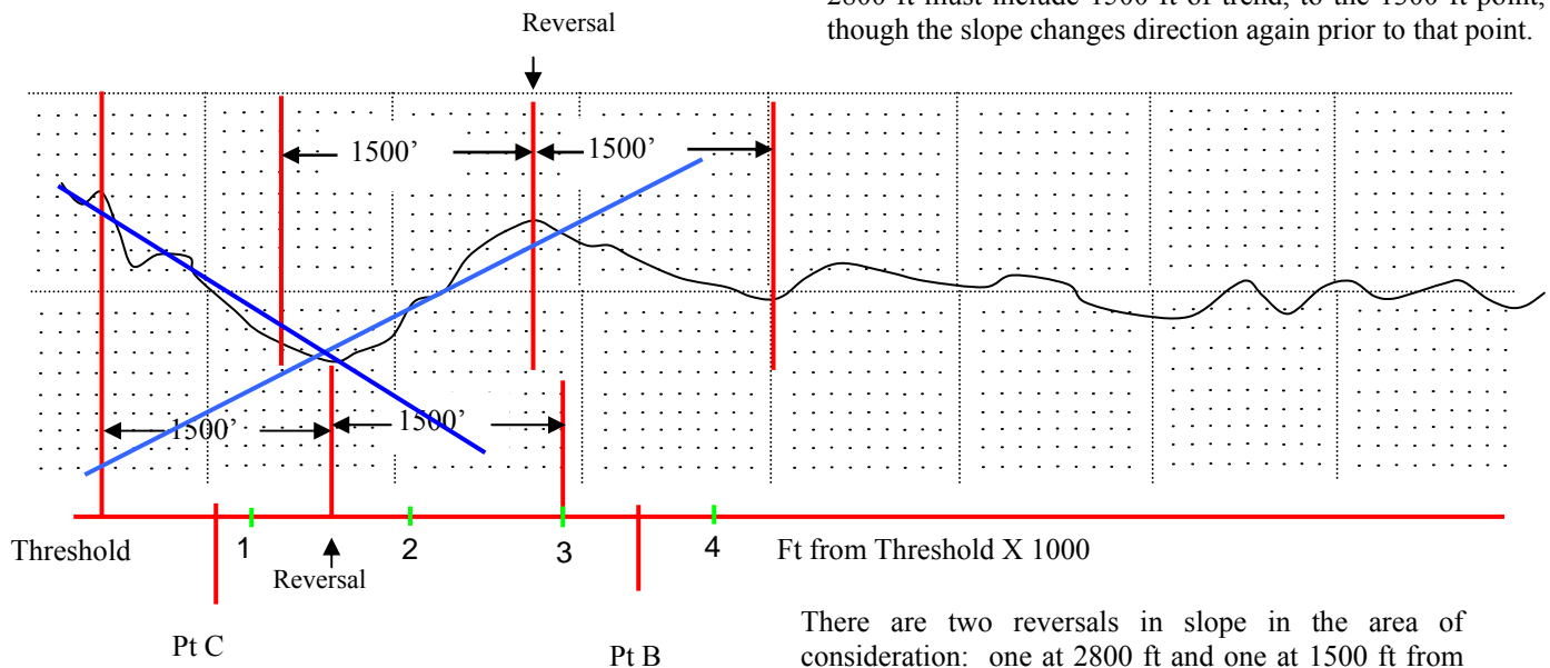
Figure 15-10 RATE OF CHANGE/REVERSAL IN THE SLOPE OF THE GLIDE PATH
