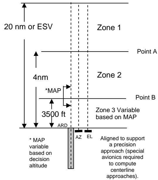
Figure 16-5 COLLOCATED MLS
