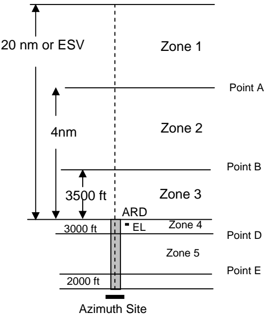
Figure 16-4 OFFSET MLS
