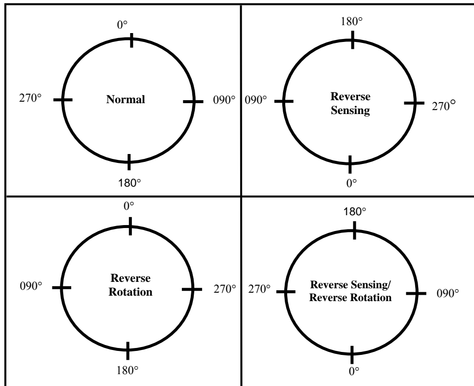
Figure A3-6B. TACAN Sensing and Rotation
