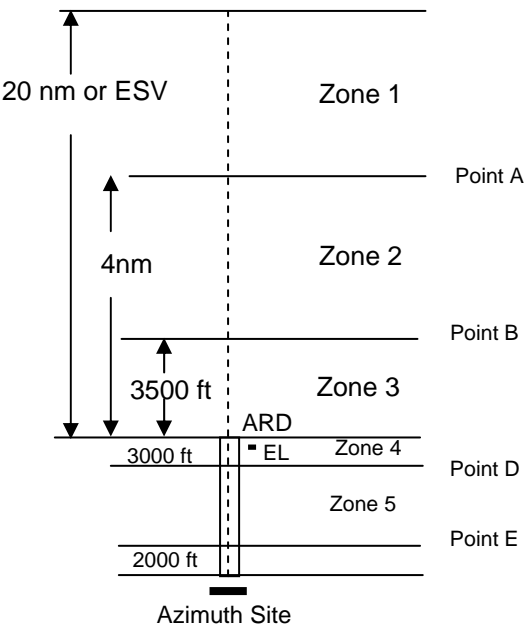
Figure 16-4 OFFSET MLS
