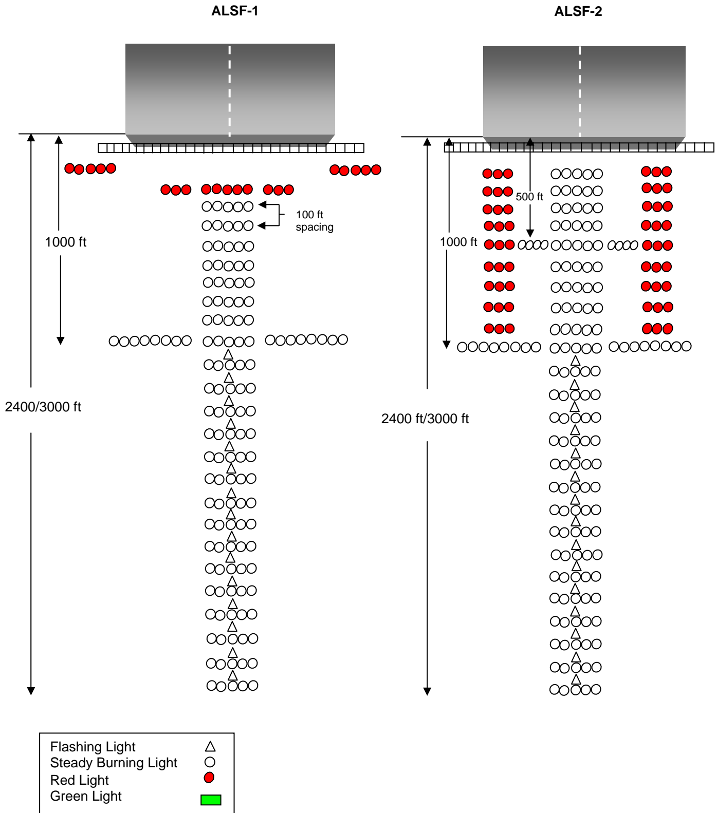
Figure 7-O LIGHTING SYSTEM CONFIGURATIONS
