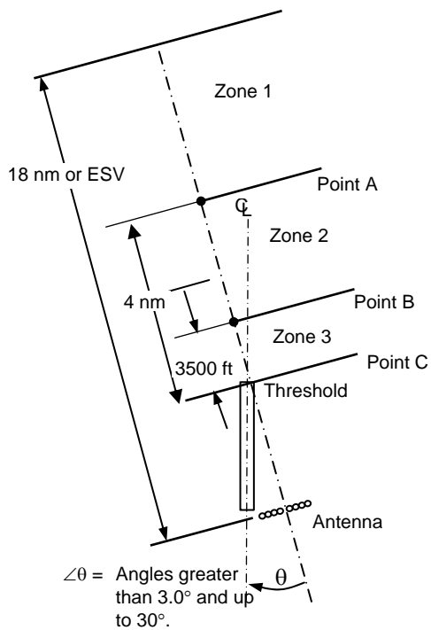
Figure 15-1B(3) Back Course Localizer/ SDF
