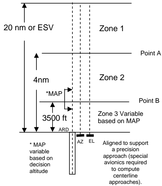
Figure 16-5 COLLOCATED MLS
