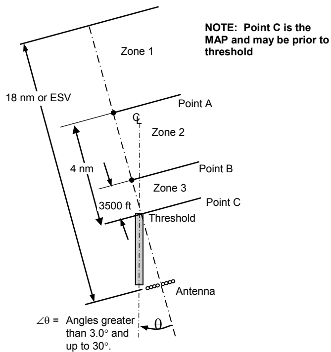
Figure 15-1B(1). LDA Configuration.
