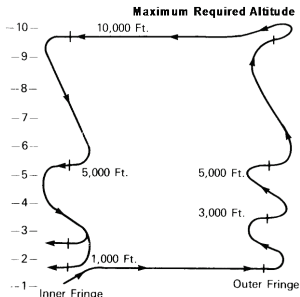
Figure 14-3. Antenna Change--ASR/ ATCRBS.
