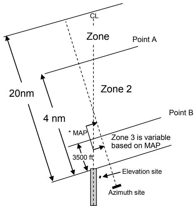
Figure 16-4. Offset MLS.
