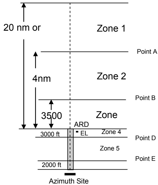
Figure 16-4. Offset MLS.
