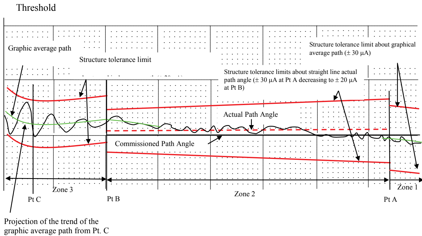
Figure 15-9. Application of Structure Tolerance -- CAT. II & III.
