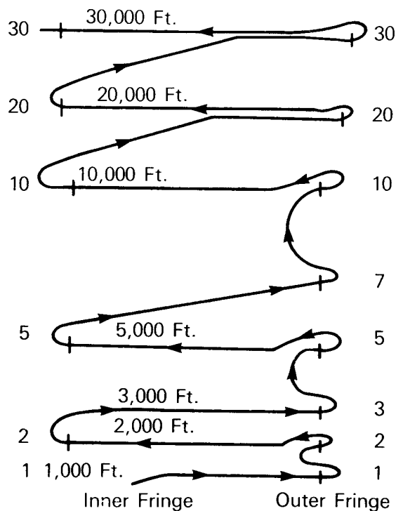
Figure 14-2. ARSR/ ATCRBS Vertical Coverage Profile.
