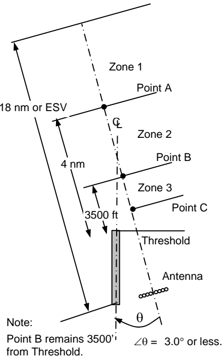
Figure 15-1A(2) TYPICAL OFFSET ILS
