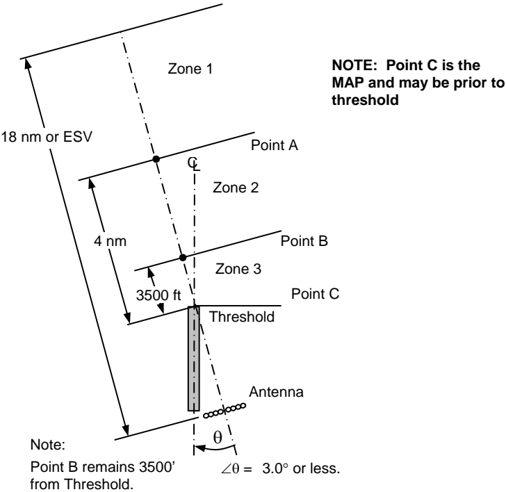
Figure 15-1A(3) TYPICAL OFFSET LOCALIZER
