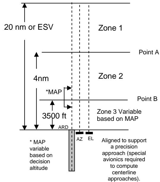
Figure 16-5 COLLOCATED MLS
