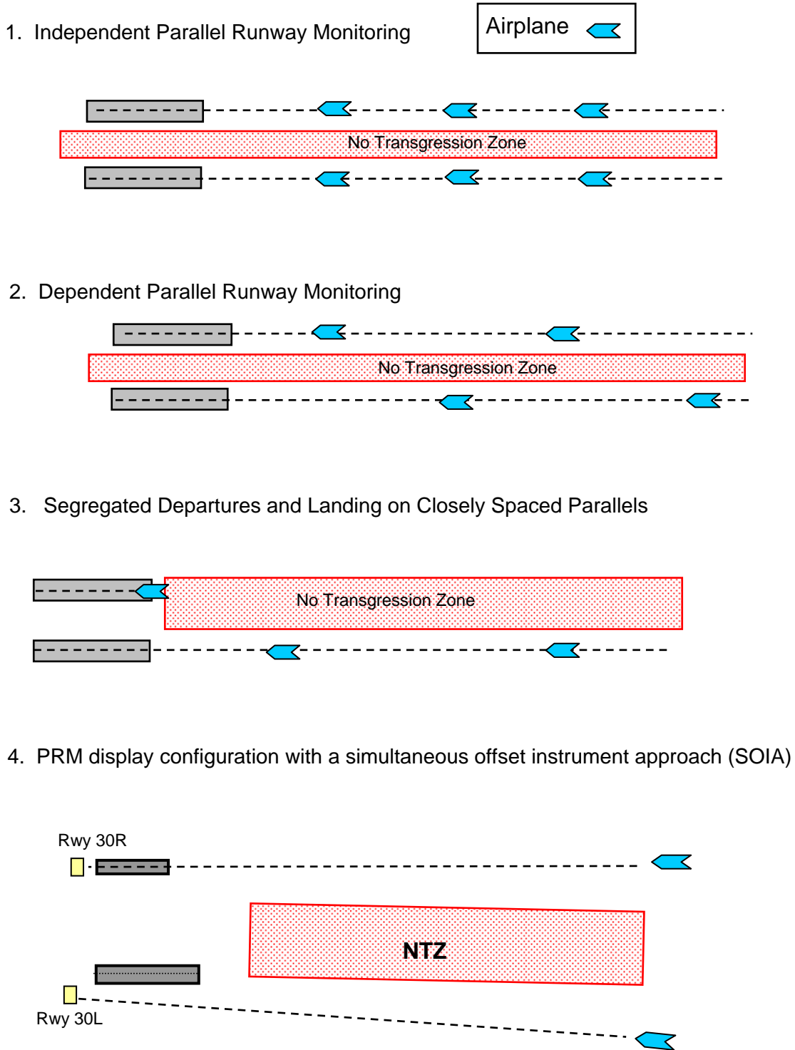
Figure A3-5 POSSIBLE PRM APPLICATIONS
