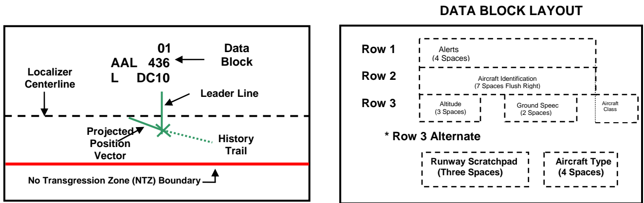
Figure A3-4 TRACK SYMBOLS AND DATA BLOCK FIELDS
