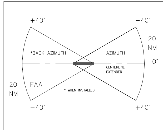
Figure 2-4. MLS AZIMUTH COVERAGE
