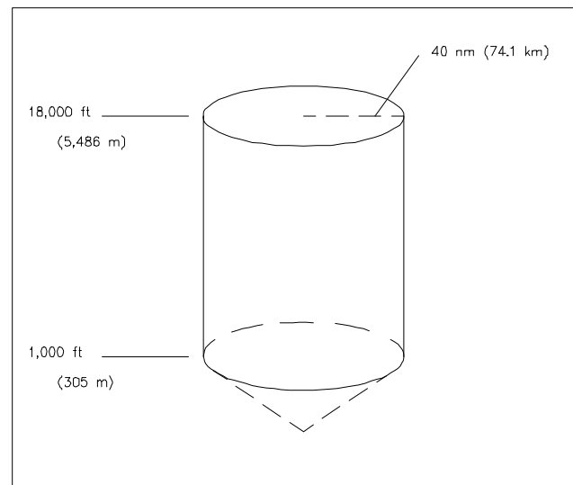
Figure 2-2. STANDARD LOW ALTITUDE SERVICE VOLUME
