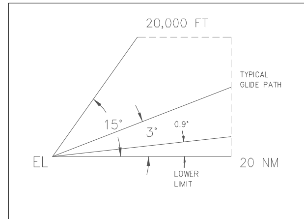
Figure 2-5. MLS ELEVATION COVERAGE
