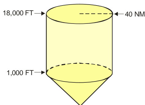
Figure 2-3. Standard Terminal Service Volume.
