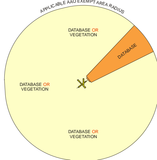
Figure 2-7F. AC 150/5300-18 Survey Area.
