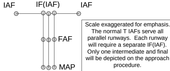
Figure 1D. BASIC T Parallel Runway Application
