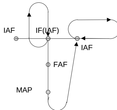
Figure 2B. Missed Approach Holding at an IAF
