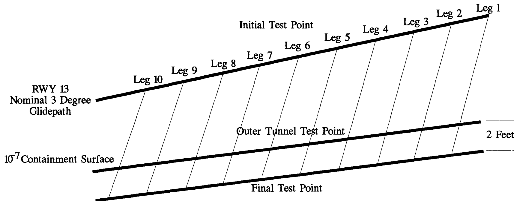
Figure 2.5-6 Vertical Containment Surface
