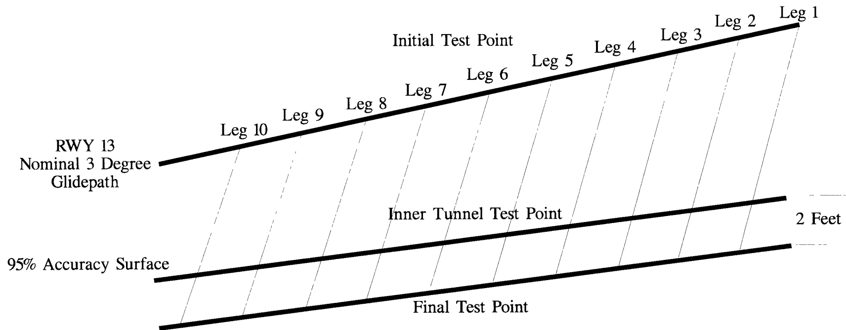
Figure 2.5-5 95% Vertical Accuracy Surface
