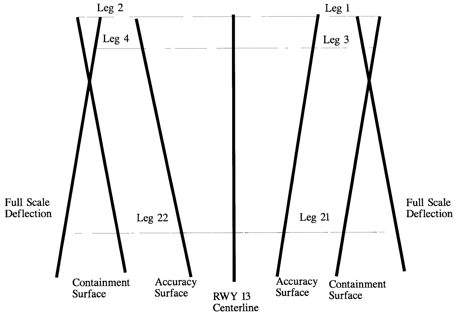
Figure 2.5-2 Horizontal Boundary Test
