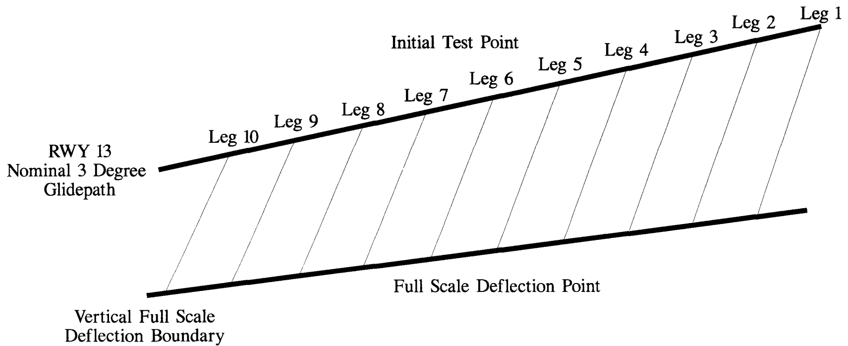
Figure 2.5-3 Vertical Full Scale Deflection
