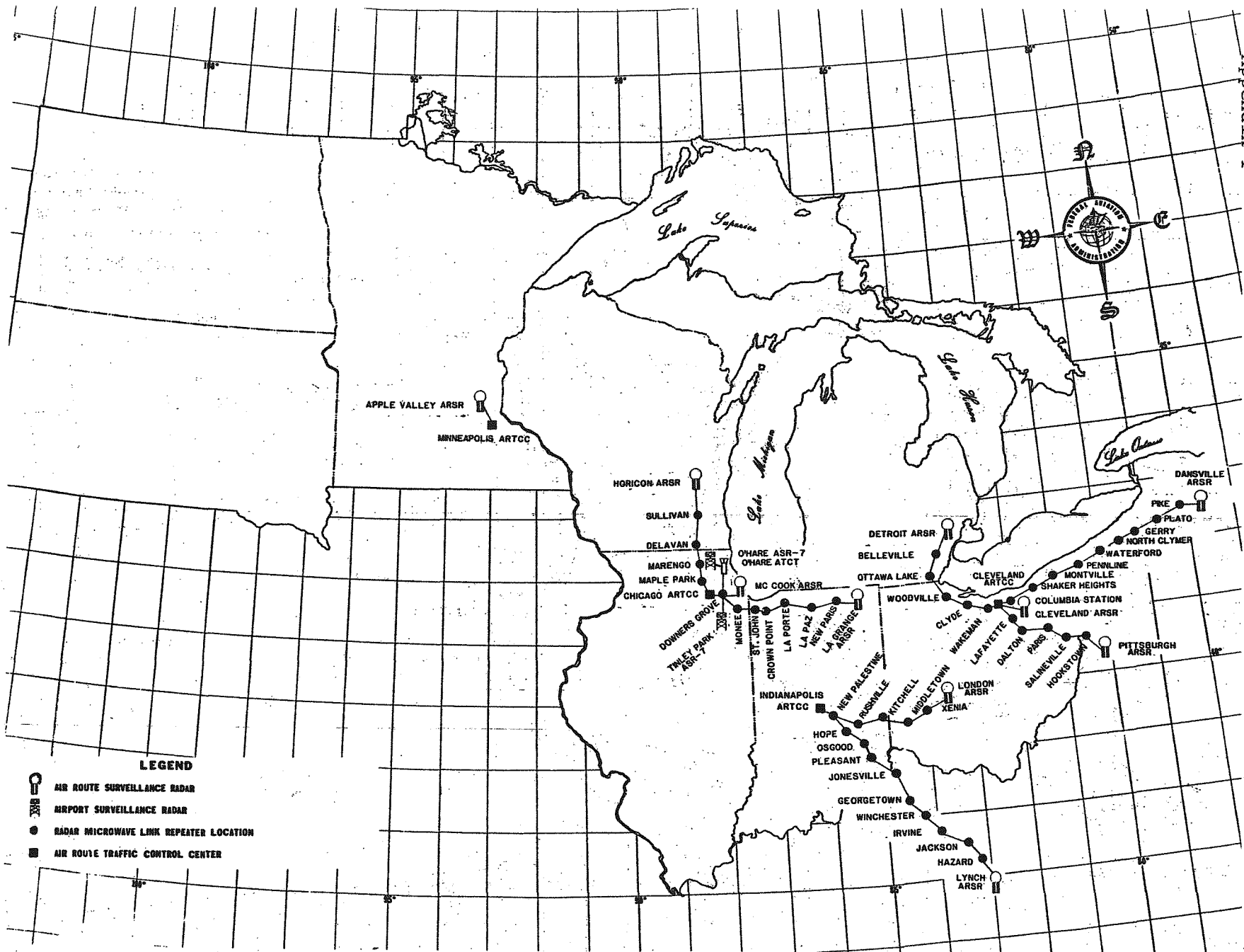
FIGURE 2. RML SYSTEMS
