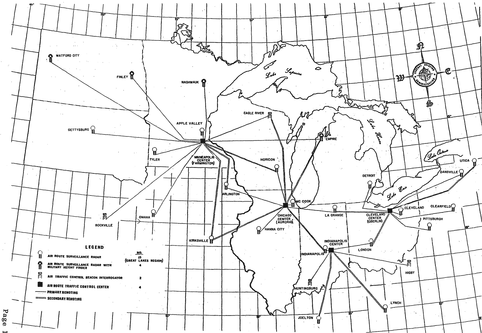
FIGURE 1. ARTCC AND ASSOCIATED LONG RANGE RADAR LOCATIONS
