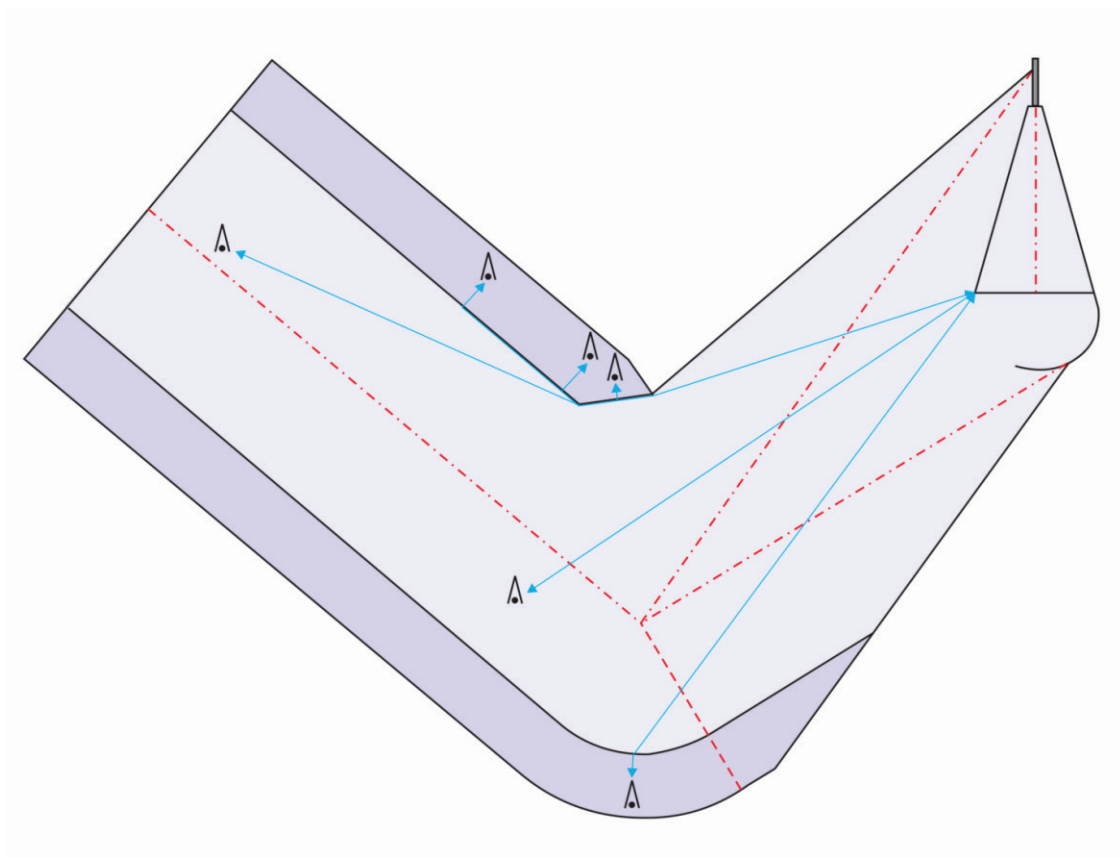
Figure 5-4-3. Obstacle Distance Measurements, Turn-at-Altitude, Multiple Legs
