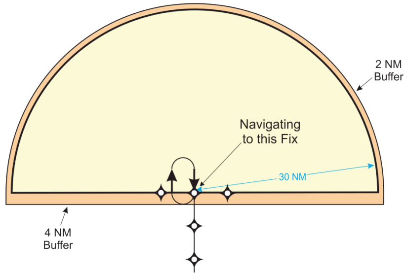
Figure 2-4-4. Straight-in Area
