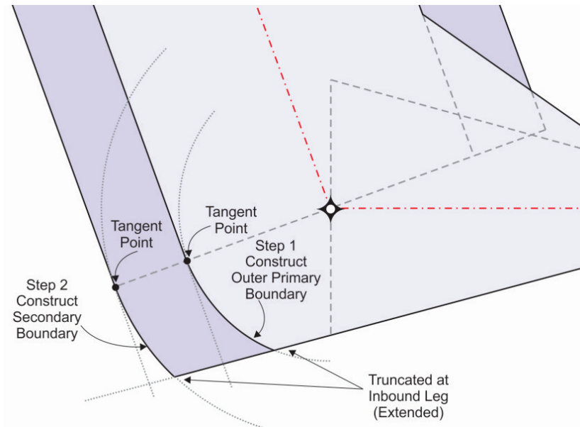
Figure 3-7-14. Late/Outside Turn, First Turn, Turn-at-Fix (FB)
