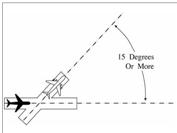
FIG 5-8-5 Intersecting Runway Departures
