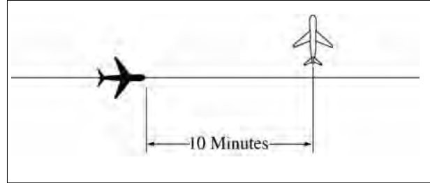
FIG 6-4-15 Climbing Through Another Aircraft's Altitude Separation
