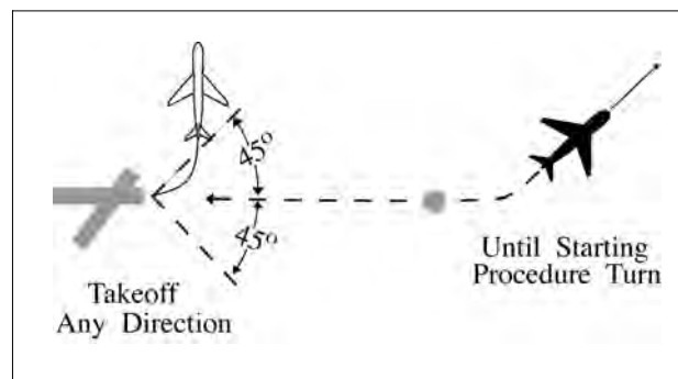
FIG 6-3-3 Separation Minima
