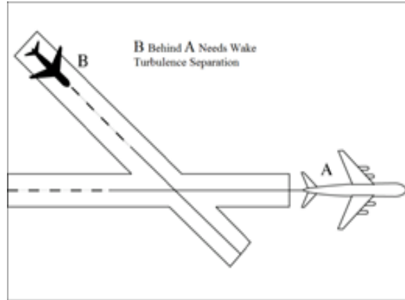
FIG 3-9-12 Departure Behind Arrival on Intersecting Runway
