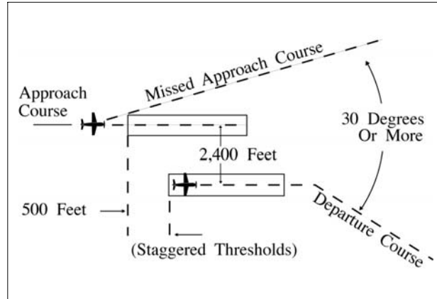
FIG 5-8-11 Parallel Thresholds are Staggered
