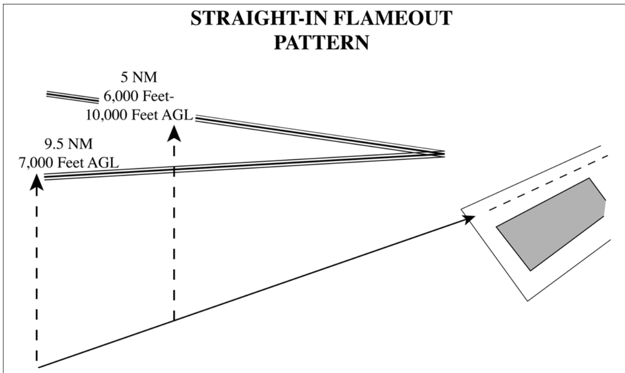
FIG 3-10-15 Simulated Flameout [2]
