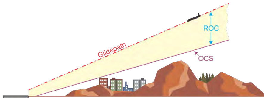
Figure 2-1-3. PA/APV Glidepath Descent
