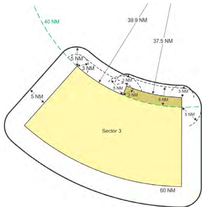
Figure 11-3-2. Buffer Area, Contiguous Sector crossing 40 NM. (Single Sensor, w/out reinforced MSSR)
