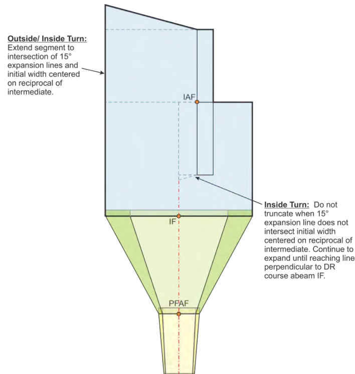
Figure 2-4-7. Example DR Segment
