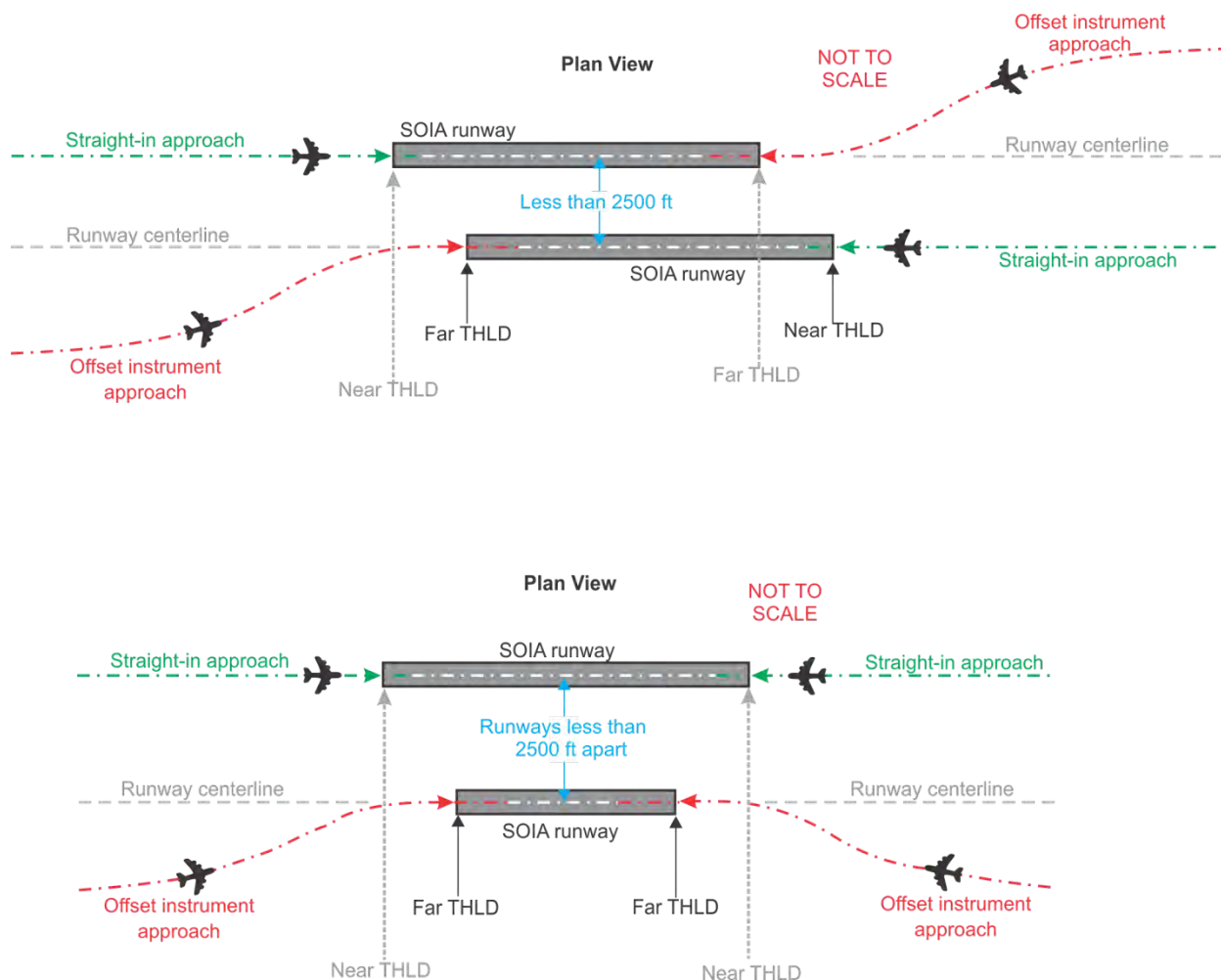
Figure E-5. Examples of SOIA Design with Staggered Thresholds
