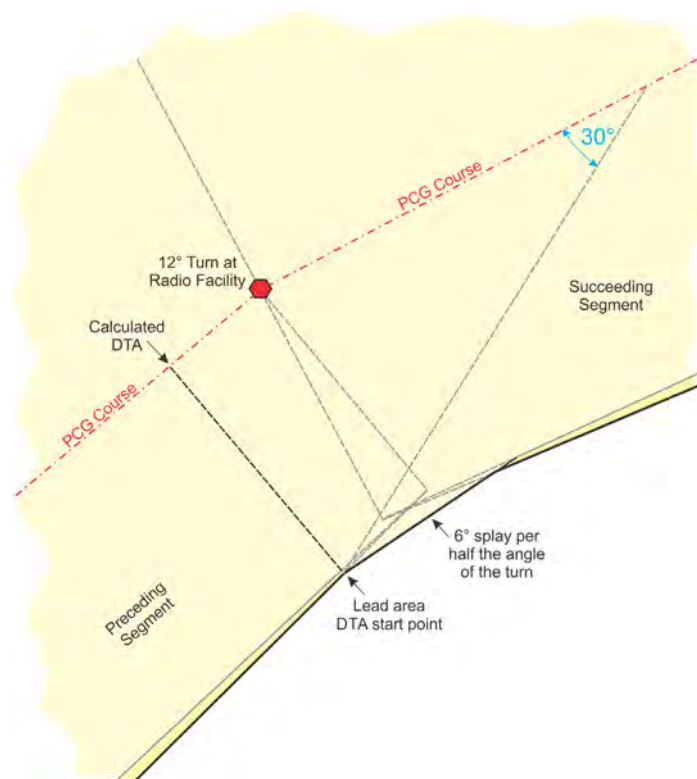
Figure 13-3-16. Inside Turn Area Construction, 12° Turn Over Radio Facility
