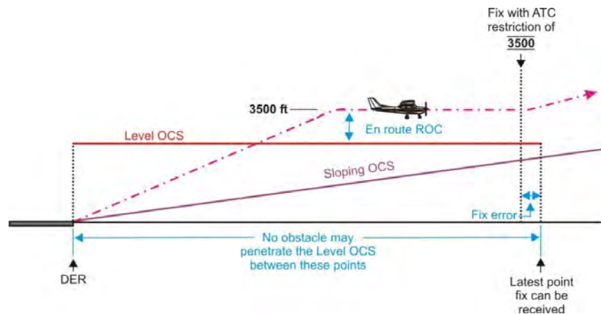
Figure 13-3-26. Continuation of Sloping OCS
