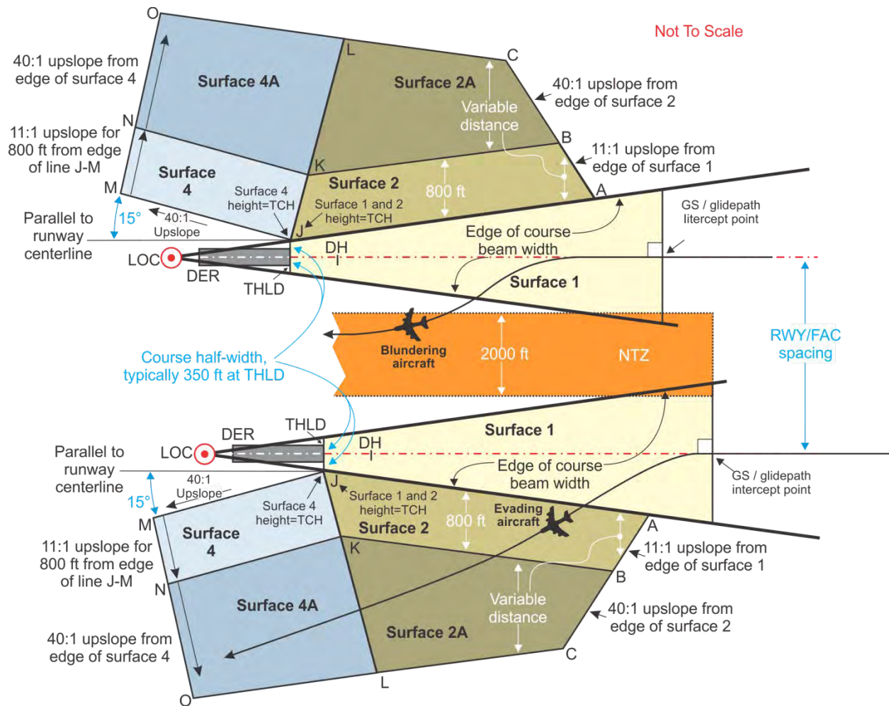
Figure E-11. Parallel Approach Obstacle Assessment Surface 4
