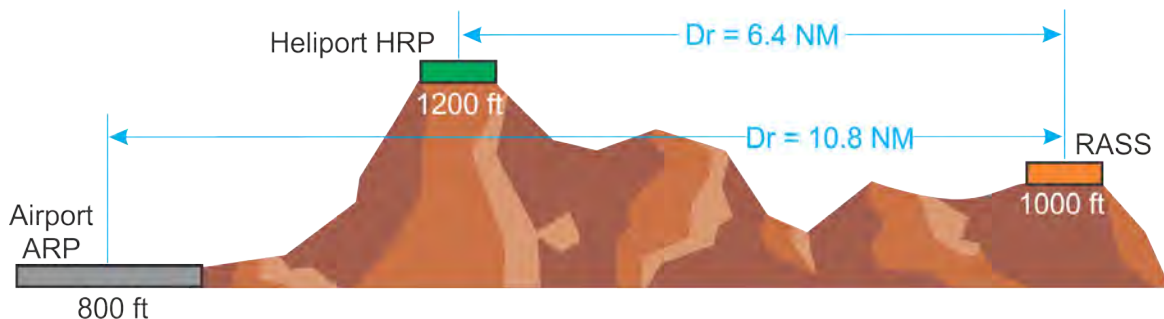
Figure 3-2-2. Basic RASS adjustment (no intervening terrain)
