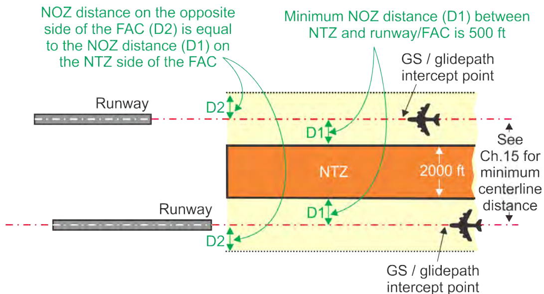
Figure E-7. Simultaneous Approach NTZ and NOZ
