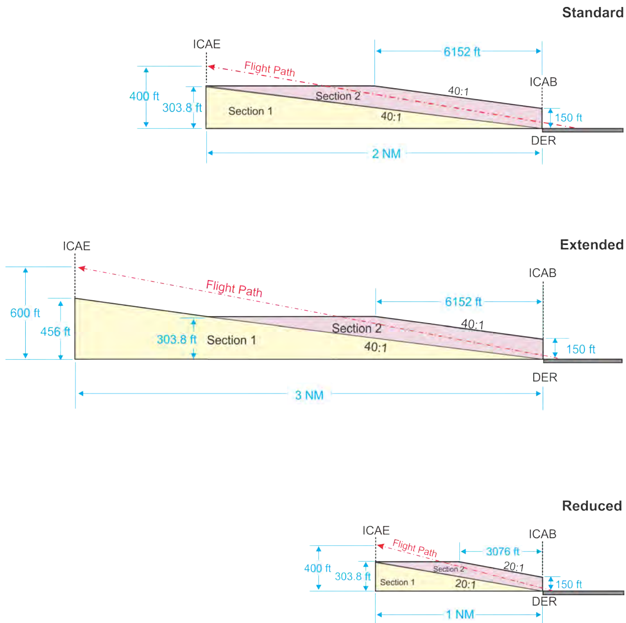
Figure 13-1-5. ICA OCS Profile: Various Lengths
