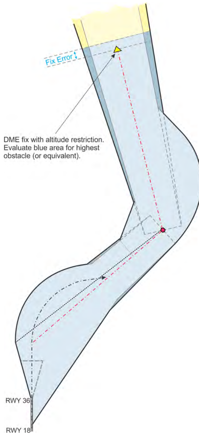
Figure 13-3-23. No Turn Required at Fix
