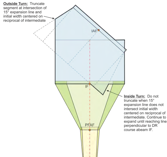
Figure 2-4-7. Example DR Segment
