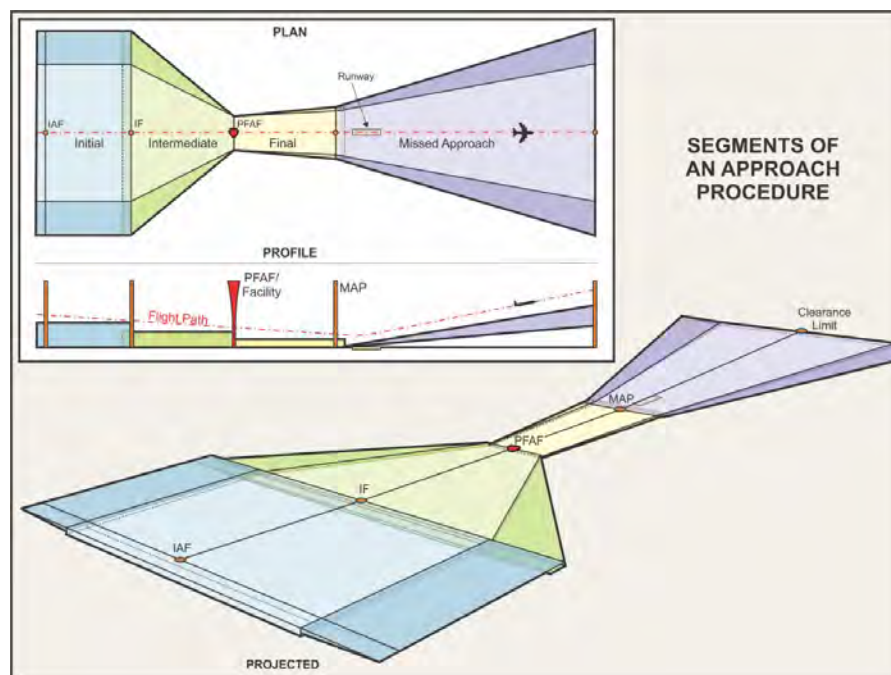
Figure 2-1-5. Segments of an Approach Procedure
