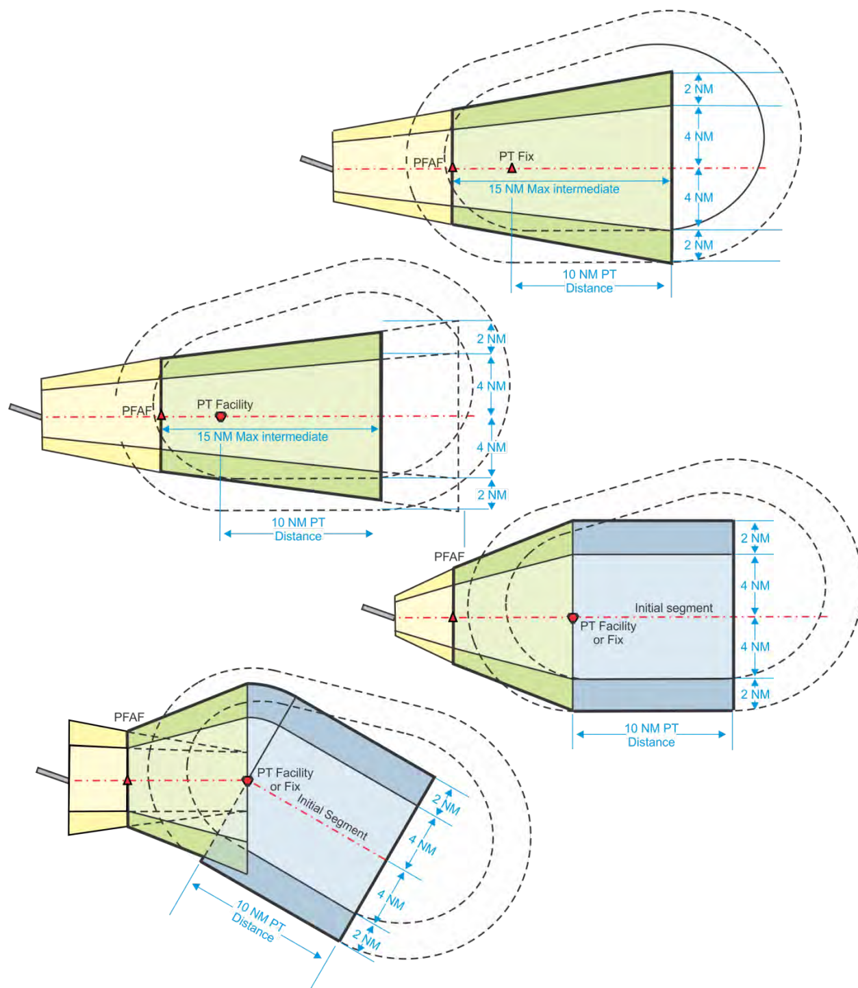
Figure 2-5-8. Use of PT Fix for IF
