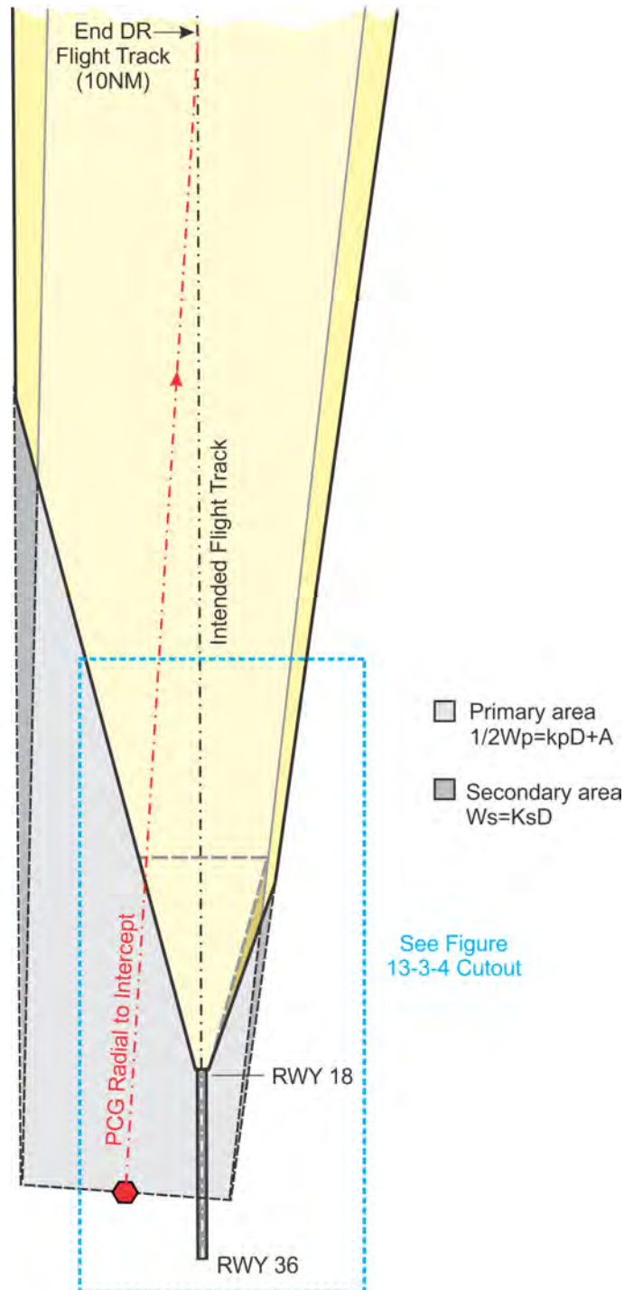
Figure 13-3-4. Facility Area and DR Area Relationship
