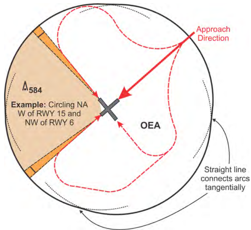
Figure 2-7-4. Complex Restricted Circling Area, Circling Aligned Approach (<180 Degrees)
