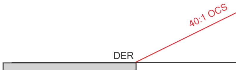
Figure 13-1-6. OCS Starting Elevation
