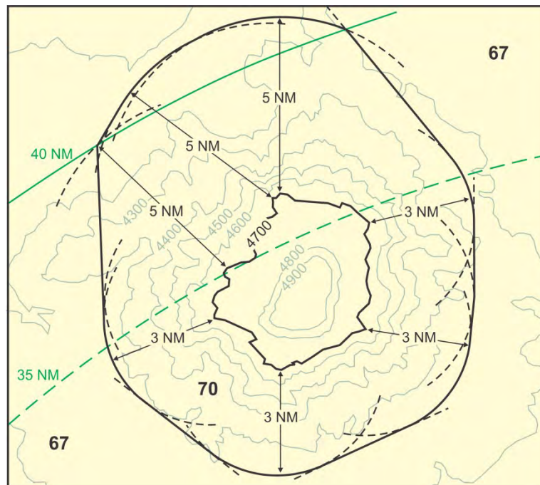
Figure 11-3-9. Isolation Area, Zone Feature, Example Construction > 35 NM from Radar (Single Sensor, w/out Reinforced MSSR)
