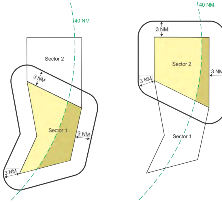
Figure 11-3-4. Fusion Adaptation Sector Buffer Areas (3-NM Separation Minima Chart)
