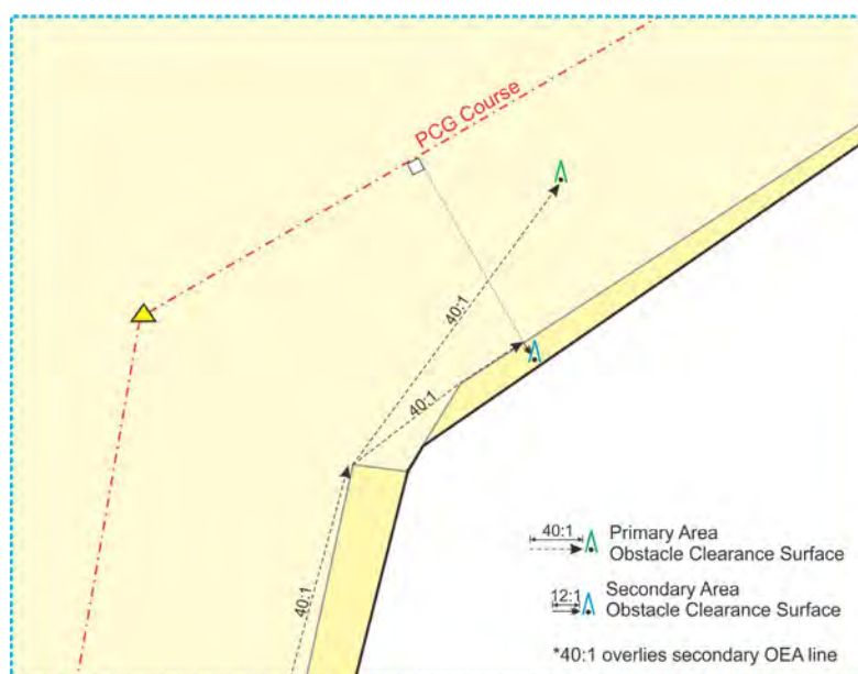
Figure 13-3-20. OEA Example 1, Cutout 2
