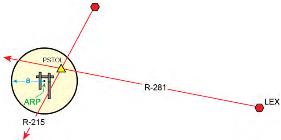
Figure 13-4-5. Offset VCOA Departure Route
