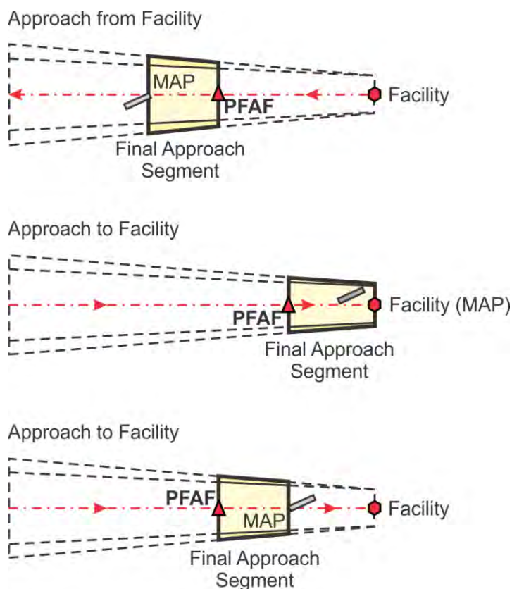
Figure 5-2-7. Typical Straight-in Final Approaches VOR with PFAF
