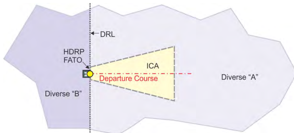
Figure 13-2-2. Heliport Diverse Departure Assessment Areas
