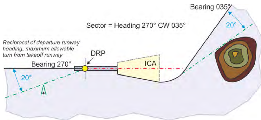
Figure 13-2-11. Maximum Heading Limitation
