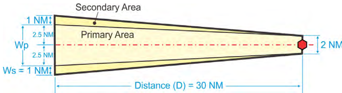
Figure 5-2-6. Final Approach Trapezoid. VOR with PFAF
