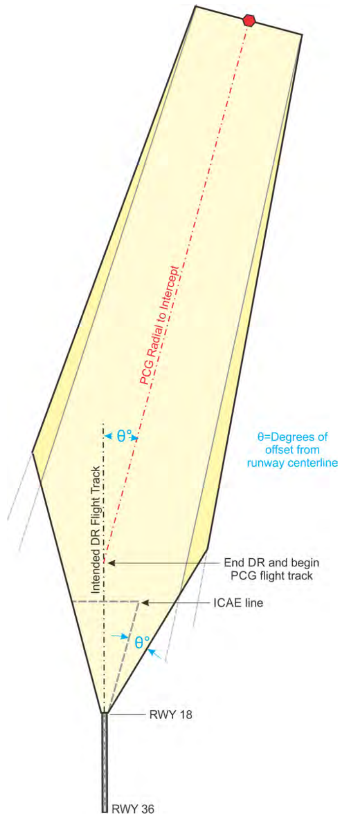
Figure 13-3-6. Facility Area Relationship, Off Airport NAVAID
