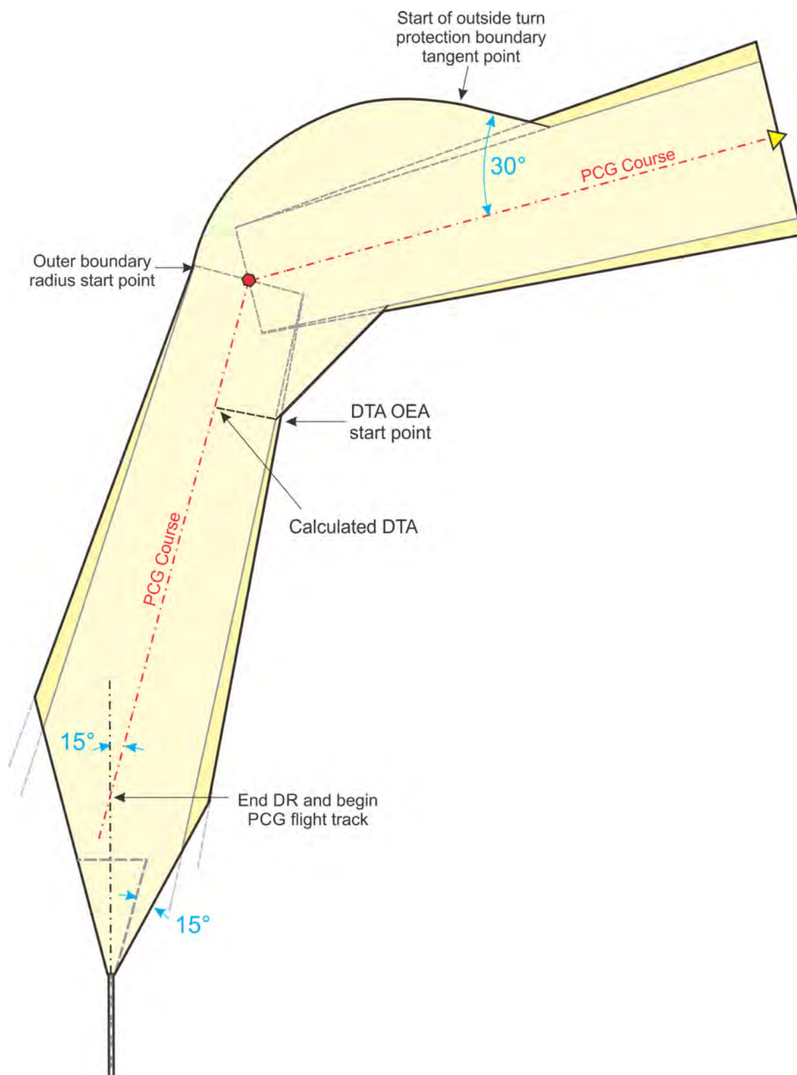
Figure 13-3-19. Turn at NAVAID to Fix
