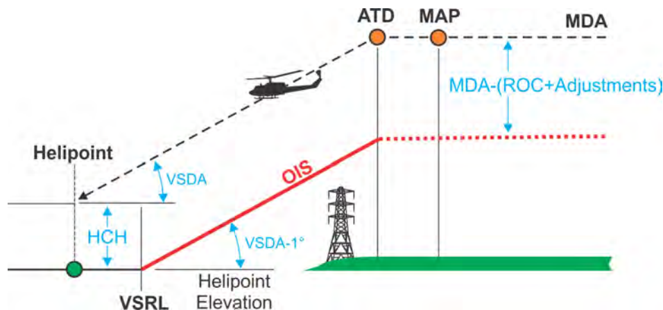
Figure 12-2-3. VSDA and Associated OIS
