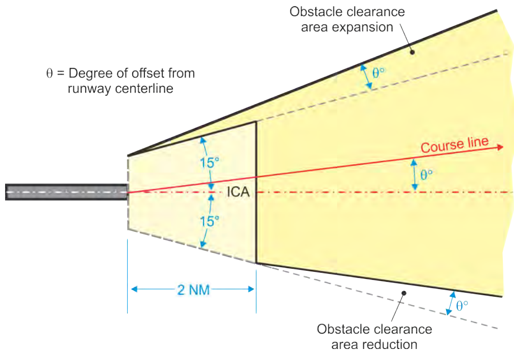
Figure 13-3-1. Turn \leq 15 degrees at DER
