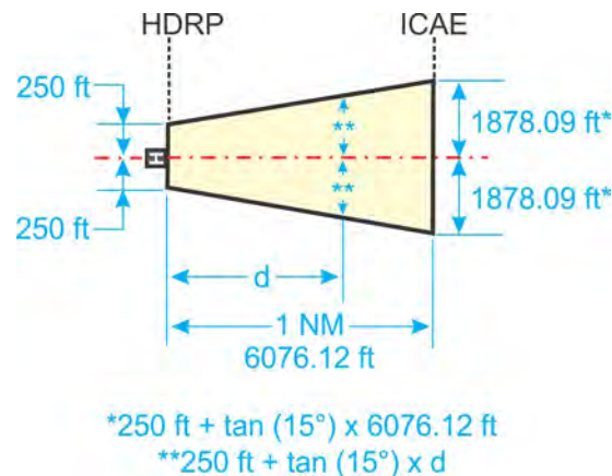
Figure 13-1-2. Legacy ICA: Helicopters
