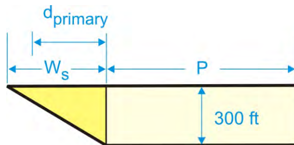
Figure 4-2-4. Final Approach Area ROC
