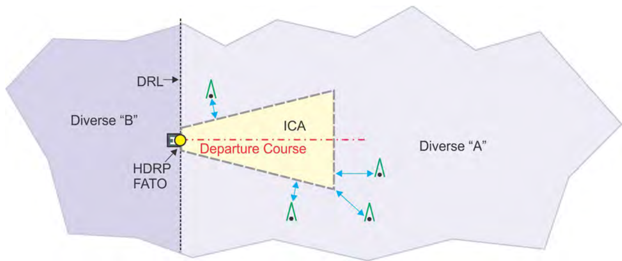
Figure 13-2-4. Heliport Diverse “A” Area Evaluation
