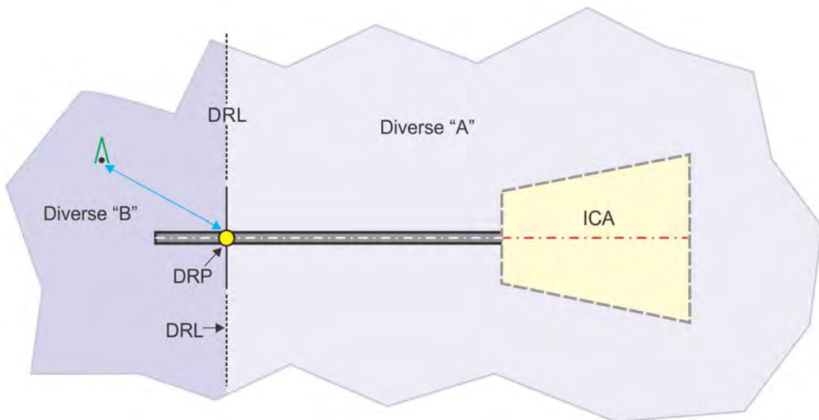
Figure 13-2-5. Diverse "B" Area
