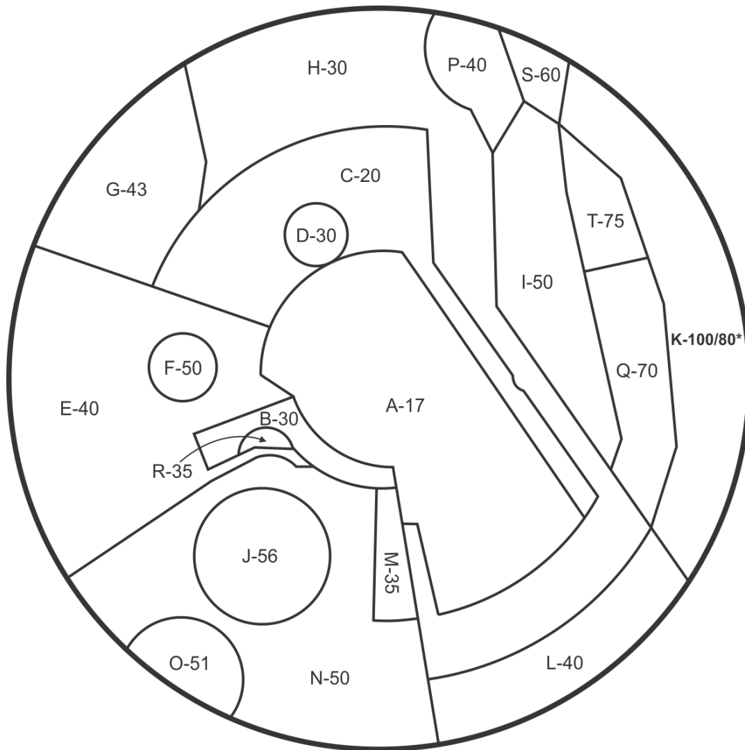
Figure 11-3-10. MVAC for Single Sensor Configuration or FUSION Adaptation
