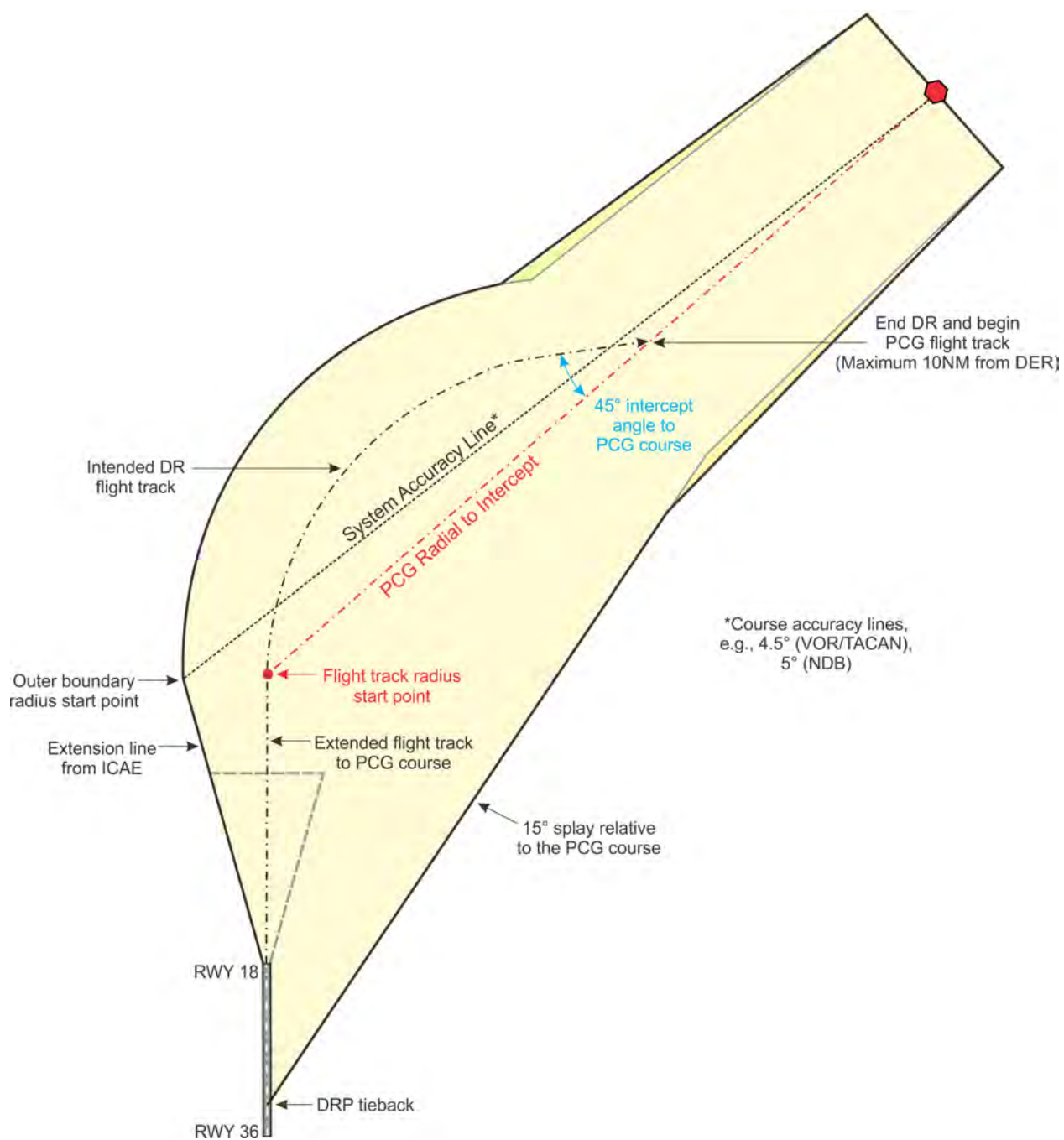
Figure 13-3-10. Turn to Intercept Radial with Arc Extension (Off Airport NAVAID)
