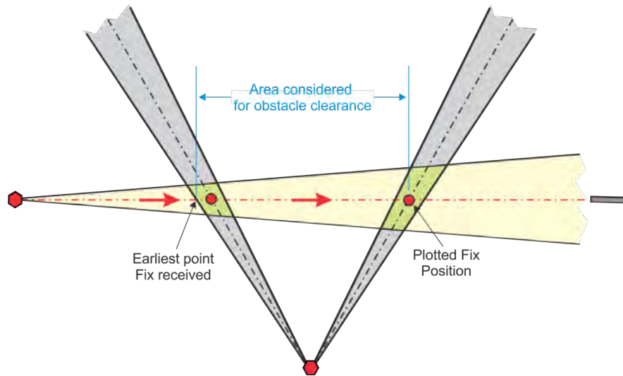
Figure 2-9-7. Obstacle Clearance Area Between Fixes
