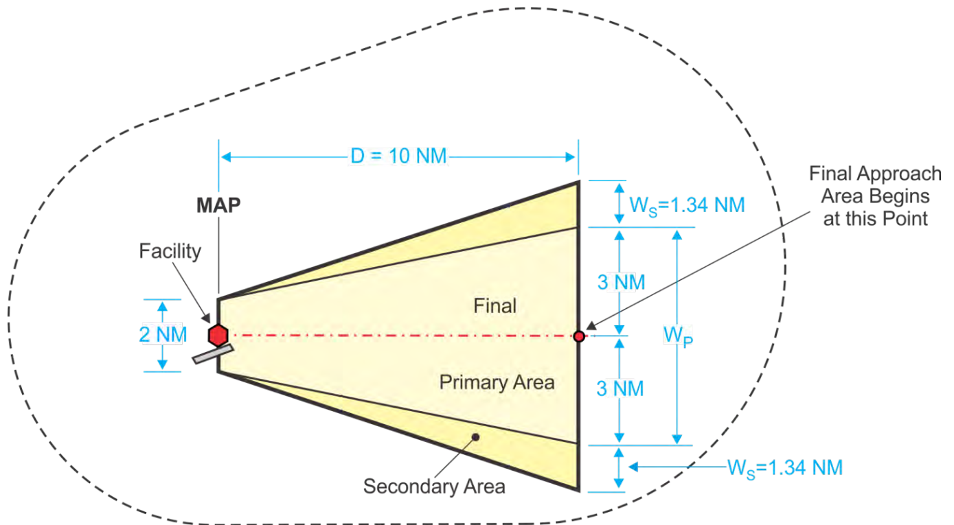
Formula 4-2-1. Final Approach Primary Area Half Width
