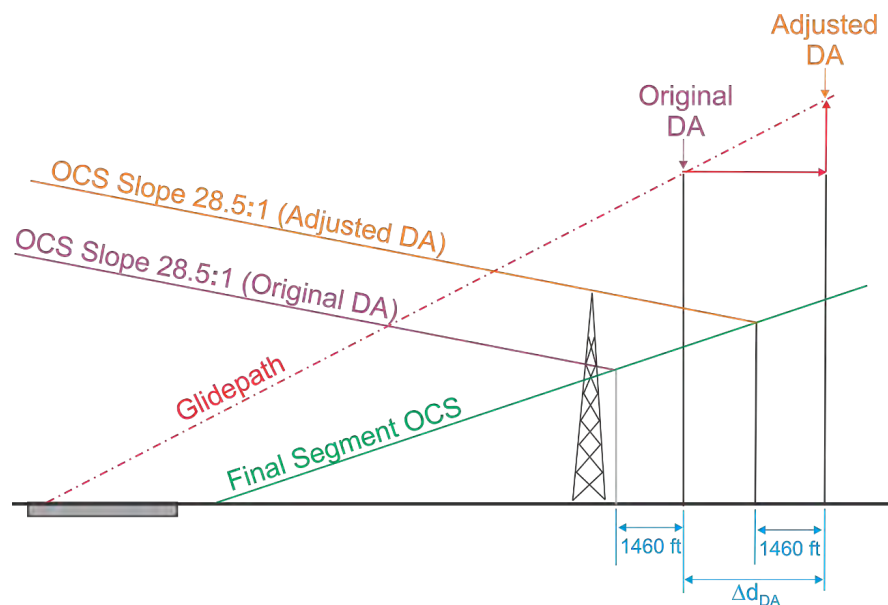
Figure 10-3-2. Penetration of Section 1b OCS
