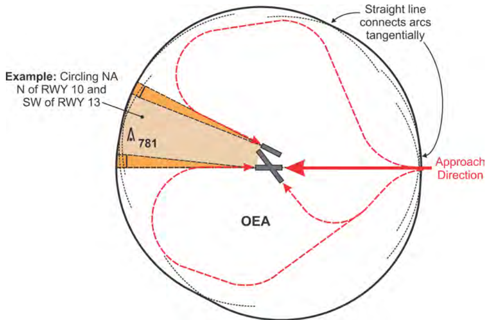
Figure 2-7-5. Complex Restricted Circling Area, Straight-in Aligned Approach (<180 Degrees, Intersecting Runways)
