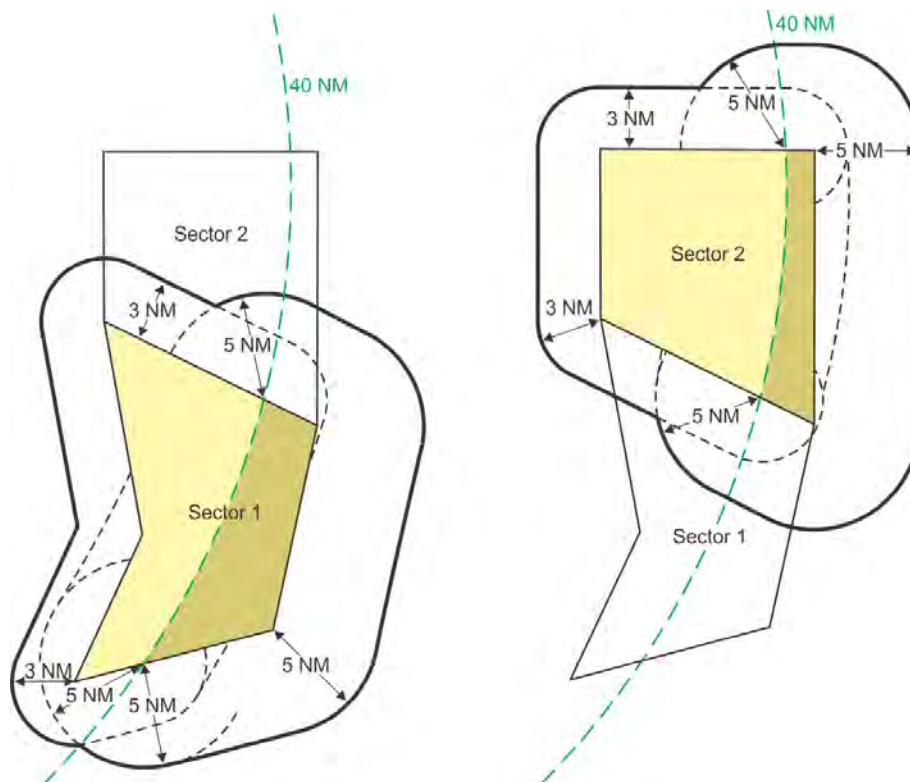
Figure 11-3-1. Sector Buffer Areas (Single Sensor, w/out reinforced MSSR)
