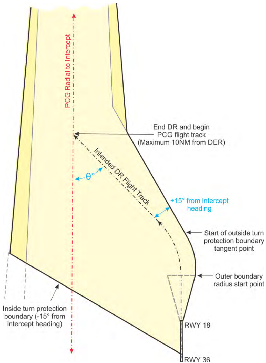
Figure 13-3-7. Turn to Intercept Radial (Off Airport NAVAID)
