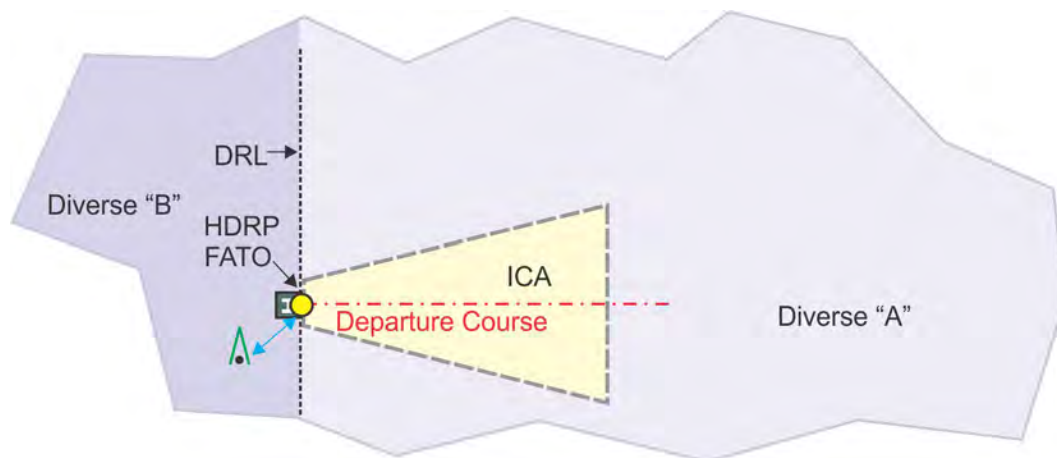
Figure 13-2-6. Heliport Diverse "B" Area
