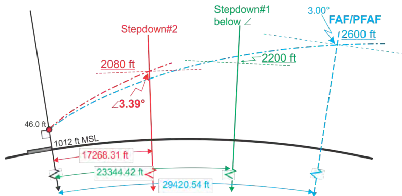
Figure 2-6-3. VDA with Stepdown Fixes
