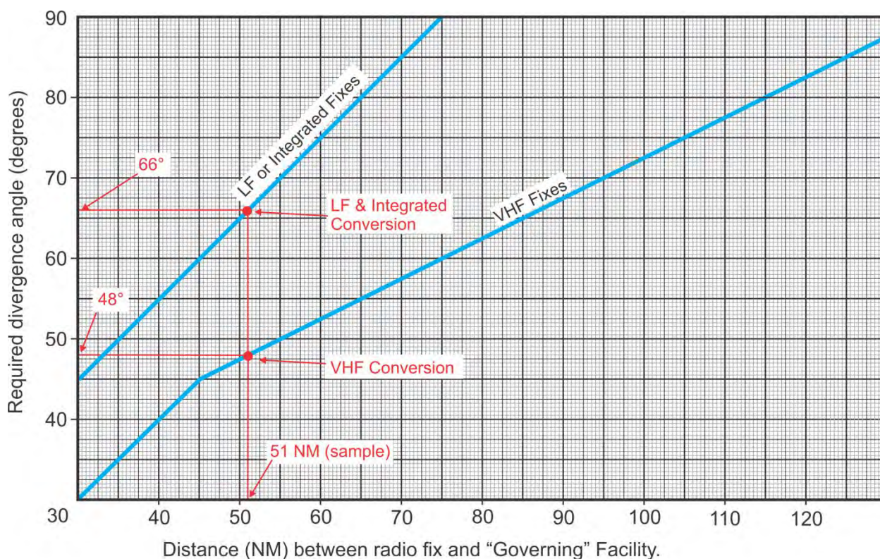
Figure 14-6-1. Minimum Divergence Angle for Radio Fix
