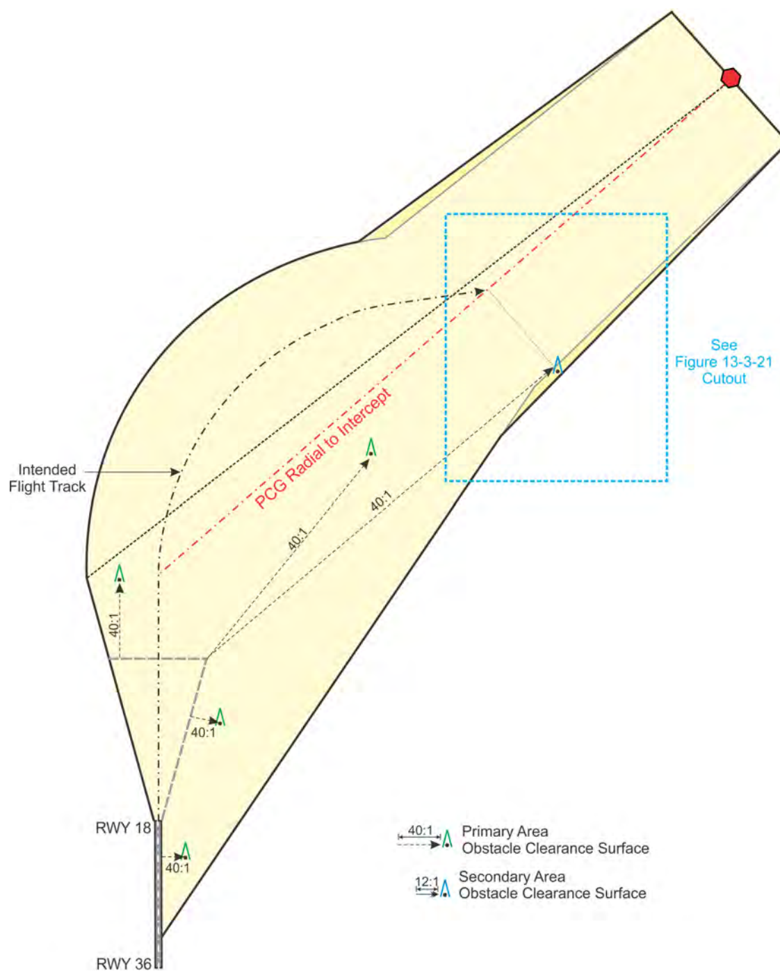
Figure 13-3-21. OCS Evaluation Along Departure Route (OEA Example 2)
