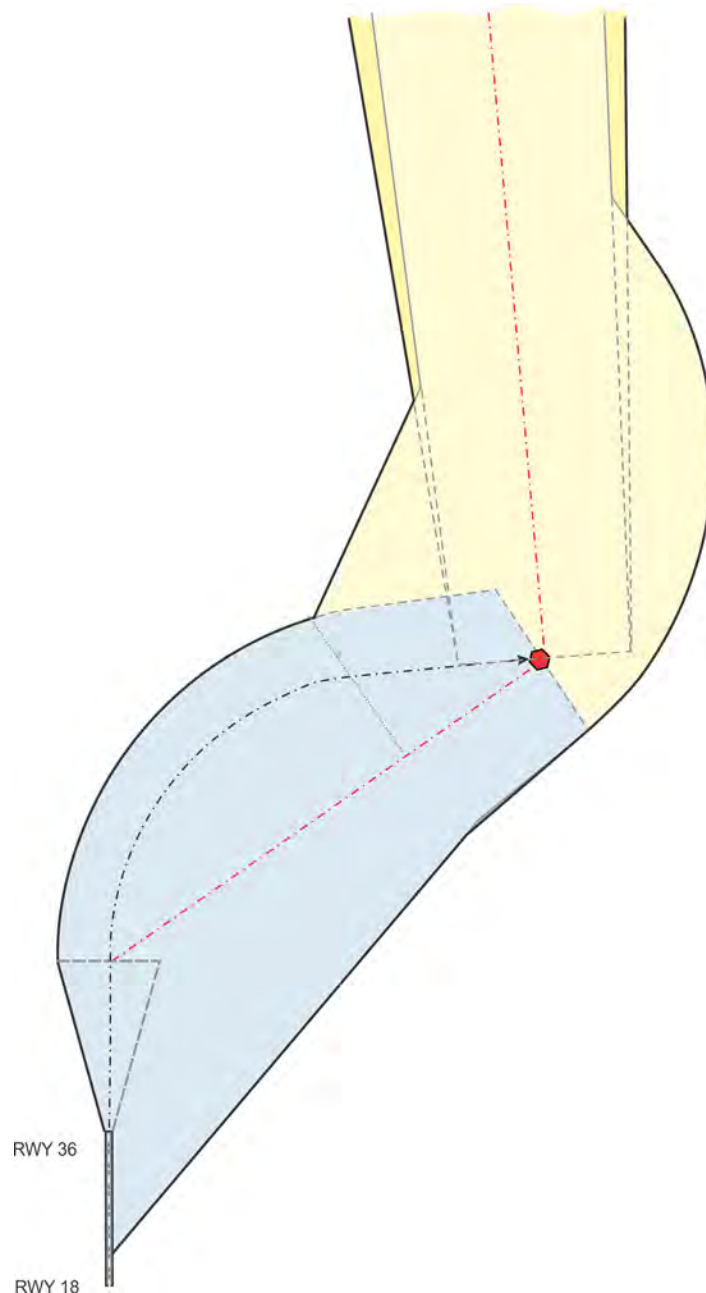
Figure 13-3-24. Turn Required at Fix
