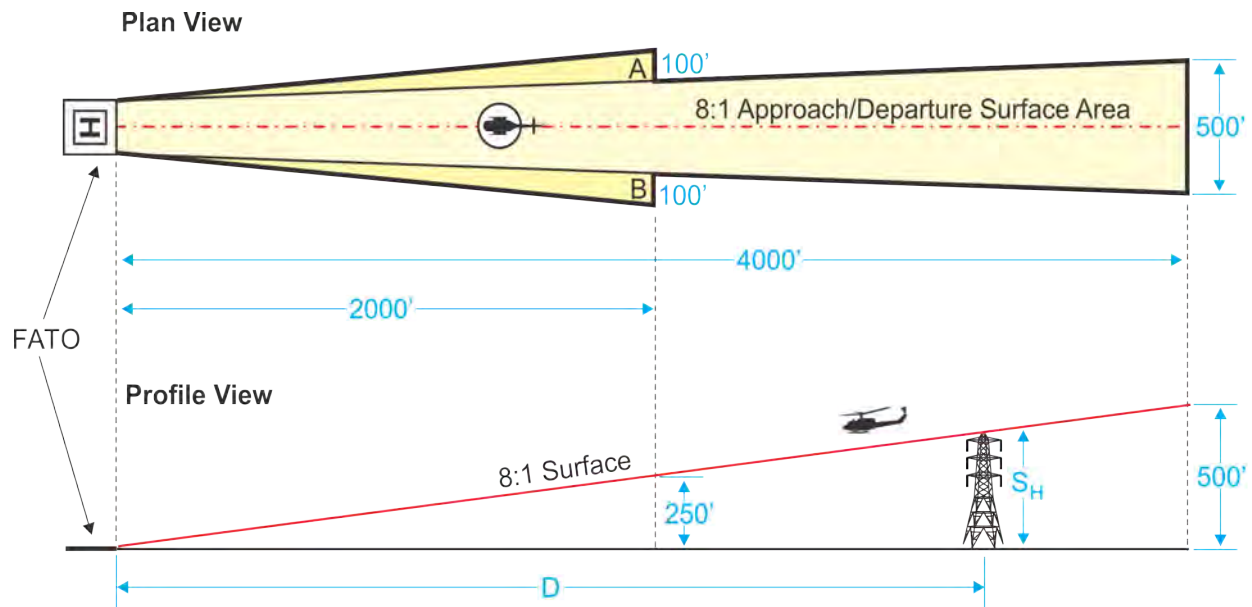
Formula G-1. 8:1 OCS Height ( S_H )
