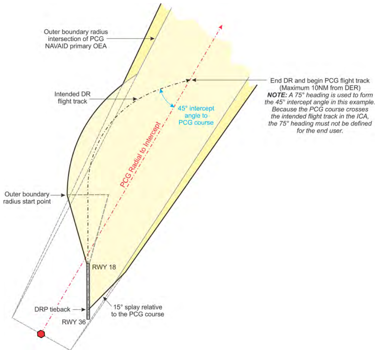
Figure 13-3-9. Turn to Intercept Radial, Example 2 (On Airport NAVAID)
