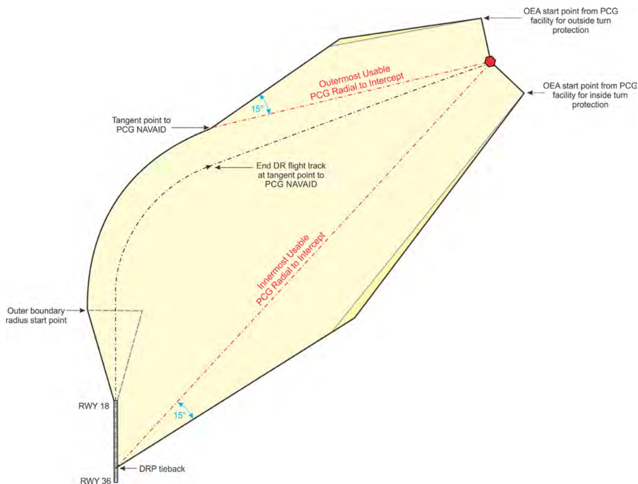
Figure 13-3-12. Direct to Facility, Turn Greater Than 15 Degrees but Less Than or Equal to 90 Degrees
