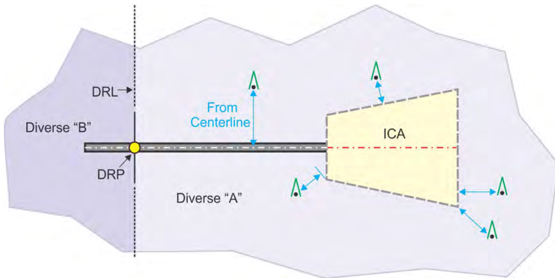
Figure 13-2-3. Diverse “A” Area Evaluation
