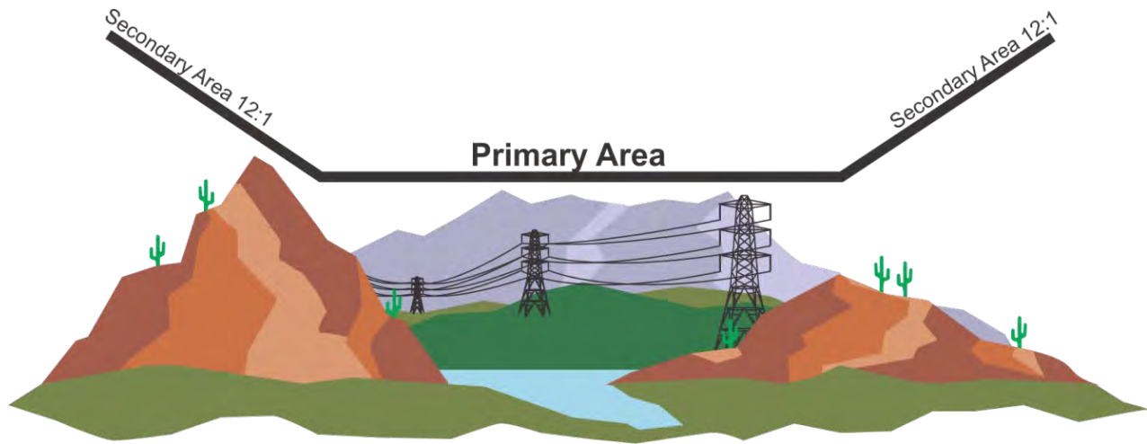
Figure 2-8-3. Missed Approach Cross Section
