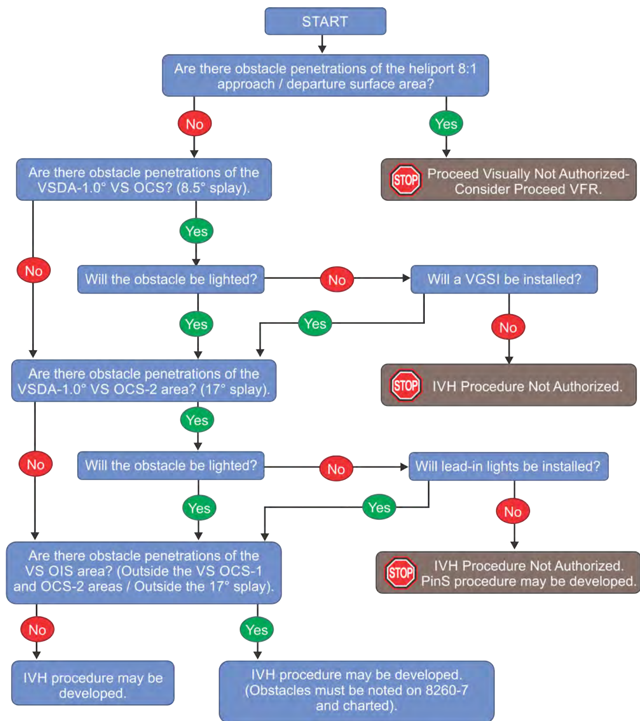
Figure G-3. IVH Procedure Decision Process
