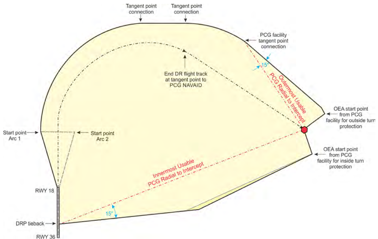
Figure 13-3-13. Direct to Facility, Turn Greater Than 90 Degrees but Less Than or Equal to 180 Degrees
