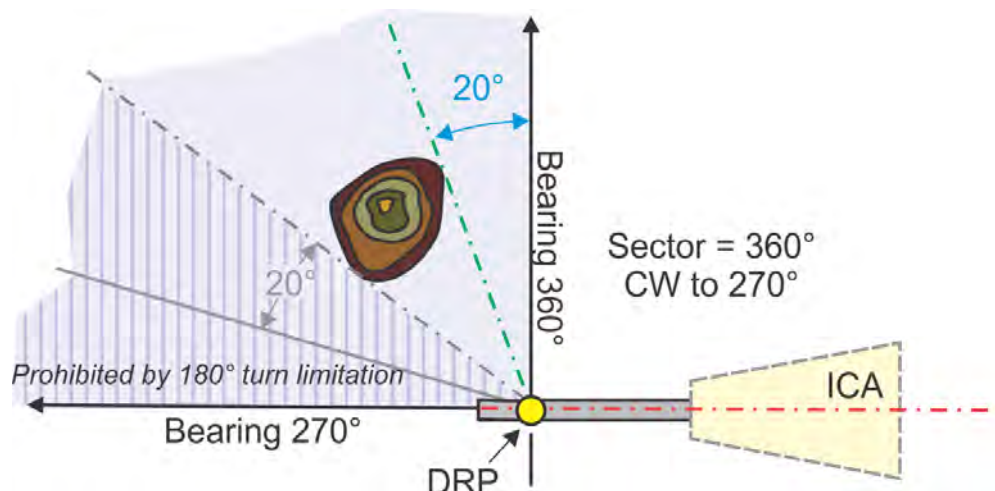
Figure 13-2-11. Maximum Heading Limitation
