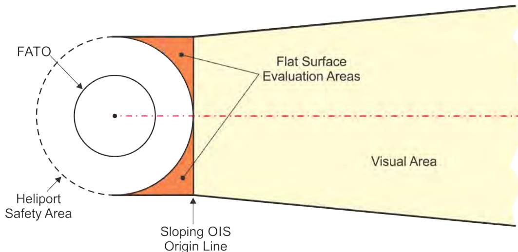
Figure 3-3-4. Helicopter Visual Area with Circular FATO
