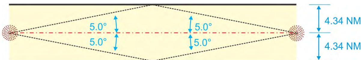
Figure 14-5-2. LF Segment Secondary Obstacle Clearance Area
