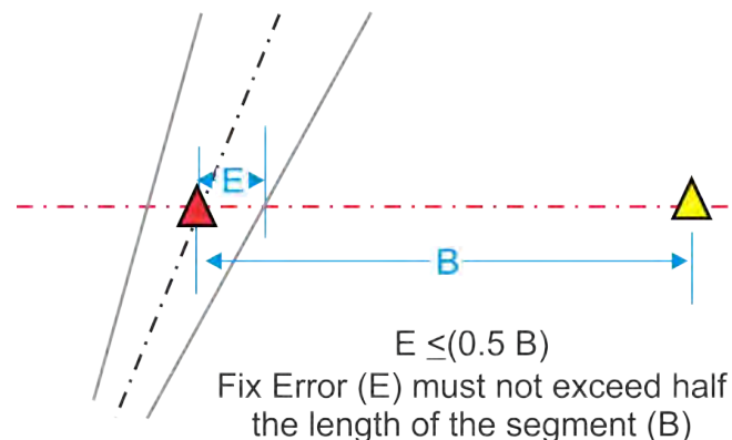
Figure 2-9-3. Intermediate, Initial, or Feeder Approach Fix Errors
