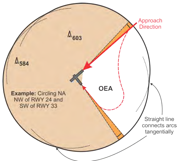
Figure 2-7-7. Complex Restricted Circling Area, Expanded Restricted Area, Straight-in Aligned Approach
