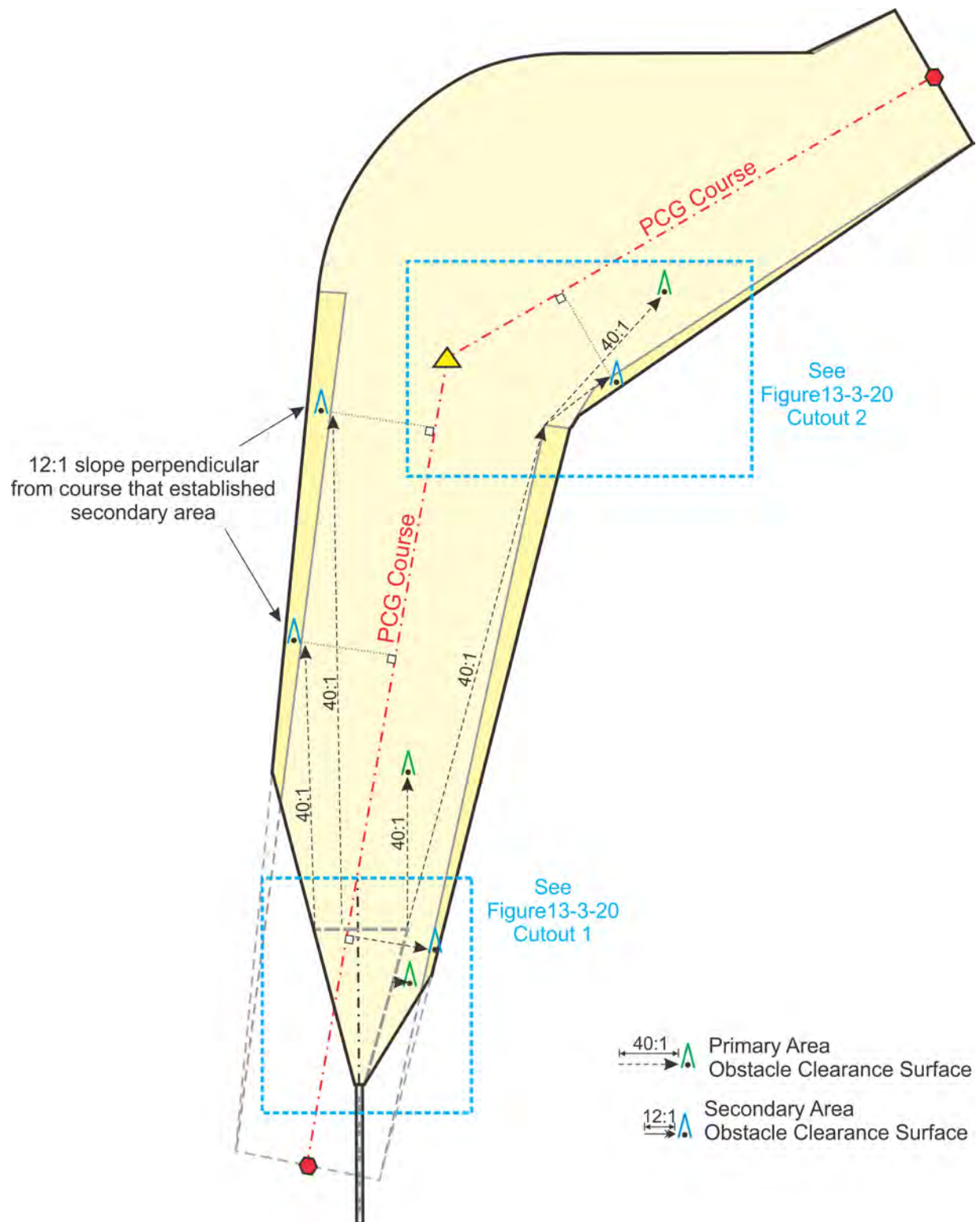
Figure 13-3-20. OCS Evaluation Along Departure Route (OEA Example 1)
