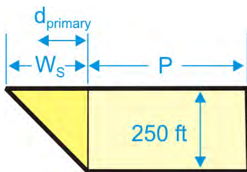
Figure 5-2-8. Final Approach Area ROC
