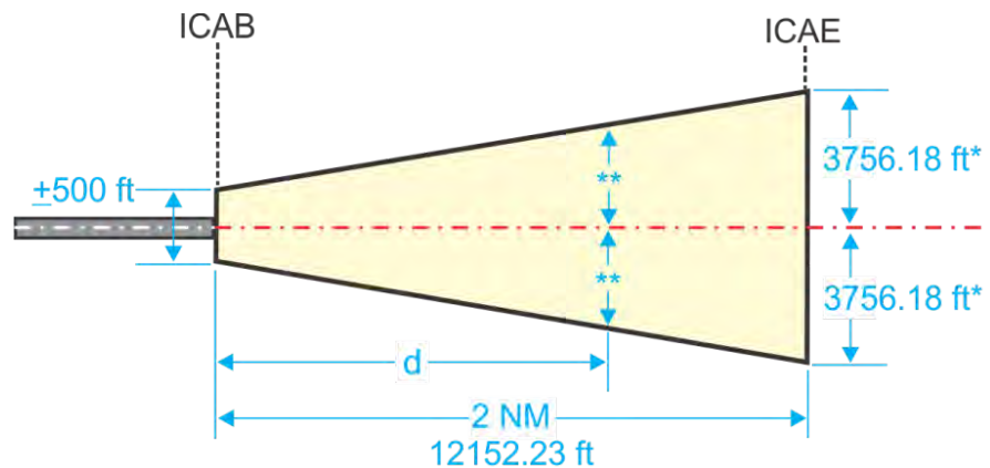
Figure 13-1-3. Initial Climb Area: Standard Length
