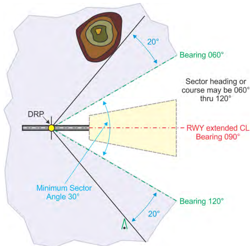
Figure 13-2-7. Minimum Sector Area
