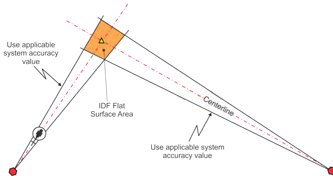
Figure 13-6-1. IDF Flat Surface
