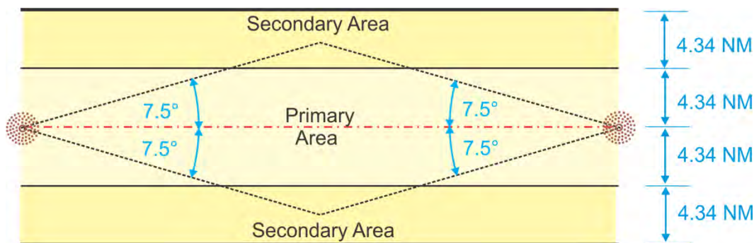
Figure 14-5-2. LF Segment Secondary Obstacle Clearance Area
