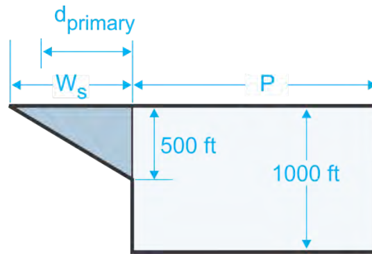
Figure 2-4-2. Straight/Arc Initial Segment Minimum ROC
