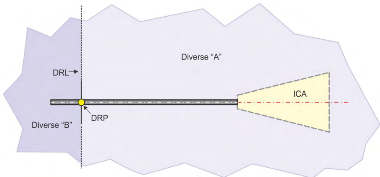
Figure 13-2-1. Diverse Departure Assessment Areas
