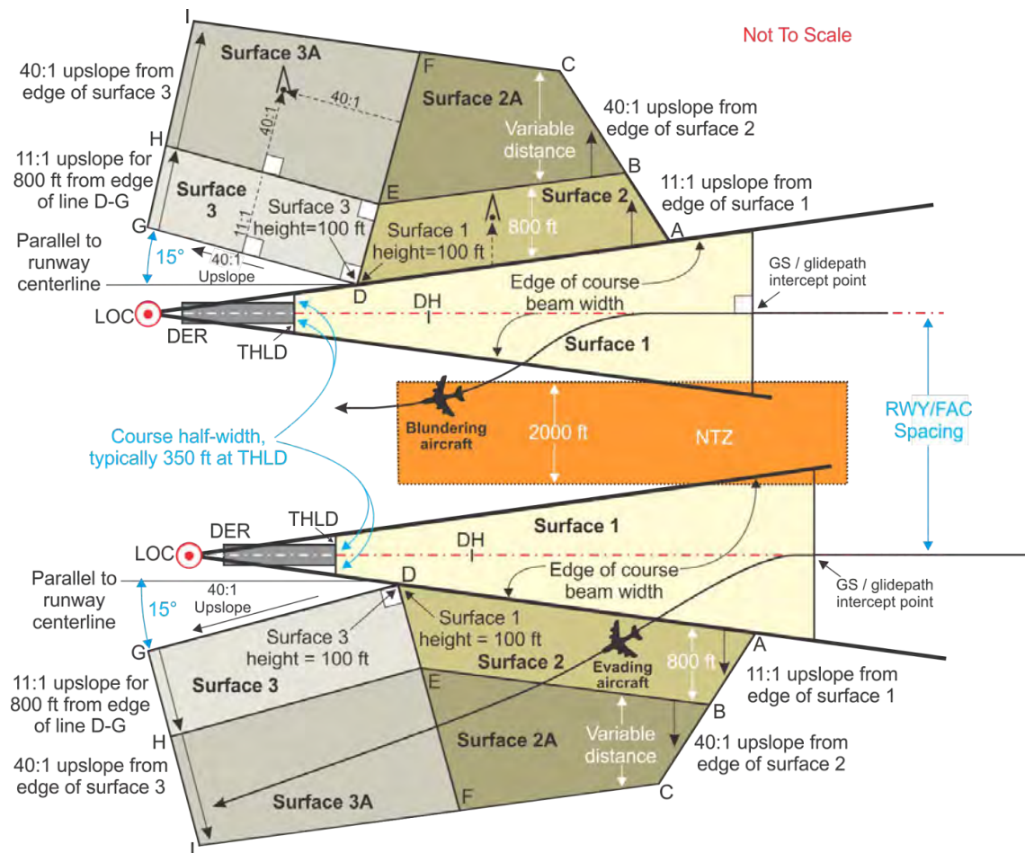
Figure E-10. Parallel Approach Obstacle Assessment Surface
