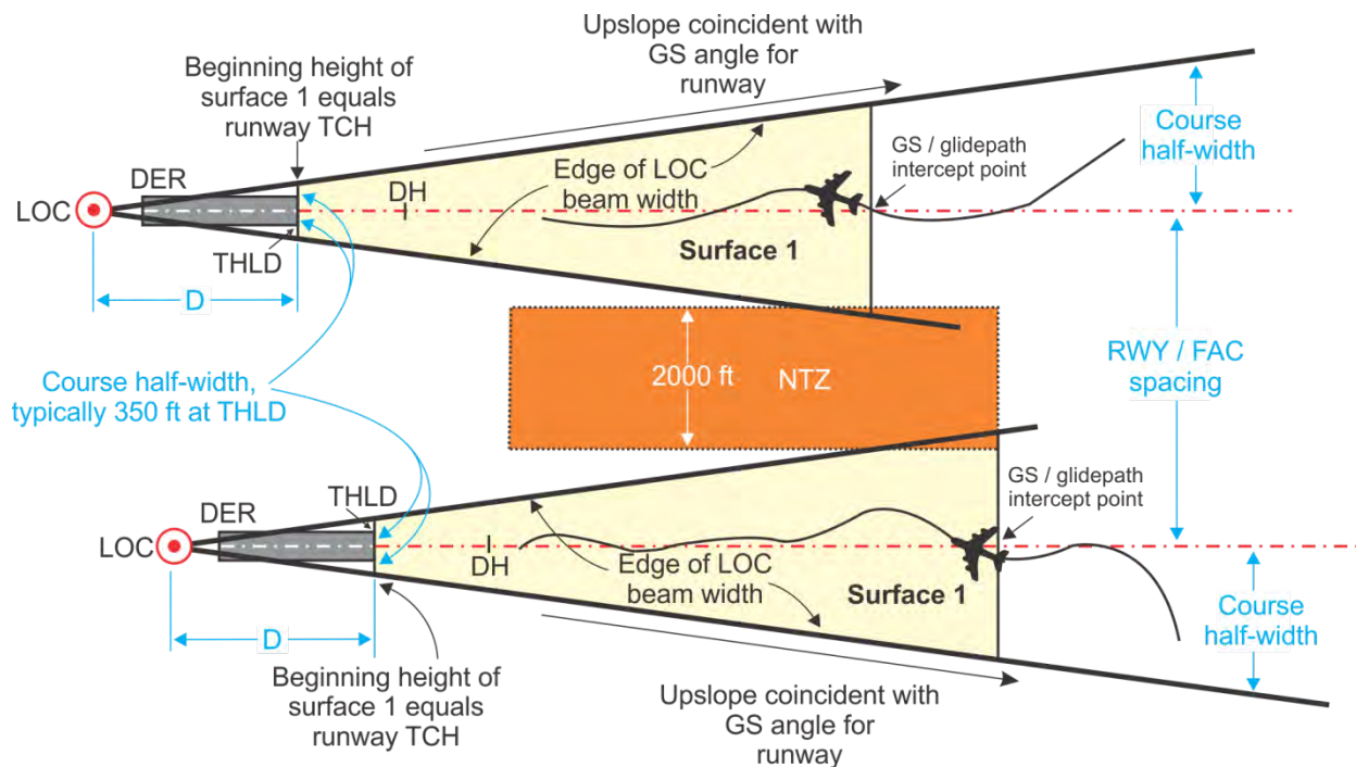
Figure E-8. Final Approach Descent Surface 1
