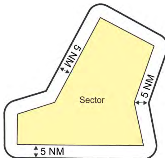
Figure 11-3-5. Fusion Adaptation Sector Buffer Areas (5-NM Separation Minima Chart)
