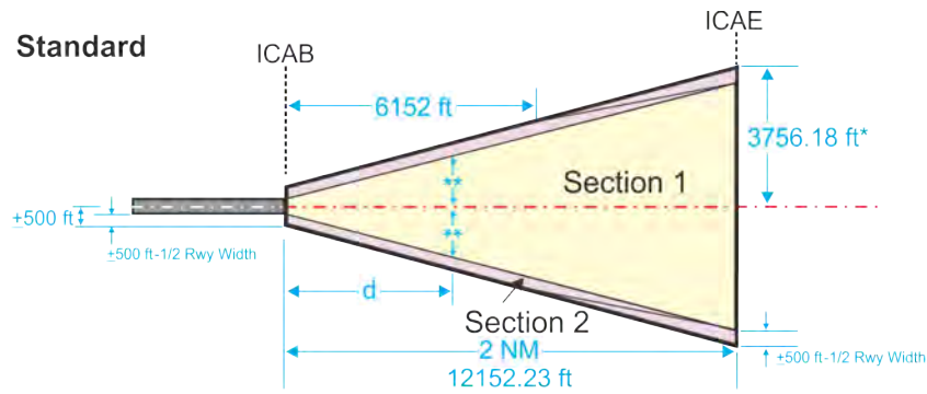
Figure 13-1-1. Initial Climb Area: Various Length
