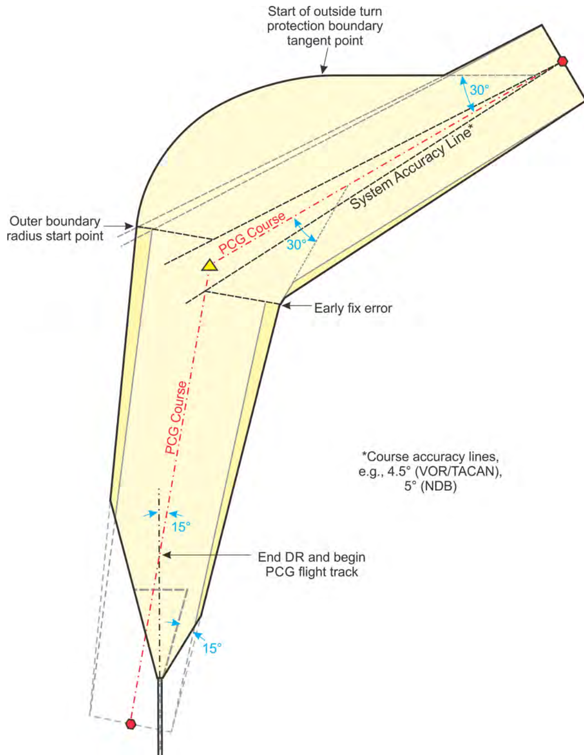
Figure 13-3-18. Turn at Fix to NAVAID
