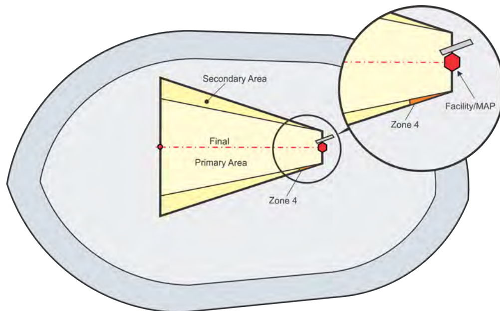
Figure 2-8-13. Climb-in Hold at MAP
