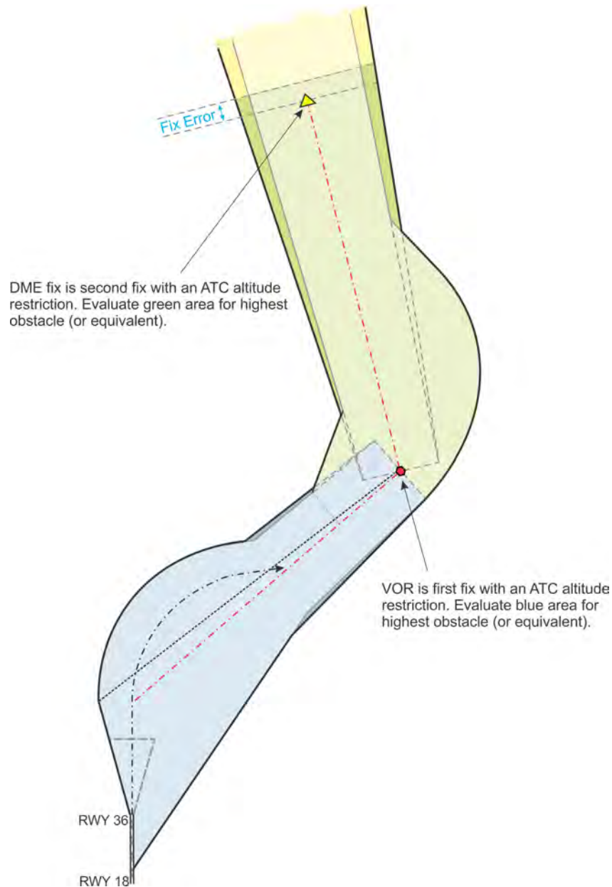
Figure 13-3-25. Multiple Altitude Restrictions
