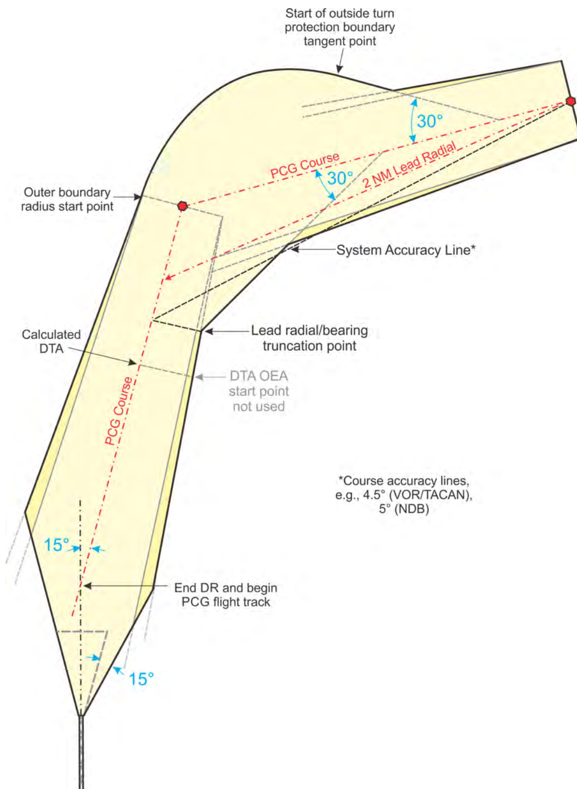
Figure 13-3-17. Turn at NAVAID to NAVAID
