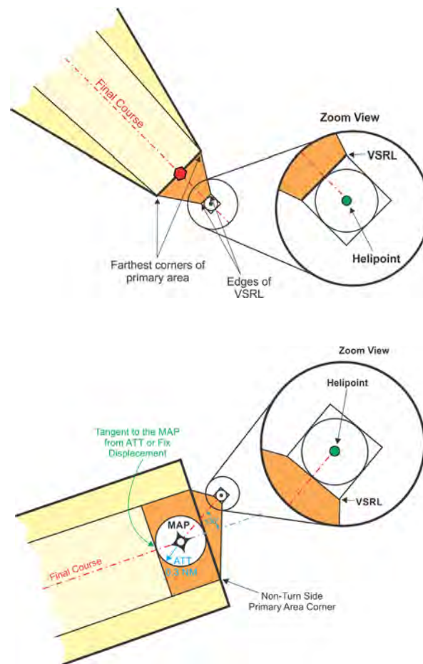
Figure 12-2-2. Visual Segment Area
