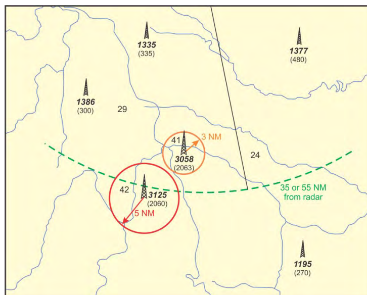
Figure 11-3-6. Isolation Area, Point Feature
