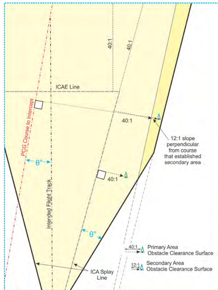
Figure 13-3-20. OEA Example 1, Cutout 2
