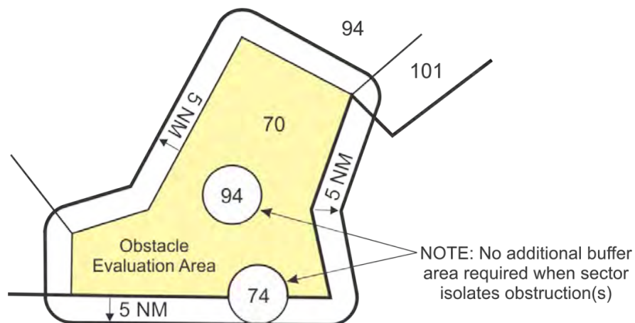
Figure 11-3-3. Multi-Sensor Buffer Areas
