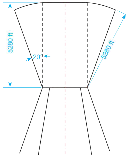
Figure 12-2-1. VFR Transition Area
