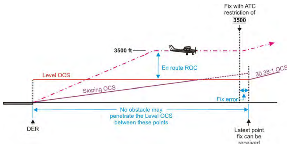
Figure 13-3-27. Sloping OCS Applied from Level OCS
