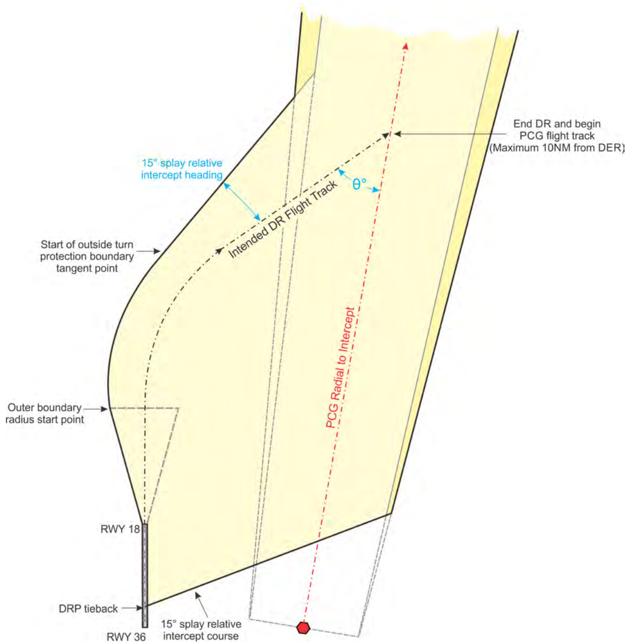
Figure 13-3-8. Turn to Intercept Radial, Example 1 (On Airport NAVAID)
