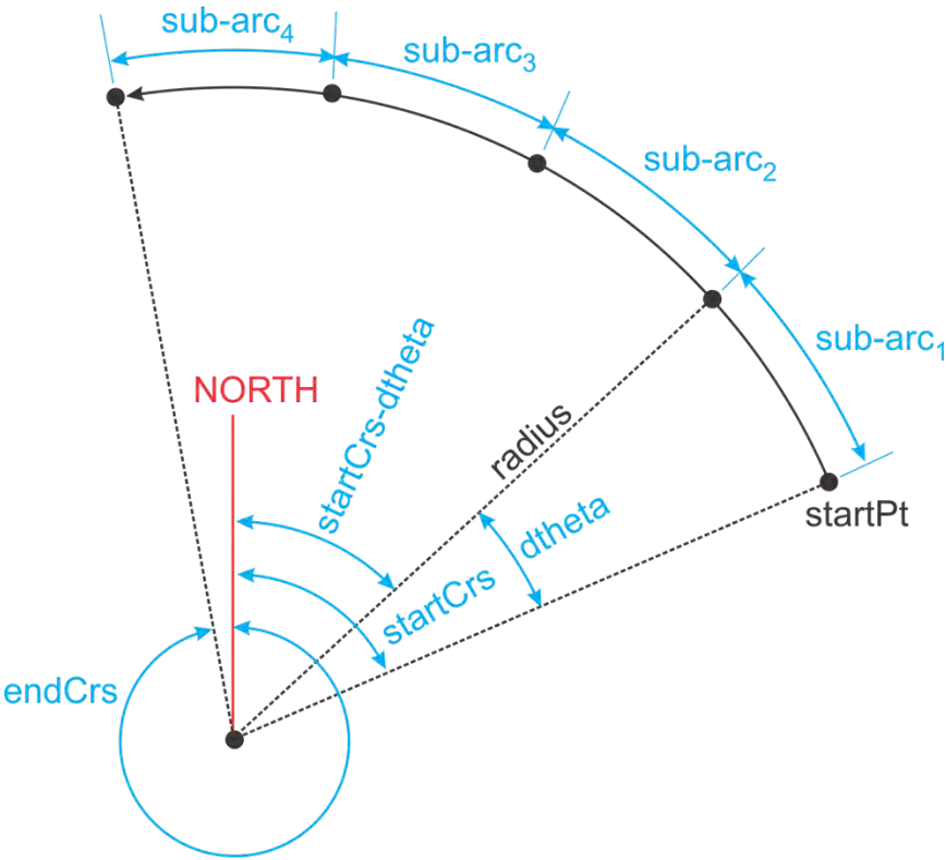
Figure F-12. Calculating the Sub-Arc Length
