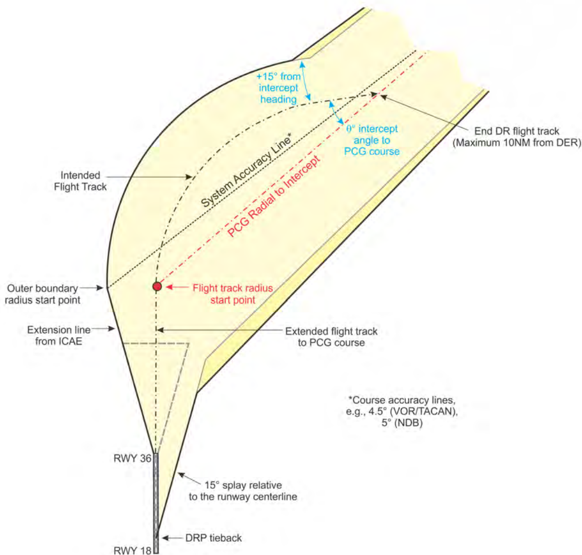
Figure 13-3-11. Turning at a Specified Radial/Bearing Prior to PCG Intercept
