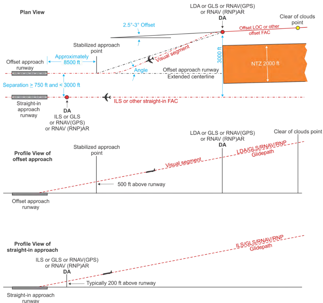
Figure E-4. Depiction of the SOIA Concept
