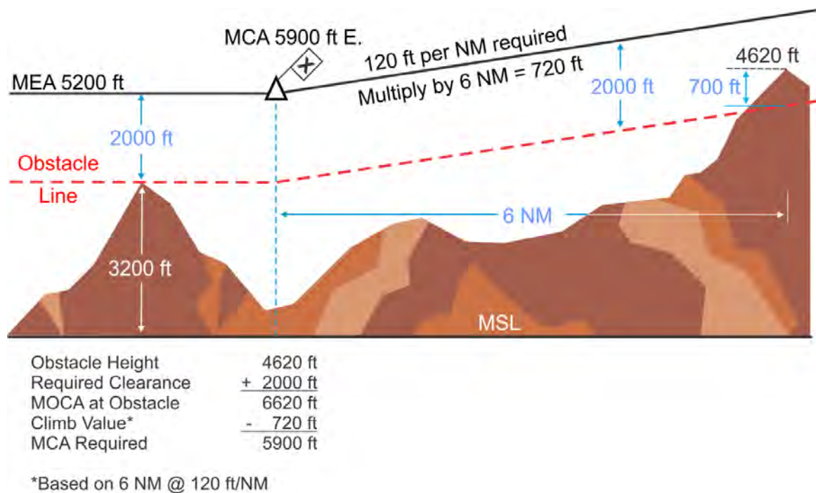
Figure 14-3-1. MCA Determination Point
