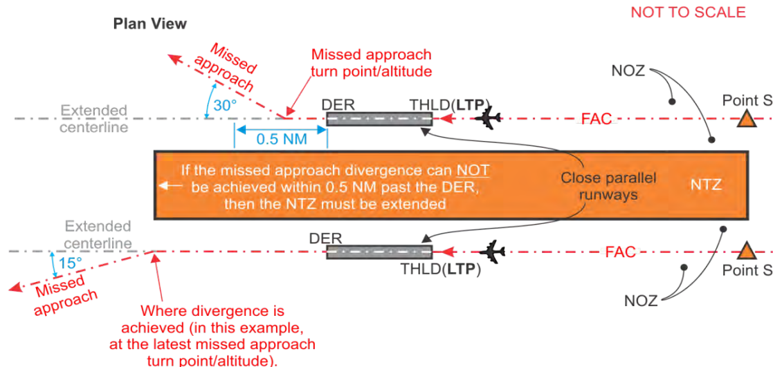
Figure 15-2-1. Missed Approach Divergence Delayed Beyond 0.5 NM
