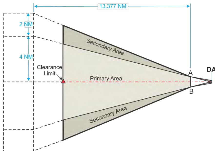
Figure 10-3-3. Section 2, Straight Missed Approach Area with PCG
