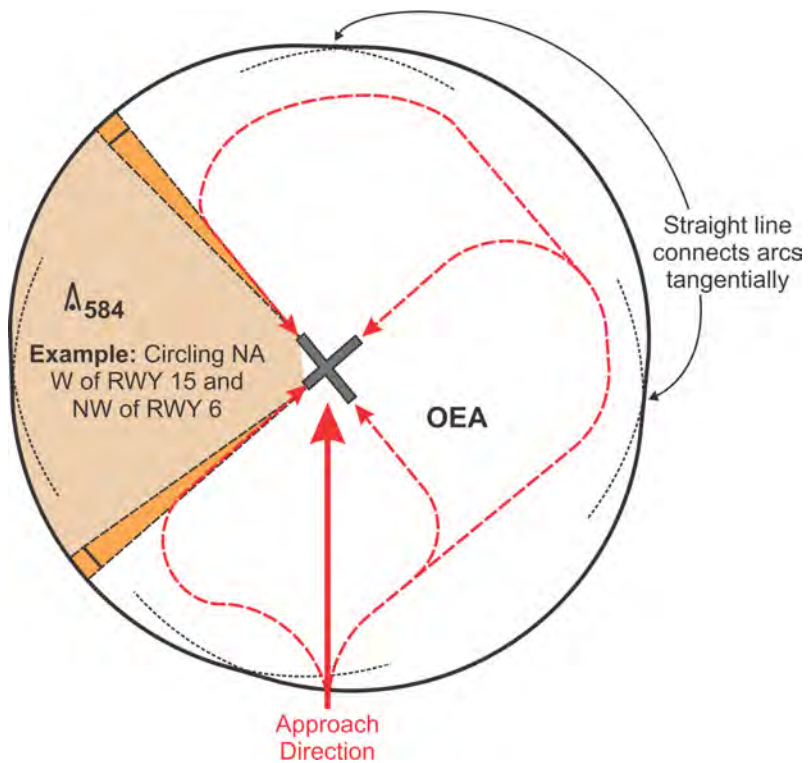
Figure 2-7-4. Complex Restricted Circling Area, Circling Aligned Approach (<180 Degrees)
