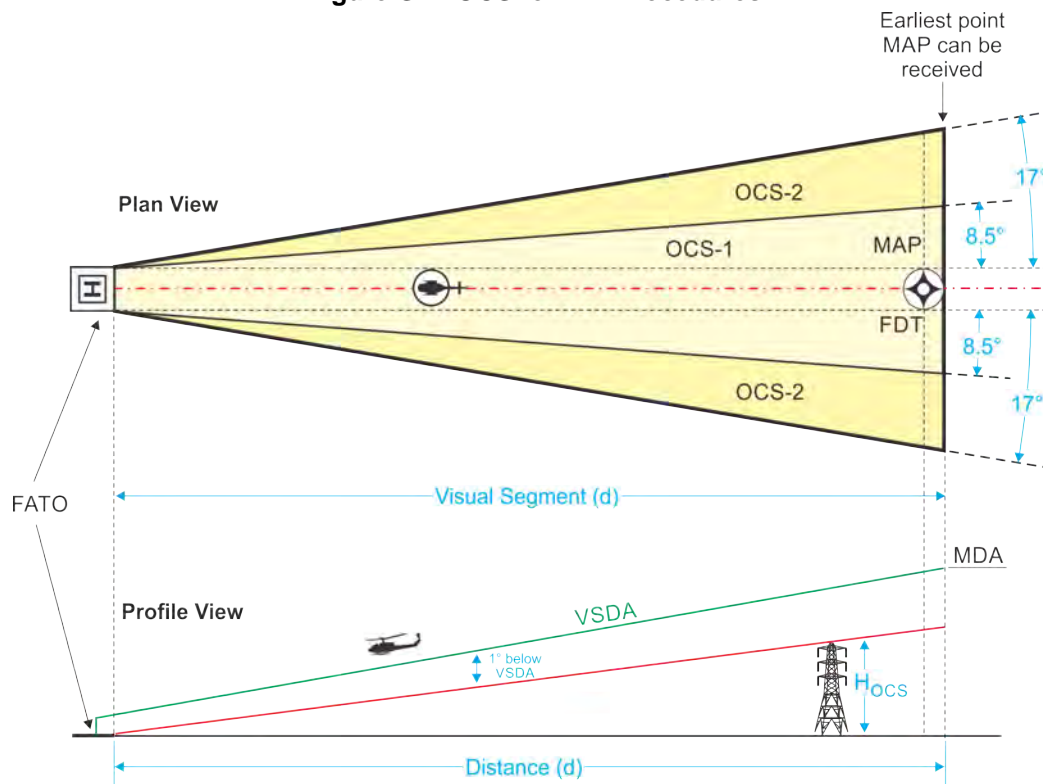
Figure G-2. OCS for IVH Procedures
