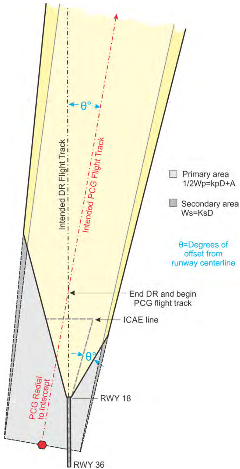
Figure 13-3-5. DER within Primary Area Facility, On Airport NAVAID
