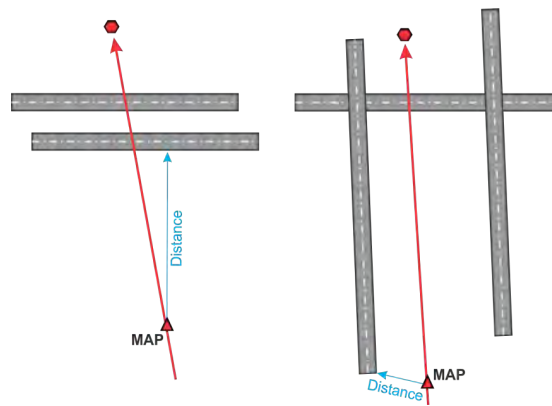
Figure 3-3-5. MAP to Nearest Landing Surface, Circling Aligned
