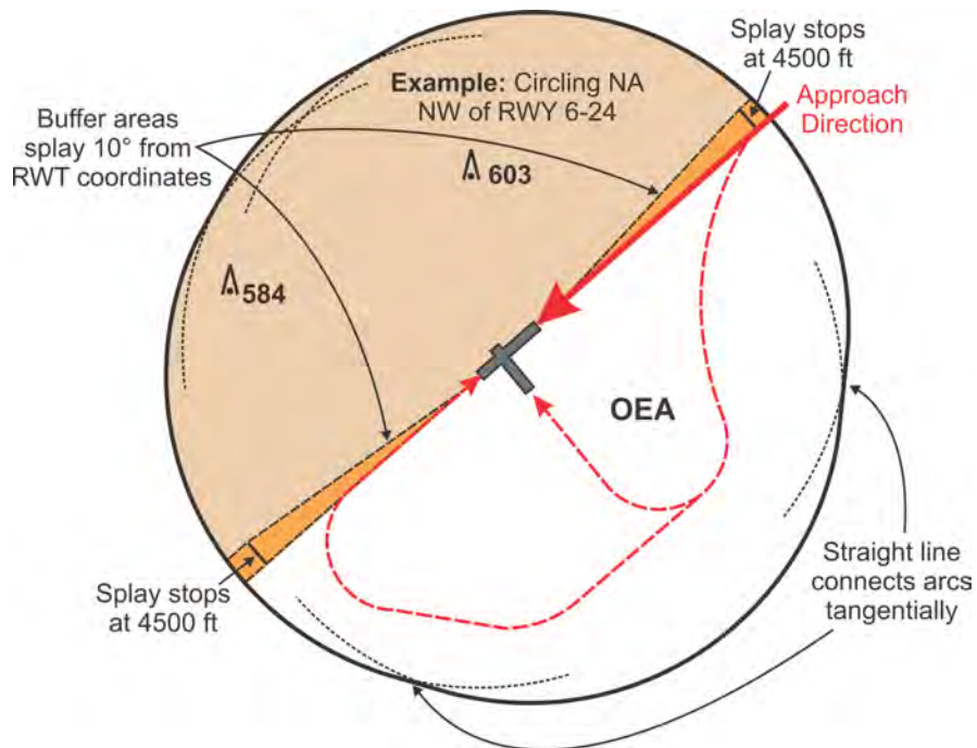
Figure 2-7-2. Simple Restricted Circling Area, Straight-in Aligned Approach
