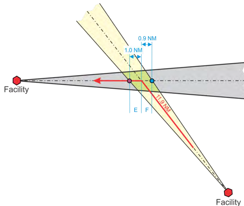
Figure 2-9-4. Measurement of PFAF Error
