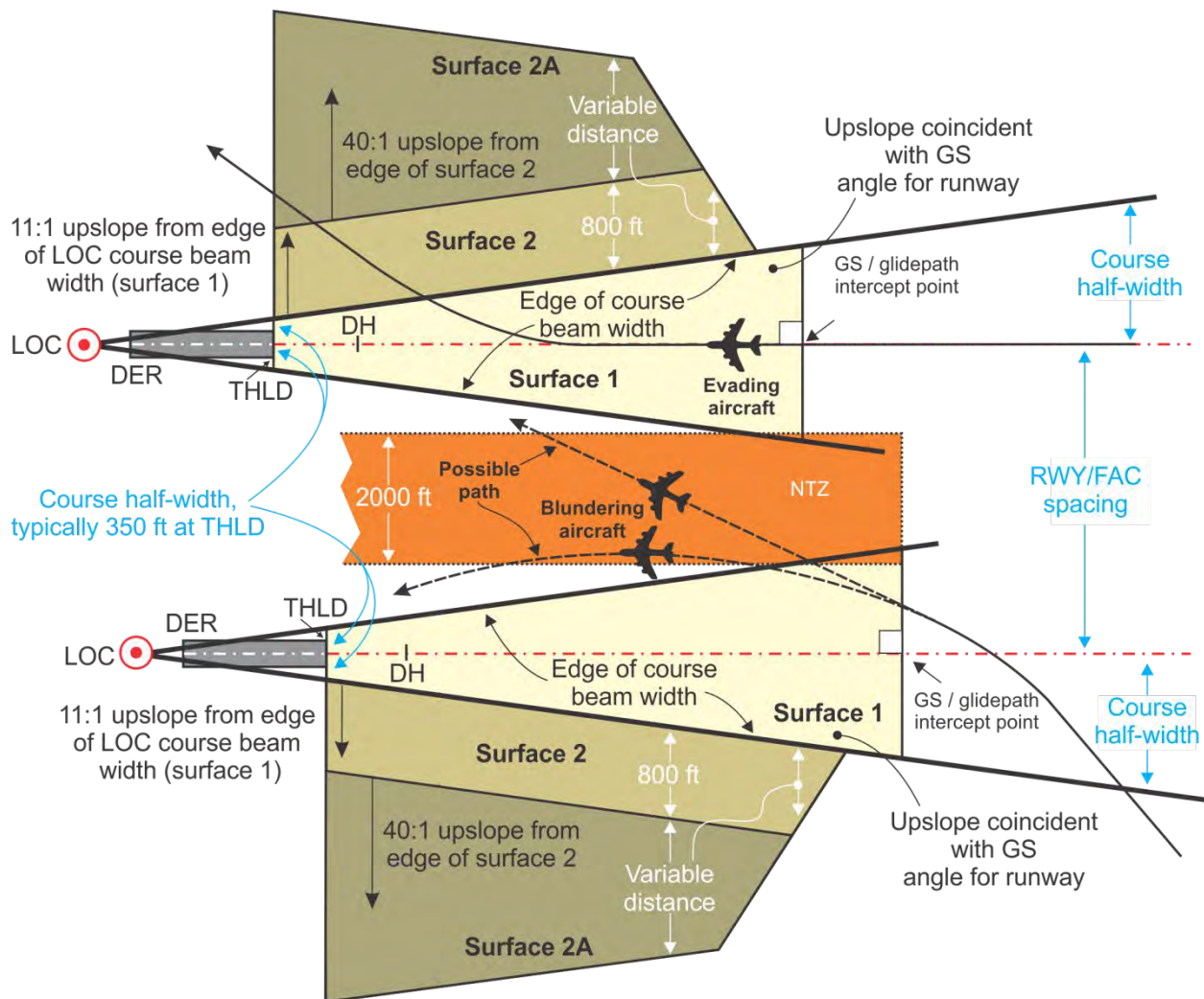
Figure E-9. Parallel Approach Obstacle Assessment Surface 2
