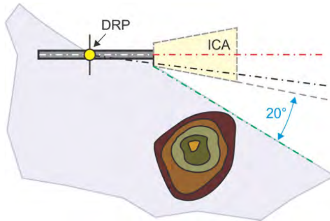
Figure 13-2-8. Boundary Based on ICA
