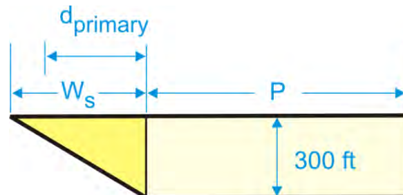
Figure 7-1-3. Final Approach Area ROC
