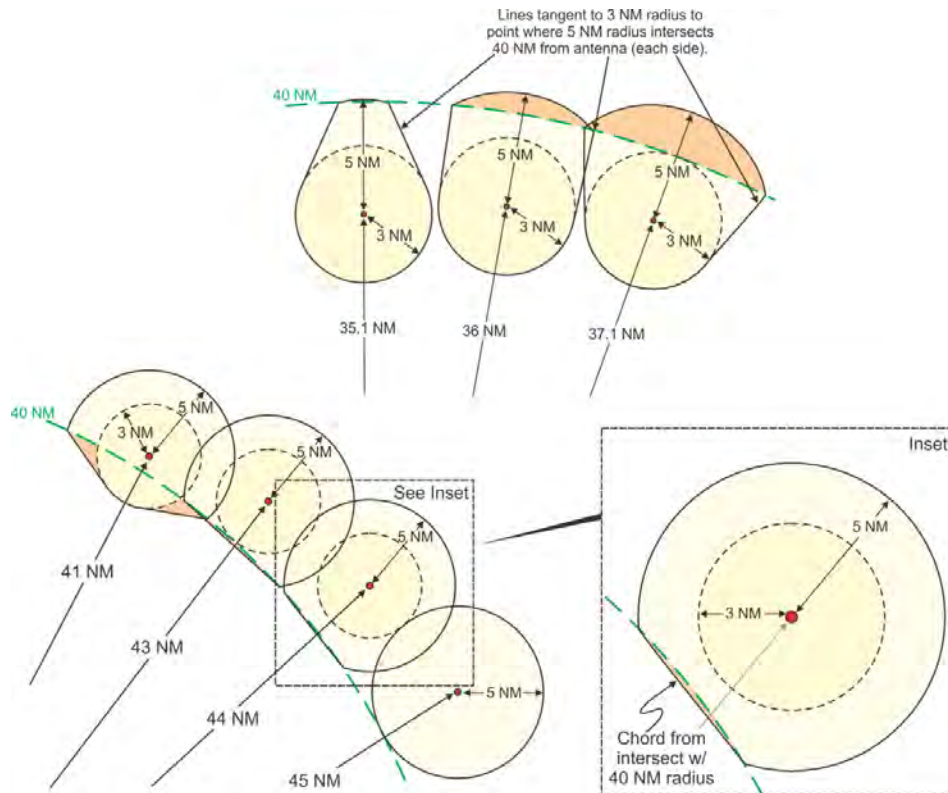
Figure 11-3-7. Isolation Area, Point Feature, Example Construction > 35 NM from Radar (Single Sensor, w/out Reinforced MSSR)
