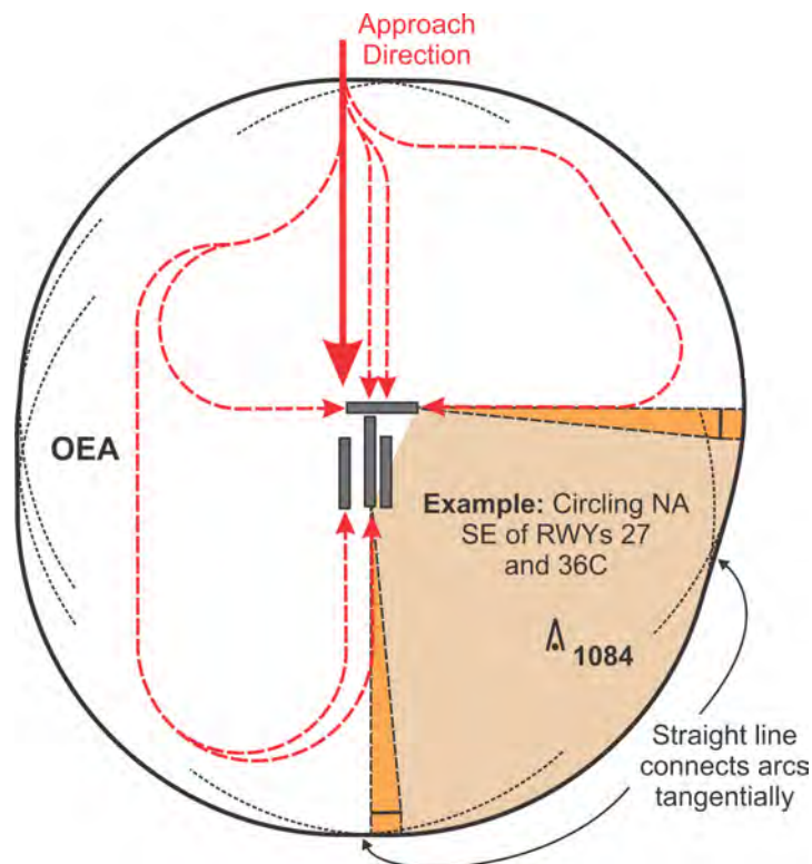
Figure 2-7-6. Complex Restricted Circling Area, Straight-in Aligned Approach (<180 Degrees, Parallel Runways)
