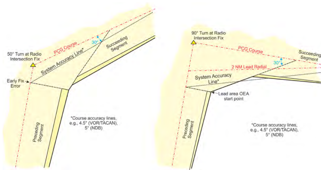
Figure 13-3-14. Inside Turn Area Construction Over a Radio Fix
