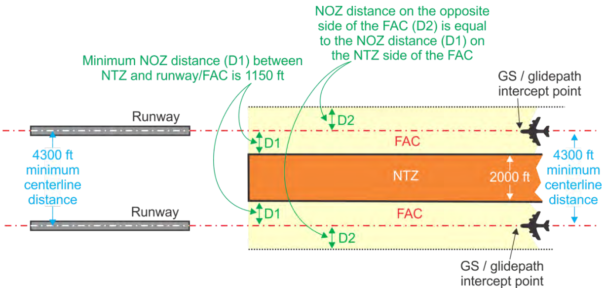
Figure E-6. Simultaneous Parallel Runway Approach Zones
