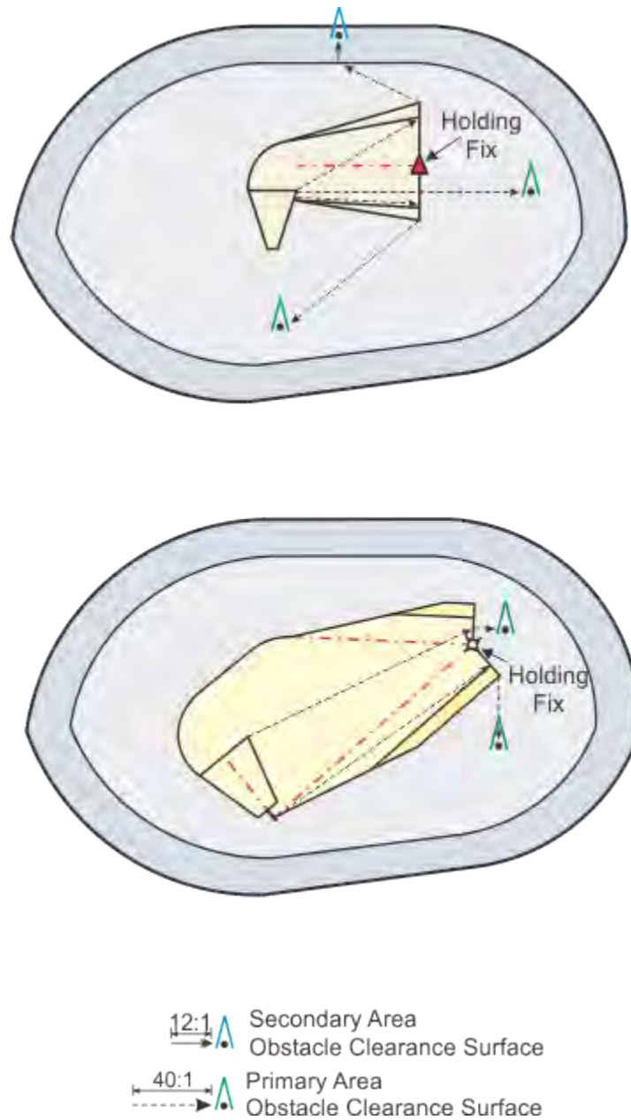
Figure 16-7-1. Climb-in-Hold Obstacle Evaluation
