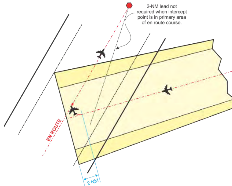
Figure 13-3-28. Turn onto En Route Course
