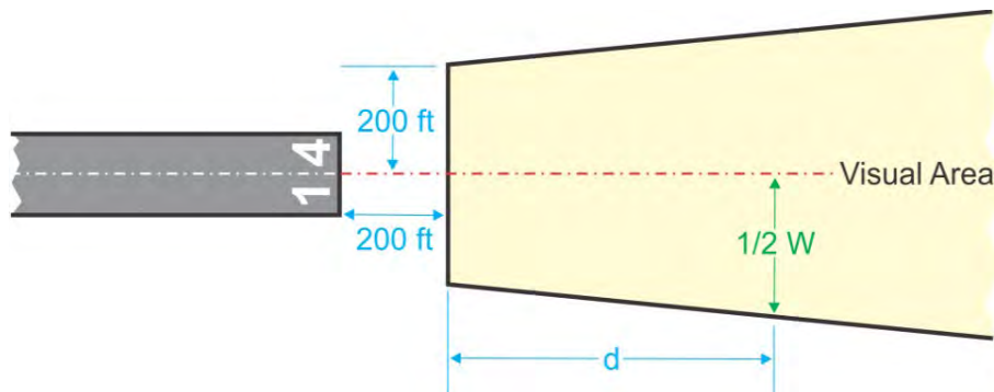
Figure 3-3-2. Circling and Straight-In Visual Area for Approach to a Runway
