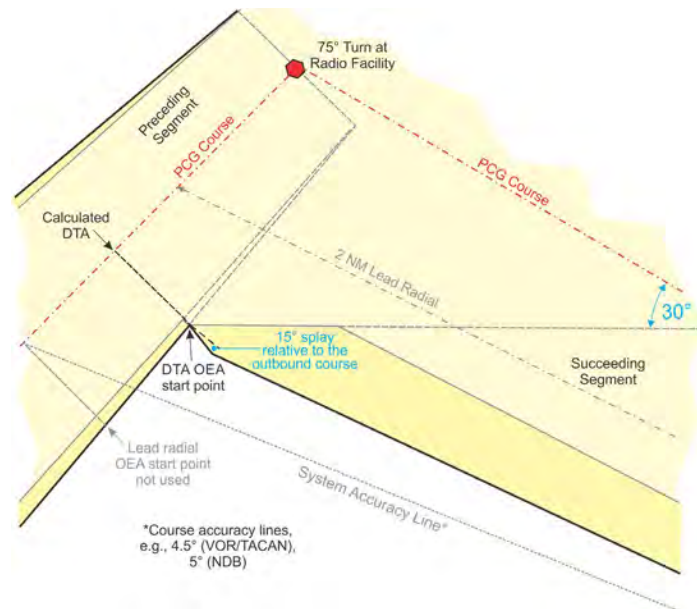
Figure 13-3-15. Inside Turn Area Construction, 75° Turn Over Radio Facility
