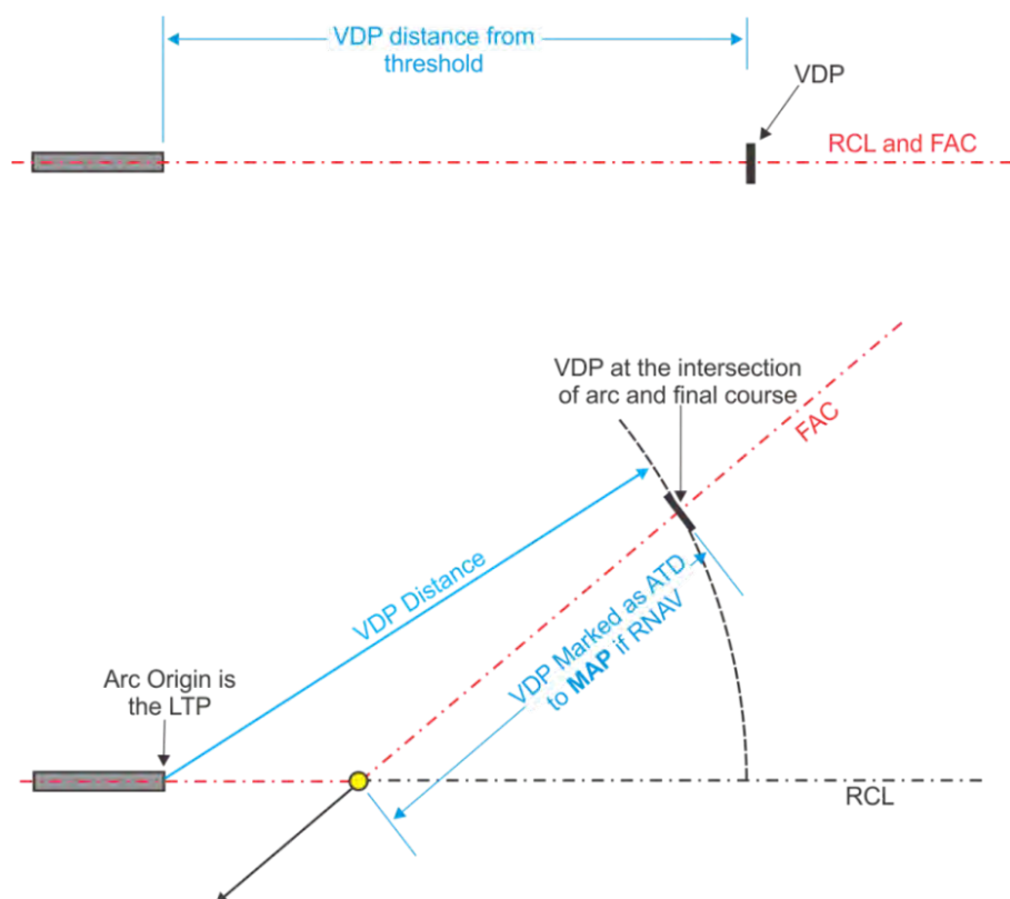
Figure 2-6-4. VDP Location
