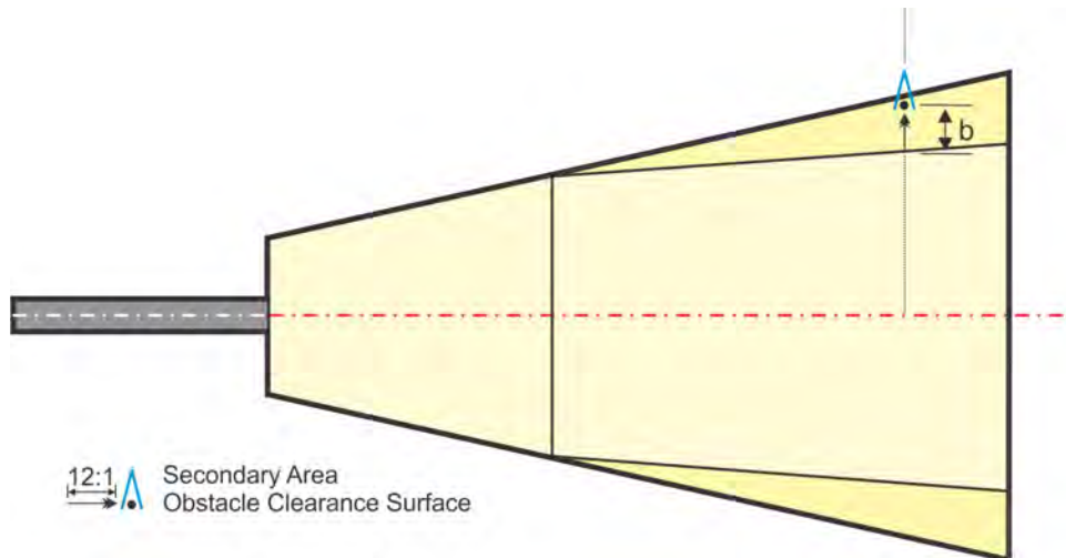
Figure 13-1-3. Secondary OCS
