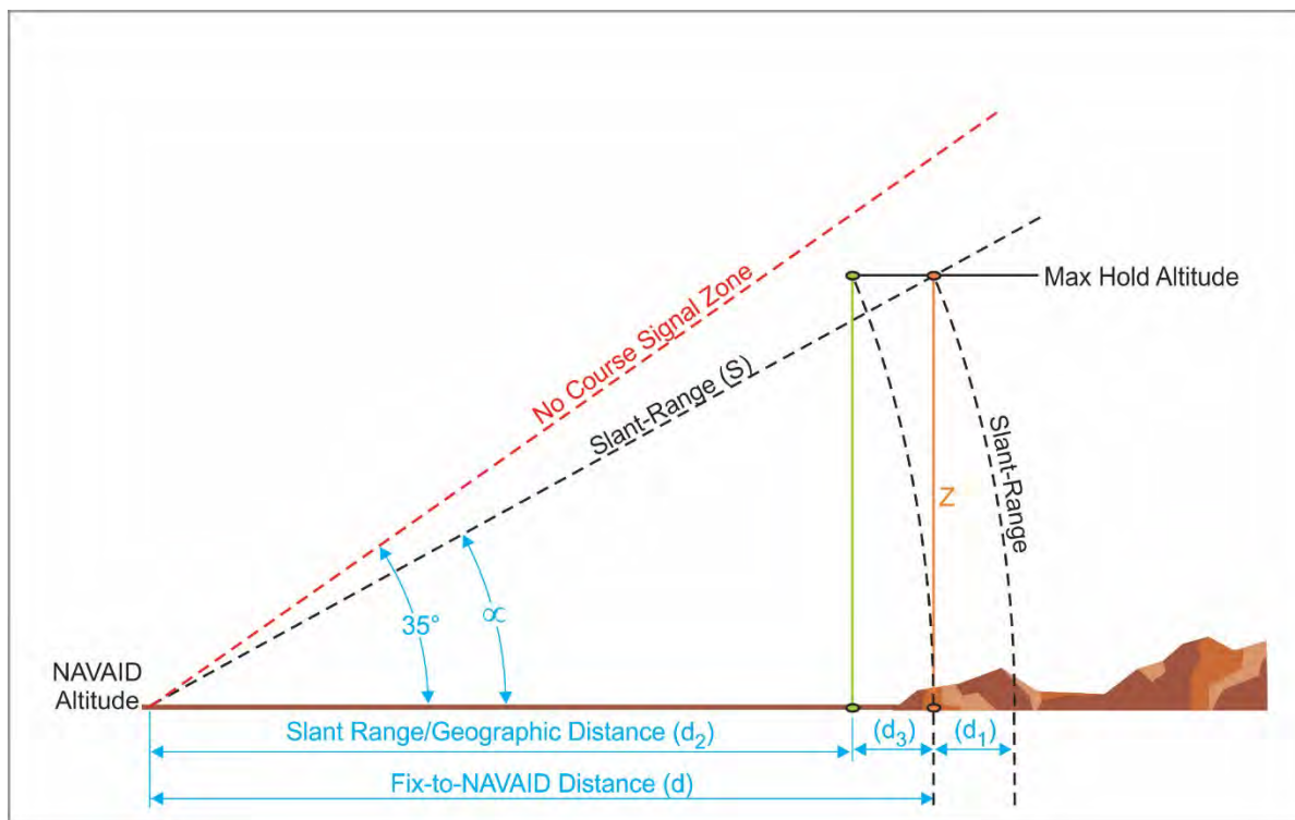
Figure 16-14-1. Holding Calculations Relationships
