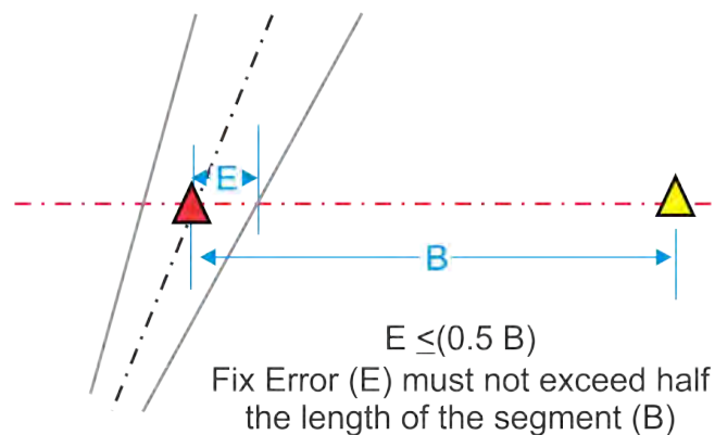
Figure 2-9-3. Intermediate, Initial, or Feeder Approach Fix Errors
