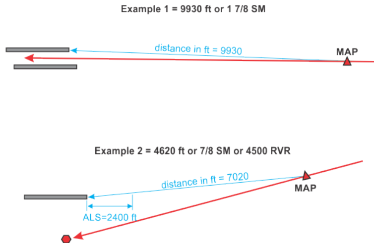
Figure 3-3-1. MAP to LTP Distance Straight-in Aligned
