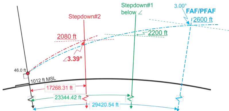
Figure 2-6-3. VDA with Stepdown Fixes
