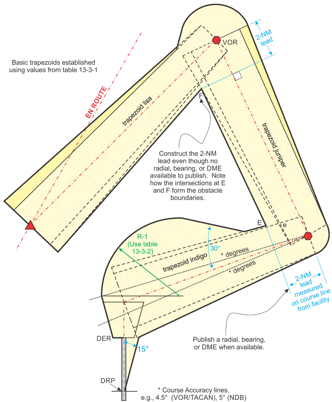
Figure 13-3-11. Multiple Turns
