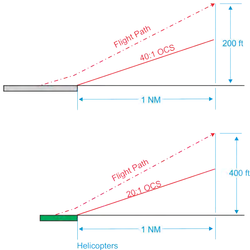
Figure 13-1-4. Standard Climb Gradient
