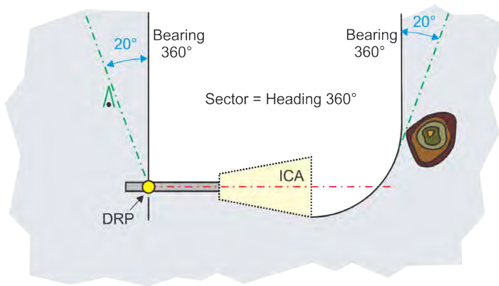
Figure 13-2-12. Parallel Boundaries
