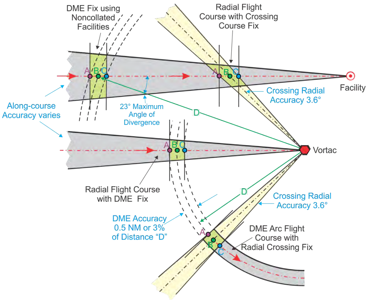
Figure 2-9-1. Fix Displacement
