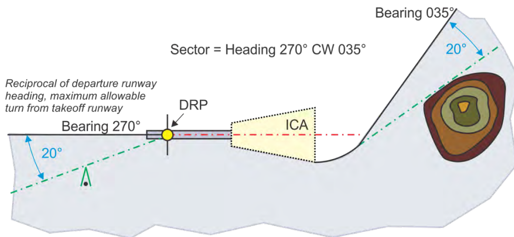
Figure 13-2-11. Maximum Heading Limitation
