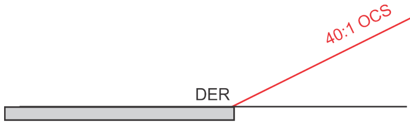
Figure 13-1-2. OCS Starting Elevation With Clearway
