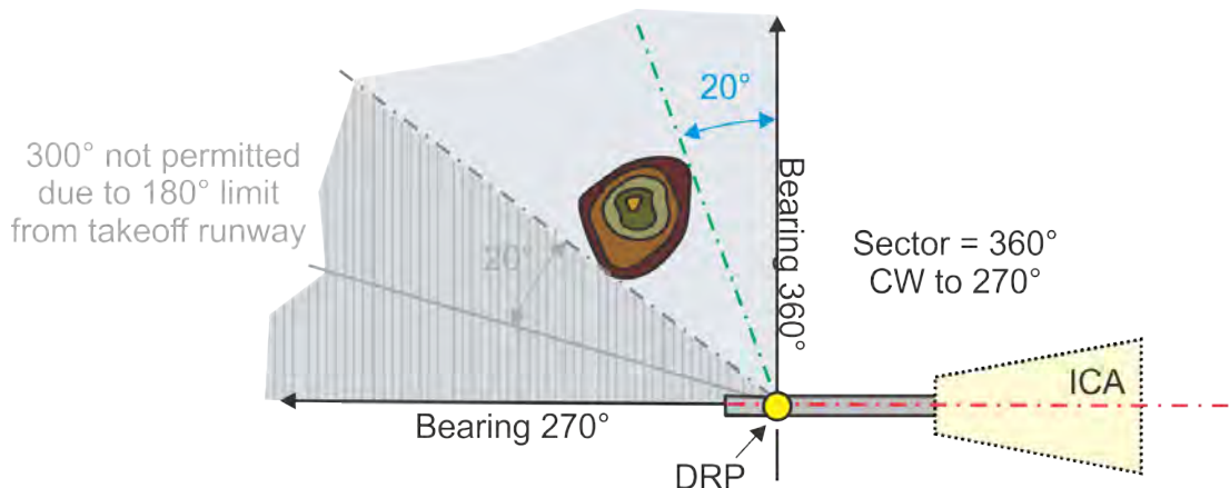
Figure 13-2-11. Maximum Heading Limitation
