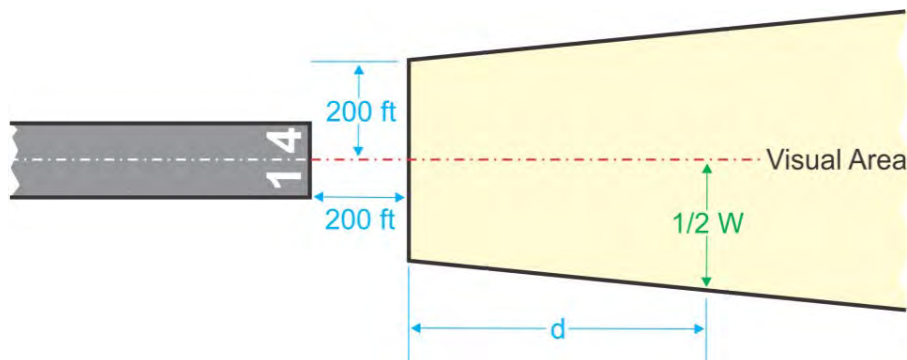
Figure 3-3-2. Circling and Straight-In Visual Area for Approach to a Runway
