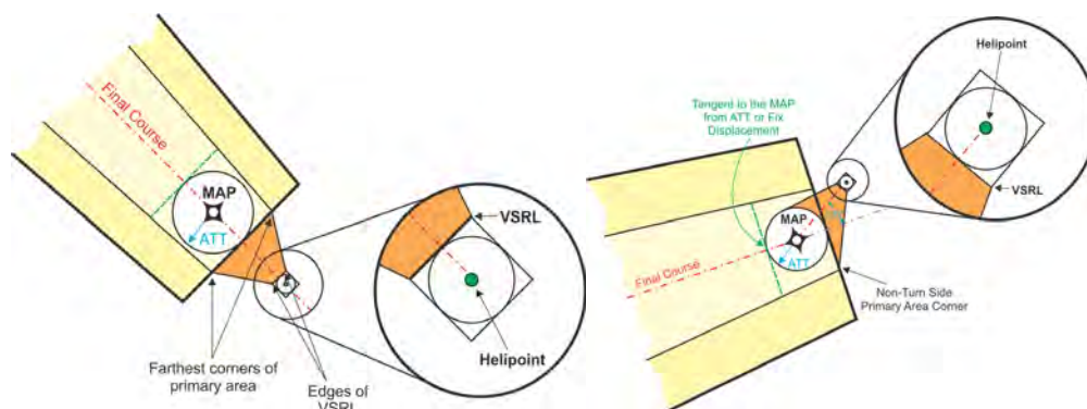
Figure 12-2-2. Visual Segment Area
