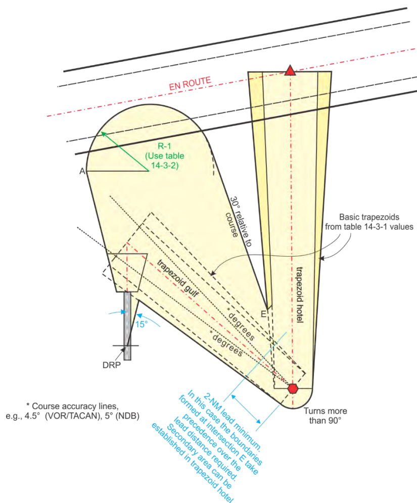
Figure 13-3-10. Climb to Intercept Course
