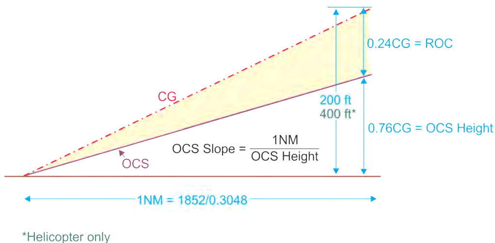
Figure 2-1-4. Climb Segment
