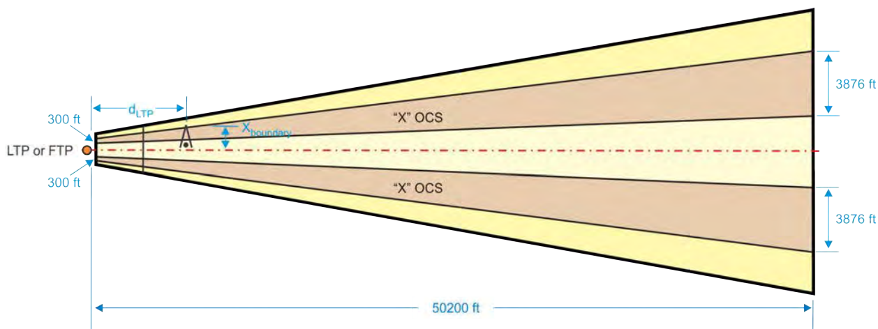
Figure 10-2-5. "X" OCS
