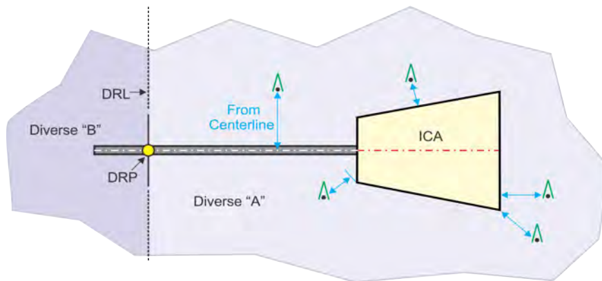
Figure 13-2-3. Diverse "A" Area Evaluation
