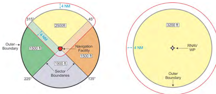
Figure 2-3-1. MSA
