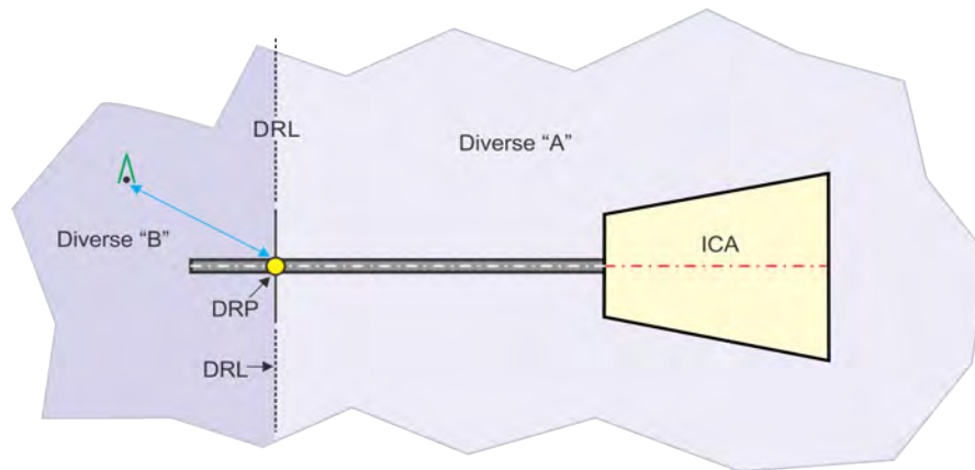
Figure 13-2-5. Diverse "B" Area
