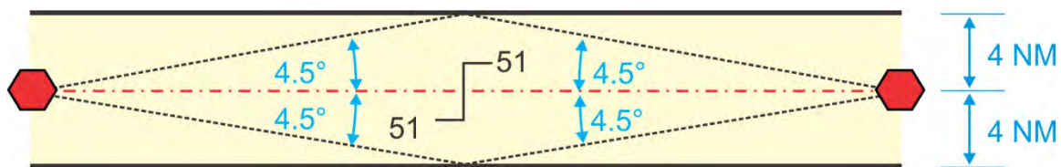
Figure 14-1-1. Primary Obstacle Clearance Area
