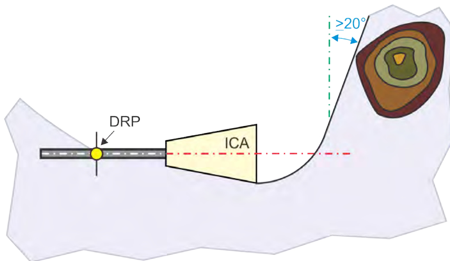
Figure 13-2-9. Outer Boundary
