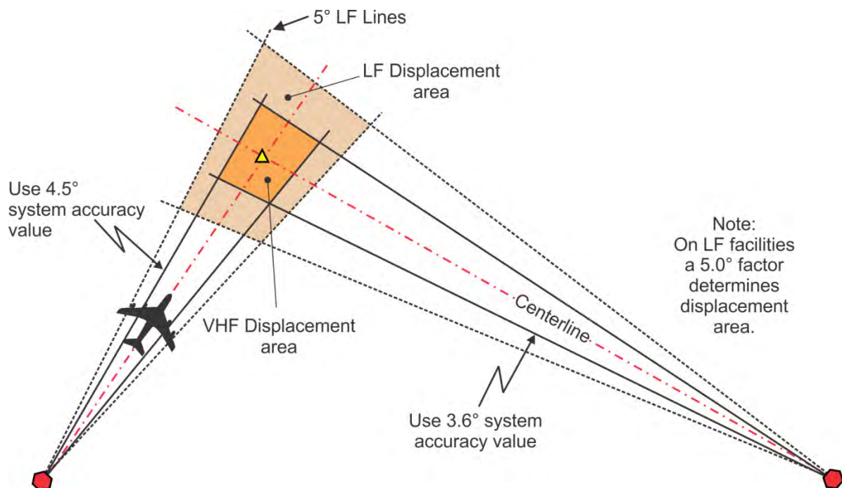
Figure 14-1-6. Fix Displacement
