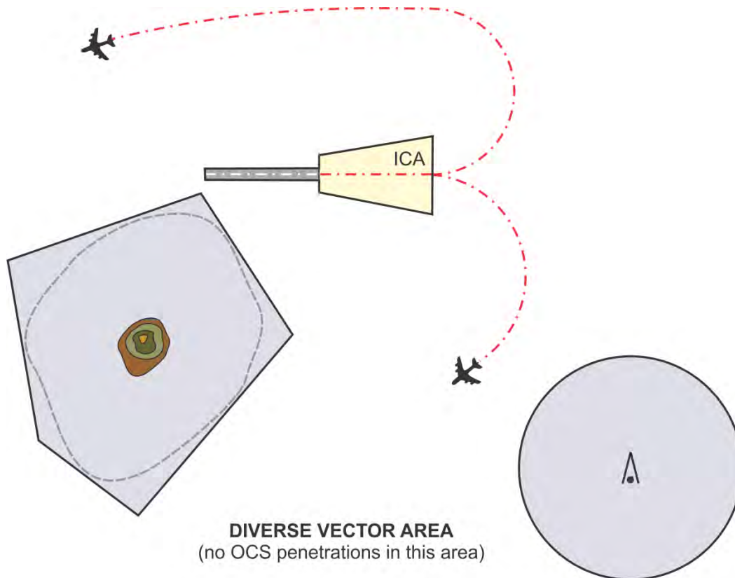
Figure 13-5-1. Isolation Areas
