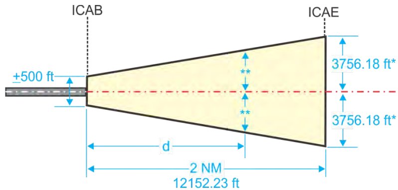
Figure 13-1-5. Initial Climb Area: Standard
