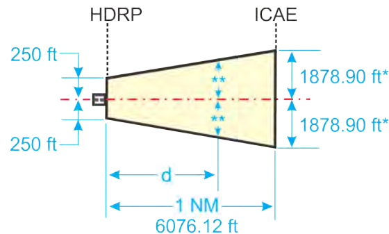
Figure 13-1-6. Initial Climb Area: Helicopters
