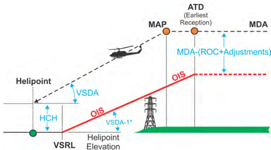
Figure 12-2-3. VSDA and Associated OIS
