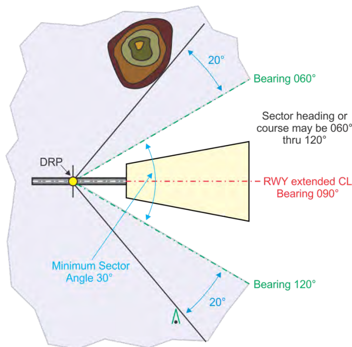
Figure 13-2-7. Minimum Sector Area
