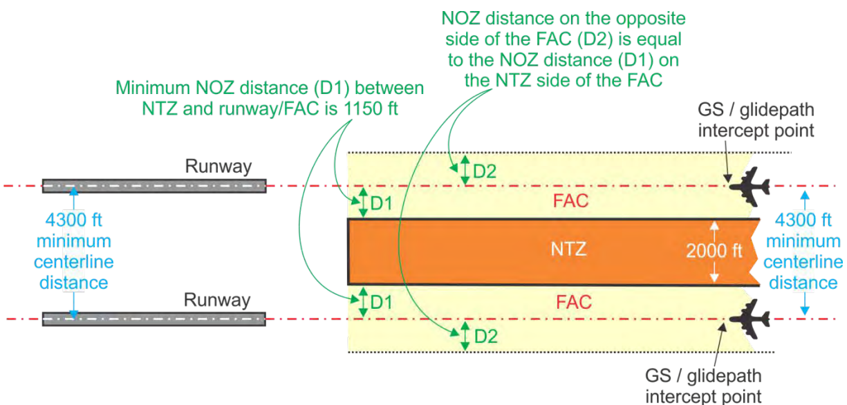
Figure E-10. Simultaneous Parallel Runway Approach Zones
