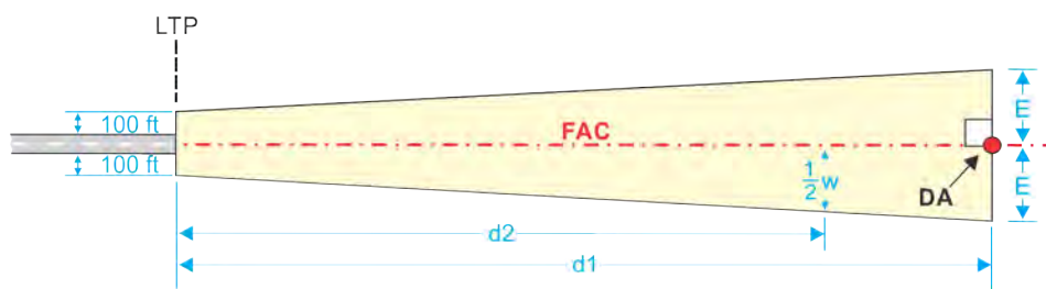
Figure 2-6-5. VGS Area
