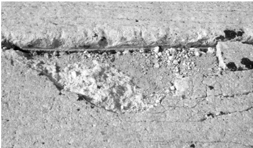
▲ Failed joint with severe spalling and pothole.
