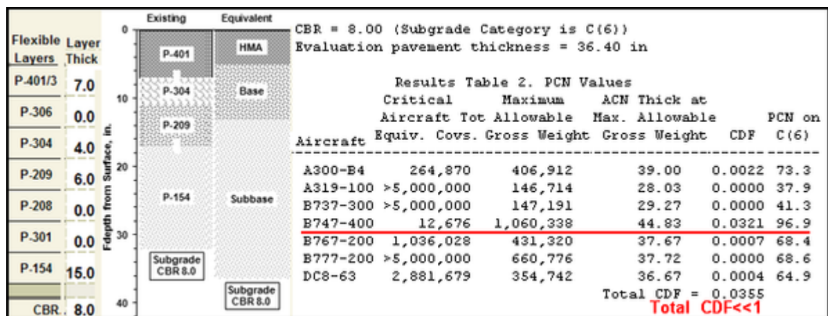
Figure D-4. COMFAA PCN Results – Flexible Pavement Overload Option Two
