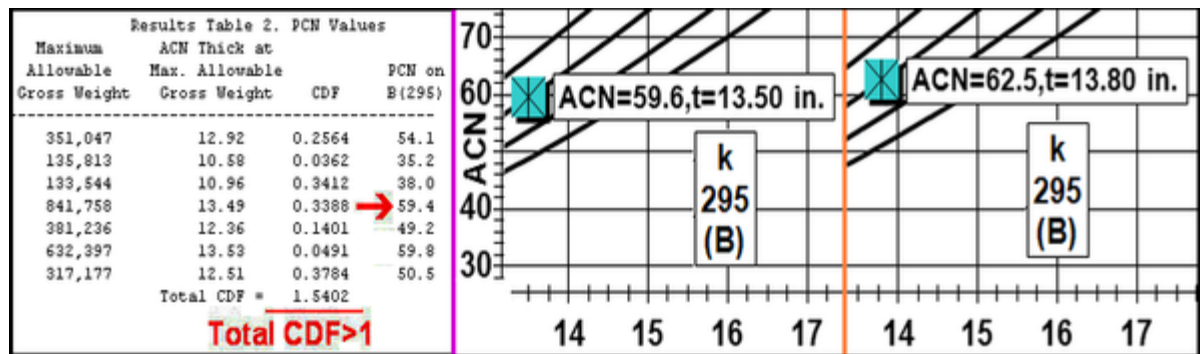
Figure D-6. CDF-PCN Results for the B-747-400 – Rigid Pavement Overload Option One
