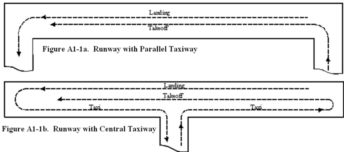
Figure A-1. Traffic Load Distribution Patterns
