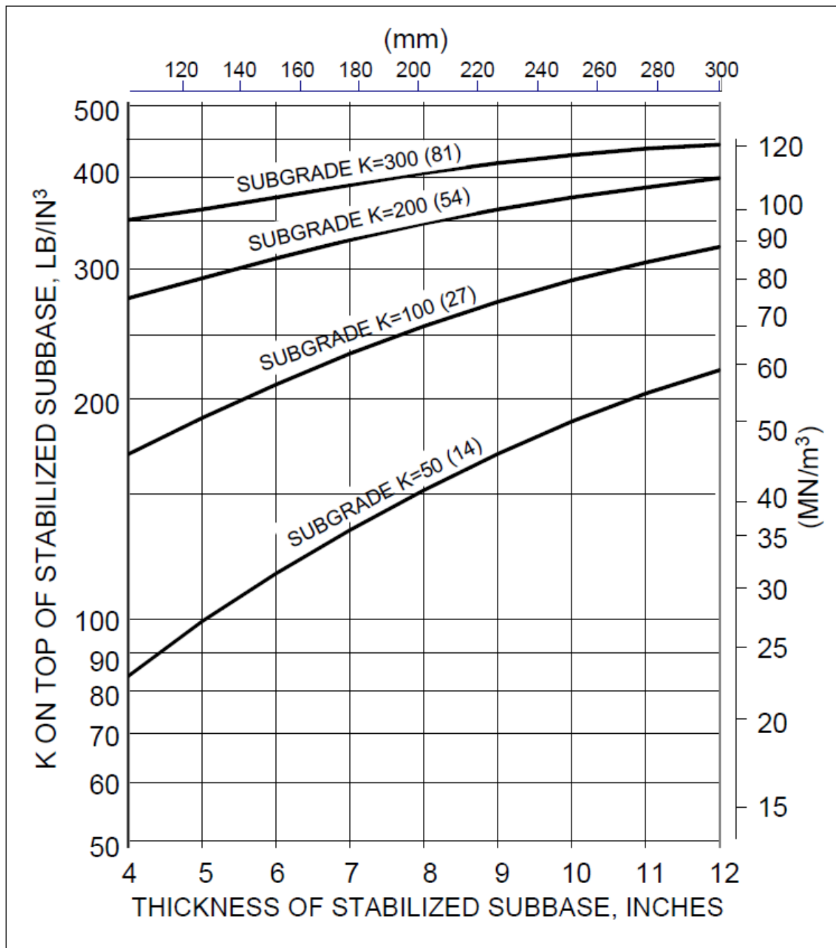
Figure B-6. Stabilized Subbase Layer Effect on Subgrade Support, k, for Rigid Pavement (FAA Westergaard method)
