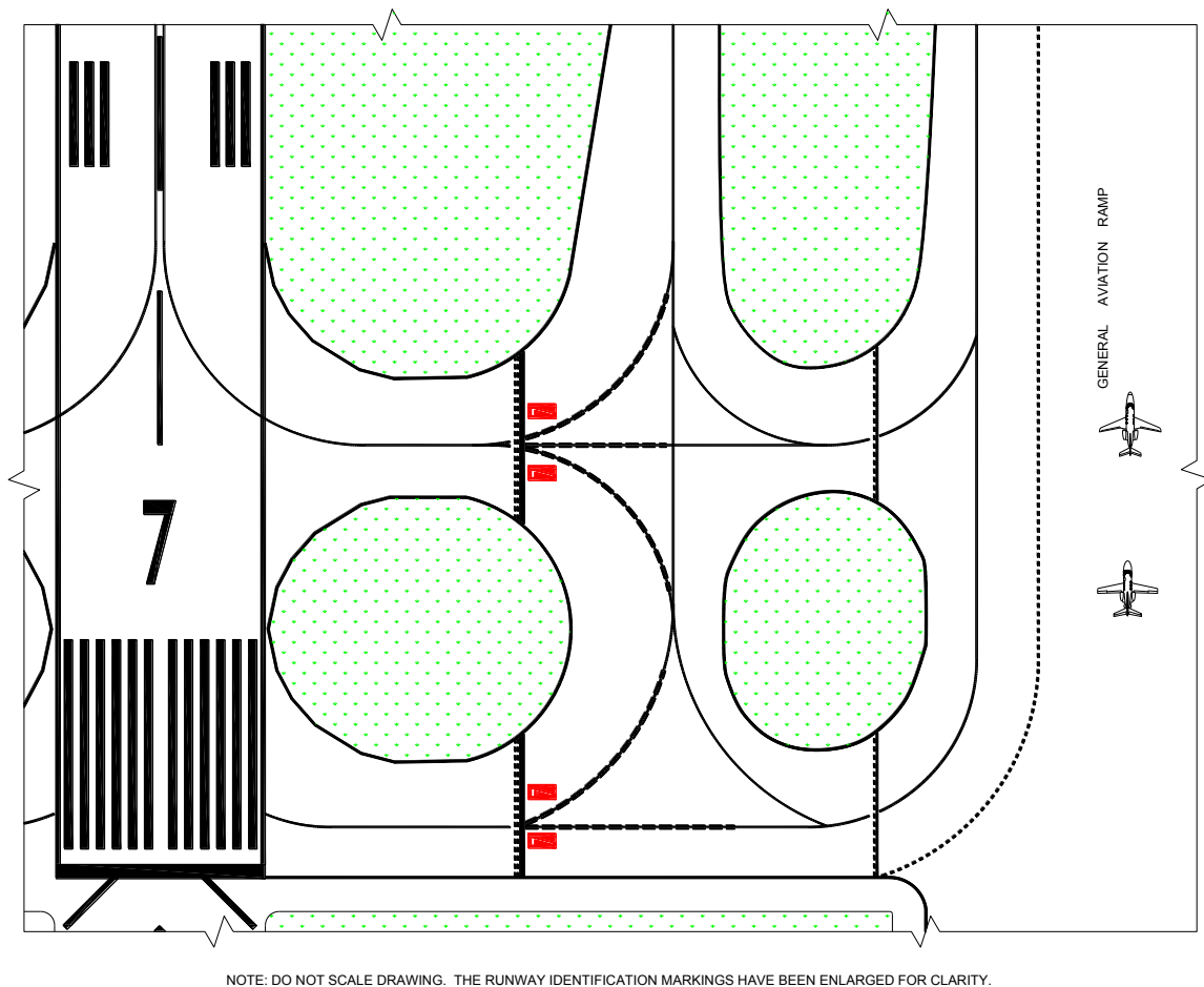
Figure 5-1 Precautionary Placement of the Non-movement Boundary Marking
