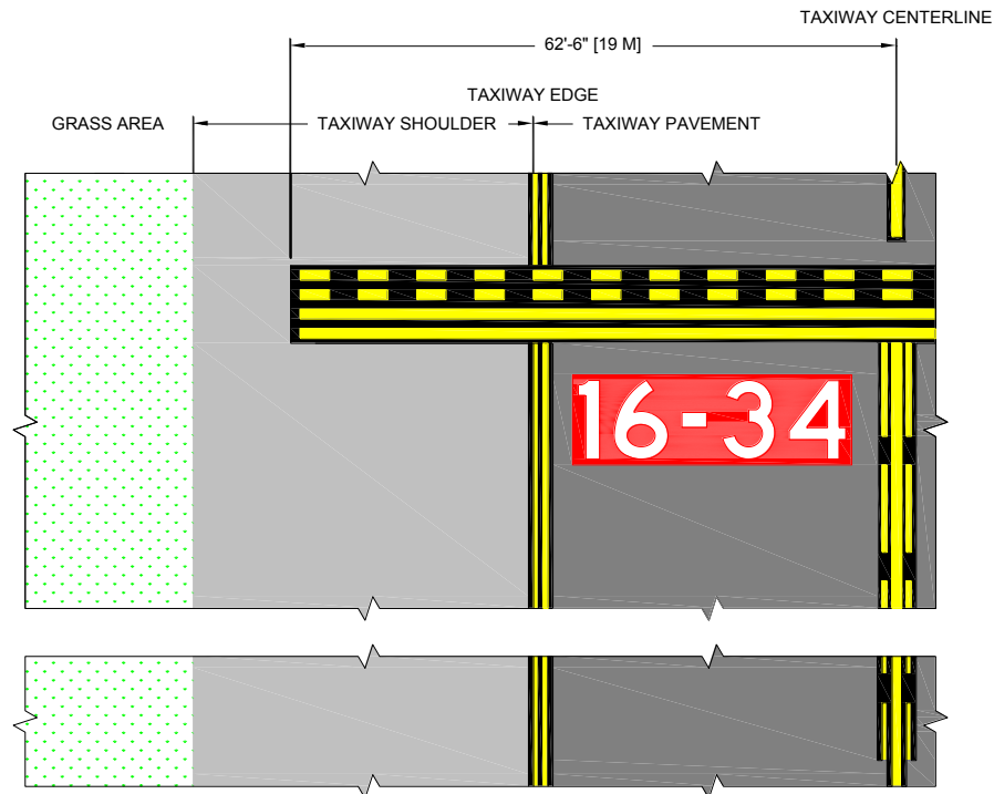
Figure C - 4. Enhanced Runway Holding Position Markings on Taxiways
