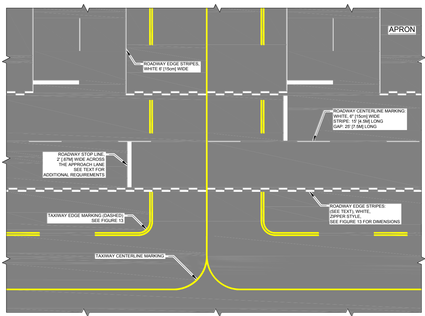
Figure 23. Vehicle Roadway Markings
