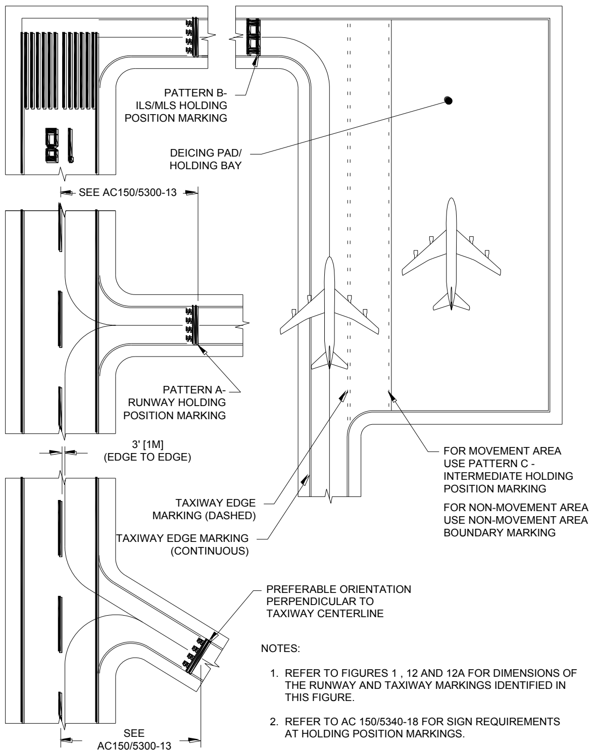
Figure 14. Taxiway Markings
