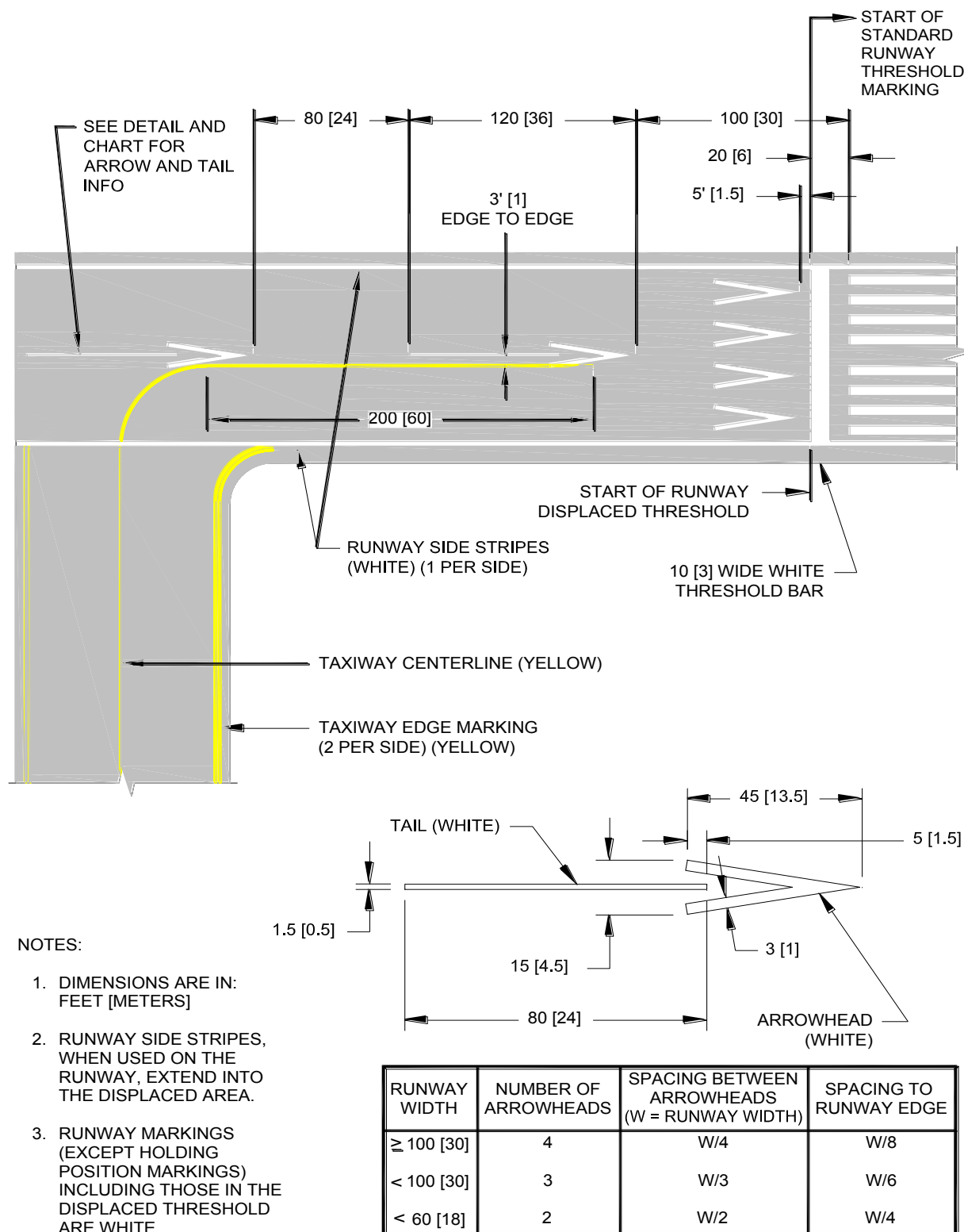
Figure 6. Displaced Threshold Markings
