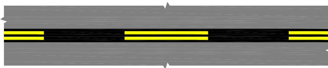
Figure B - 4. Dashed Taxiway Edge Line Marking
