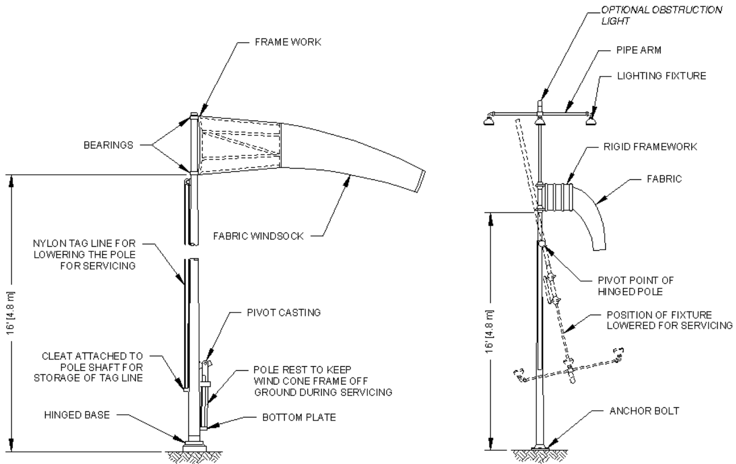
Figure 2. Typical Type L-807 supports
