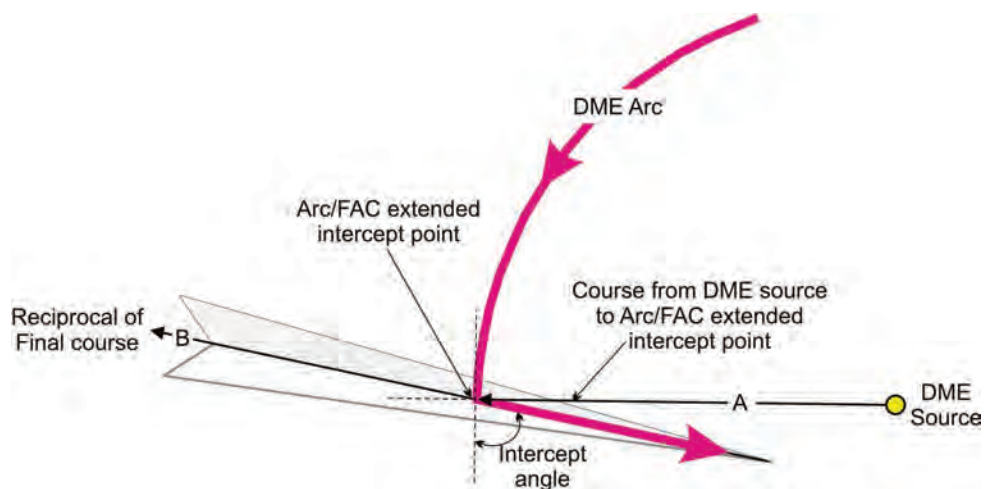
Figure 2-2A. DME Source on Arc Side
