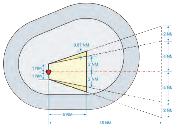
Figure 107. Final Approach Primary and Secondary Area. On-Heliport VOR, No PFAF, Par 1132b. See also Figure 105.
