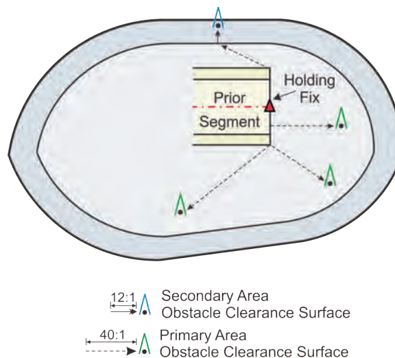
FIGURE 37-2. CLIMBING IN A HOLDING PATTERN. Par 293b.
