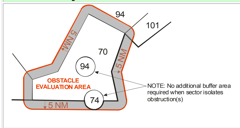
Figure 10-6. Multi-sensor Buffer Areas.
