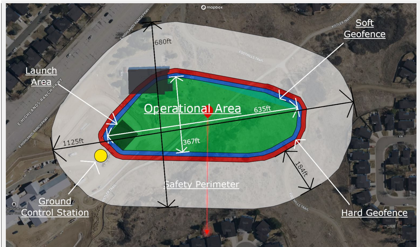
Figure 4: Additional Airspace / Site Assessment Screenshot
