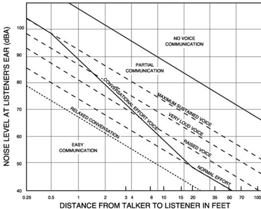
Figure E-5 Outdoor Speech Intelligibility
