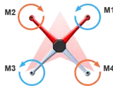
Quad-rotor X
