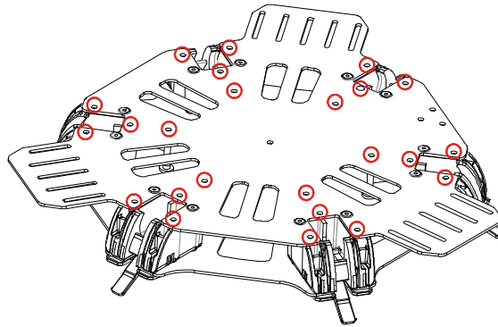
Fig.3 Fix the screws
