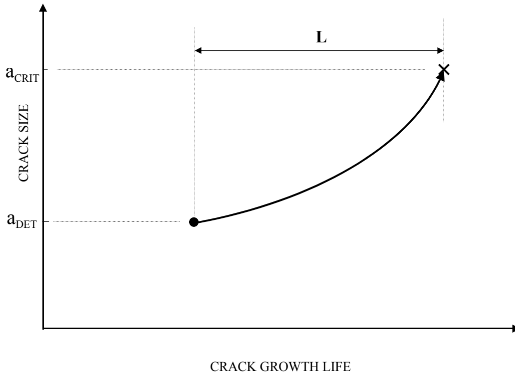
Figure 1 Single Load Path Structure Basis for Inspection Interval
