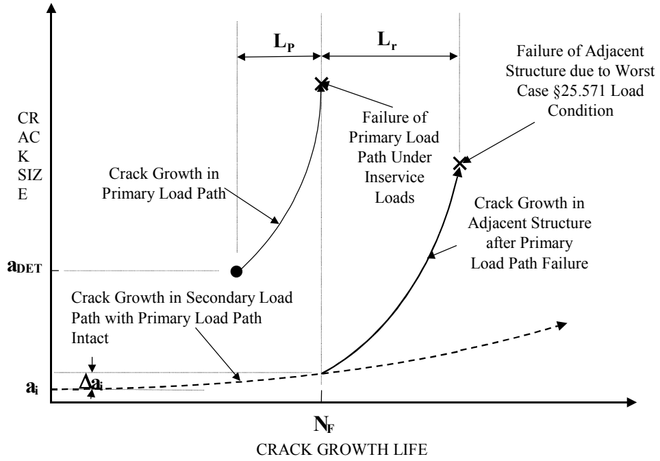
Figure 3 Inspection Interval Determination for Multiple Load Path Structure Based on Crack Growth and Residual Strength Evaluations
