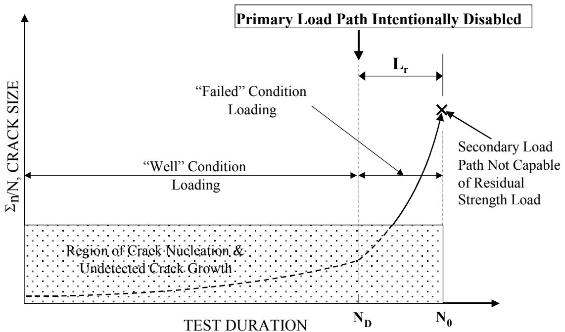
Figure 2. Multiple Load Path Structure Evaluation by Test to Support Inspection for Failed Load Path
