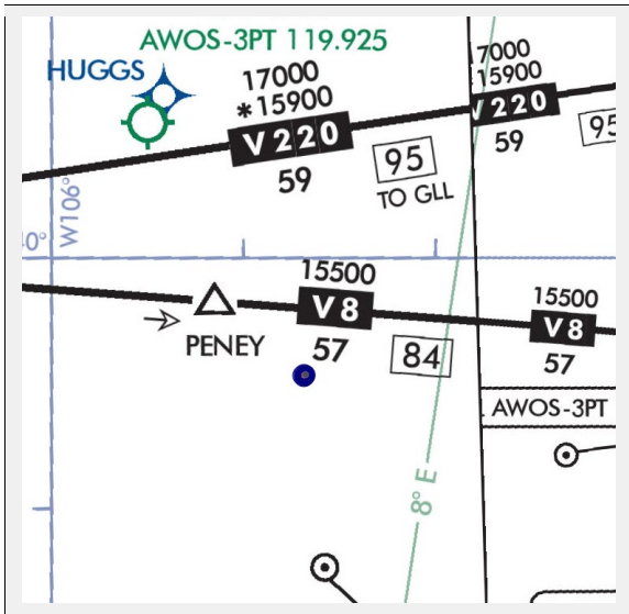
Figure 3: IFR Low Altitude Enroute Chart / UASFM Overlay
