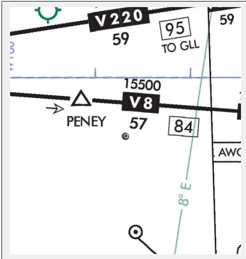
Figure 3: IFR Low Altitude Enroute Chart / UASFM Overlay
