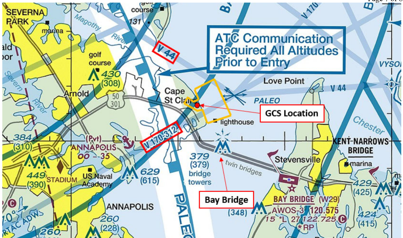
VFR SECTIONAL
