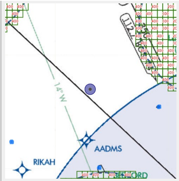
Figure 3: IFR Low Altitude Enroute Chart / UASFM Overlay
