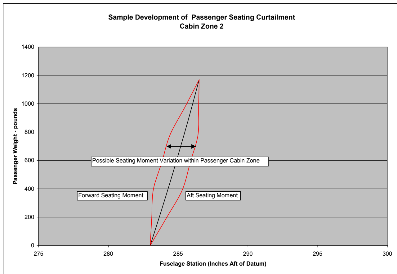
FIGURE 3-3. SAMPLE PASSENGER SEATING MOMENT (ZONE 2)
