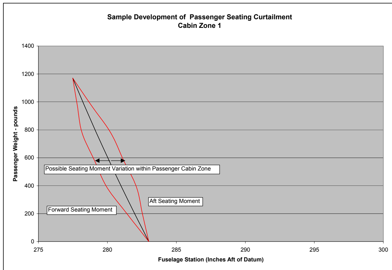
FIGURE 3-2. SAMPLE PASSENGER SEATING MOMENT (ZONE 1)
