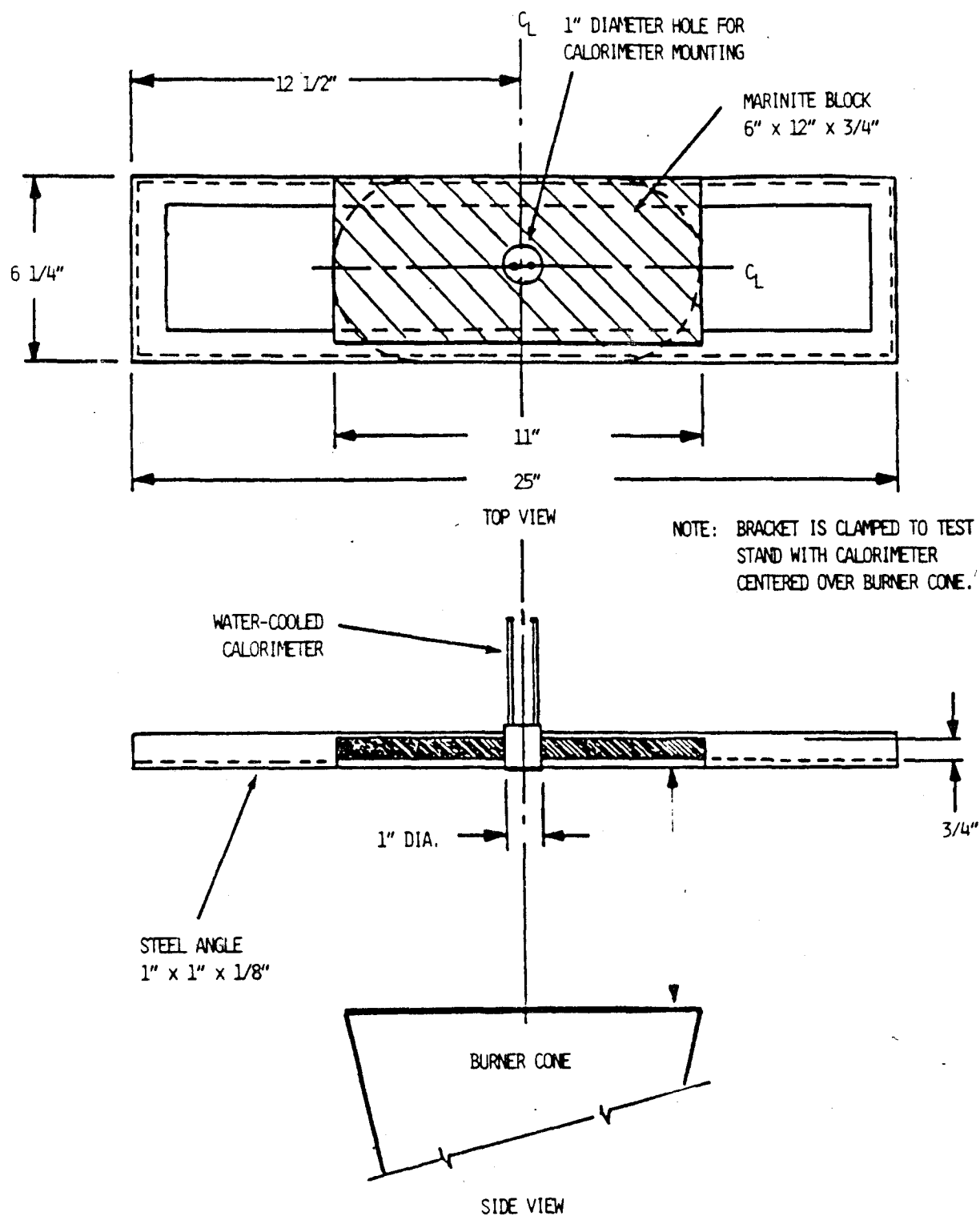
FIGURE 2. CALORIMETER BRACKET
