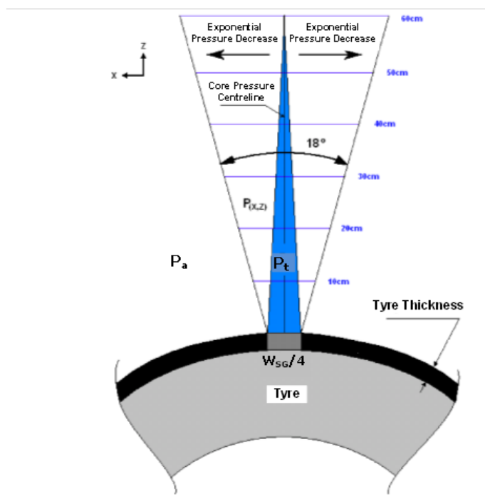
Figure 4b – Tyre Burst Pressure Effect – Bias Tyre
