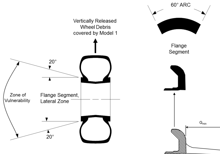
Figure 2 - Wheel Flange Release Threat
