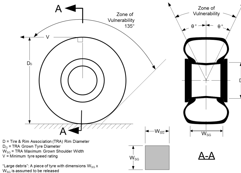
Figure 1 – Tyre Debris Threats
