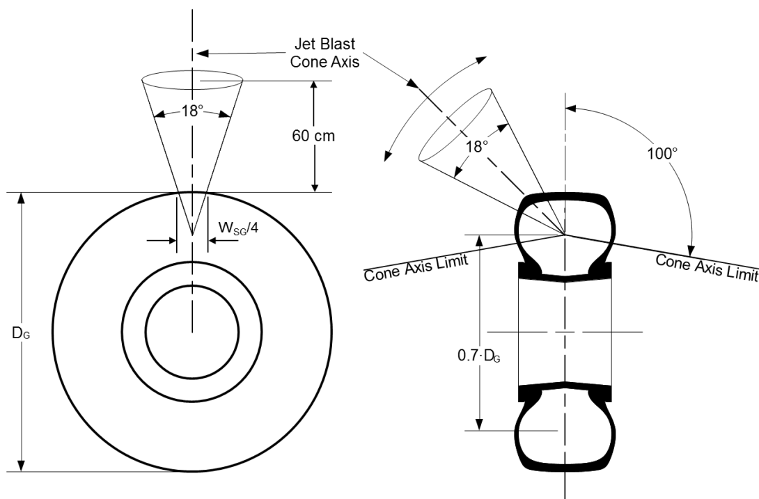
Figure 4a – Tyre Burst Pressure Effect – Bias Tyre
