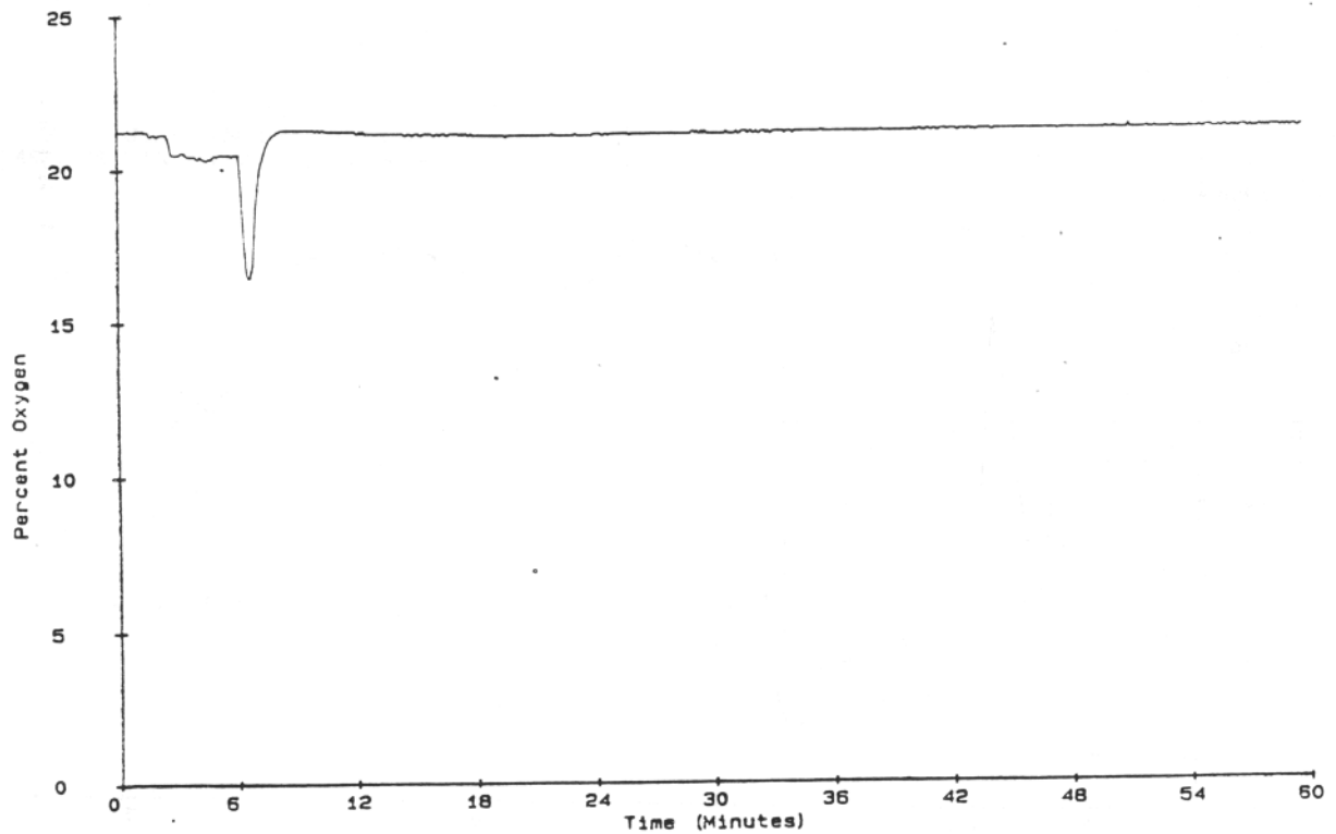
FIGURE 5. CONTAINER TEST NUMBER 16 - OXYGEN PROFILE
