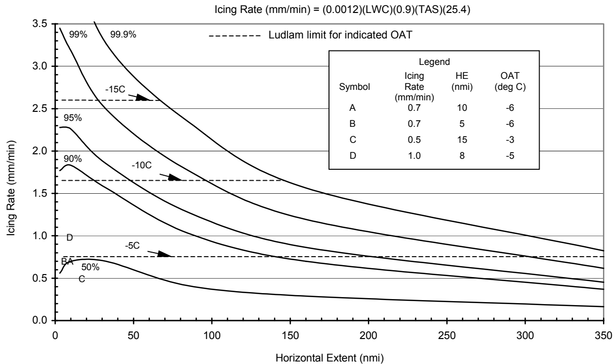
FIGURE 29. NATURAL PROBABILITIES FOR ICING RATES ON A 1/4-inch CYLINDER AT 150 kt IN STRATIFORM ICING CONDITIONS WITH AVERAGE MVDs (15 \mu m) AND IN-CLOUD TEMPERATURES OF 0° TO -10°C
