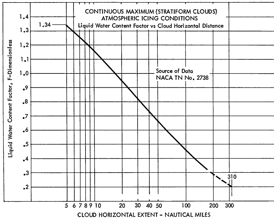
FIGURE 3. CONTINUOUS MAXIMUM (STRATIFORM CLOUDS) ATMOSPHERIC ICING CONDITIONS (Liquid water content factor vs cloud horizontal extent)
