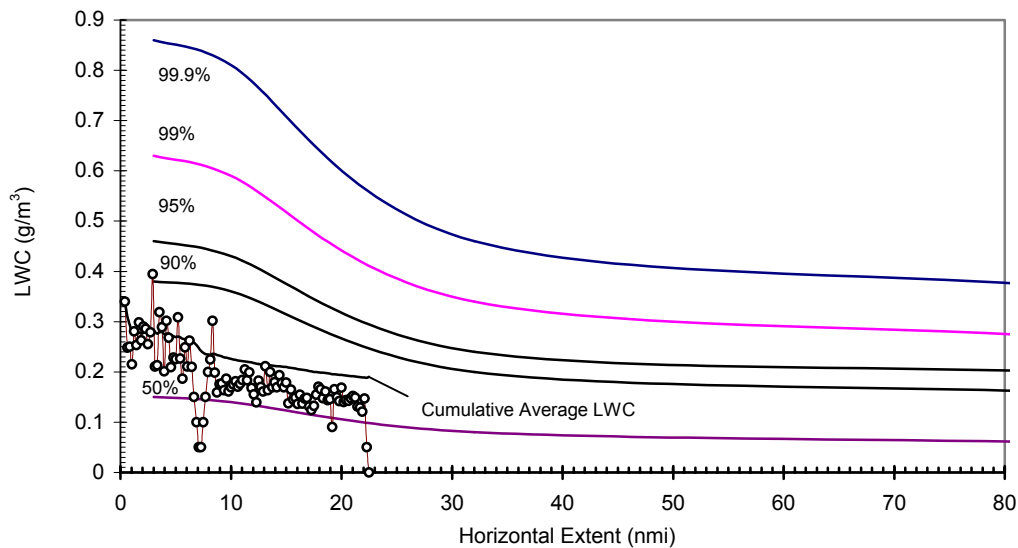
FIGURE 26. SAMPLE FLIGHT DATA (CLOUD GAP REMOVED) COMPARED WITH NATURAL PROBABILITIES FOR LWC AVERAGES AT ALTITUDES UP TO 2500 ft AGL
