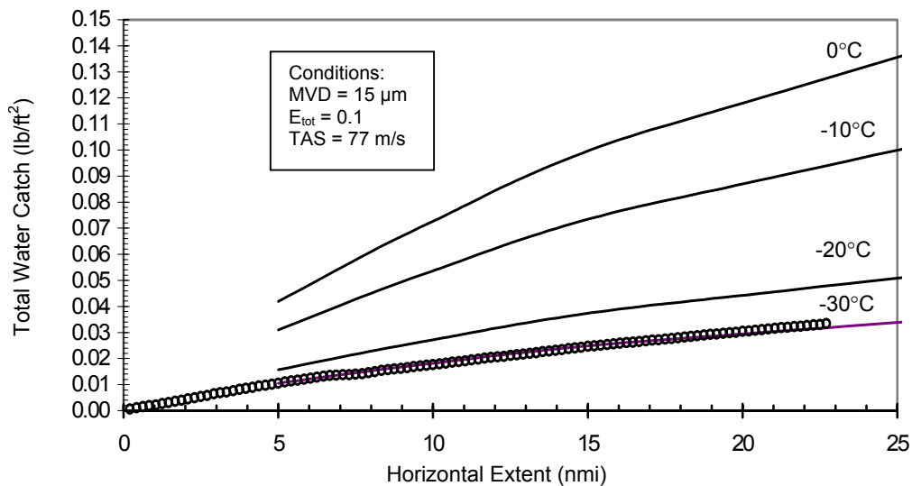
FIGURE 18. TOTAL WATER CATCH (TWC) FOR SAMPLE EXPOSURE (CLOUD GAP REMOVED) COMPARED WITH CONTINUOUS MAXIMUM, APPENDIX C, CONVERTED TO TWC ENVELOPES (For the conditions shown)
