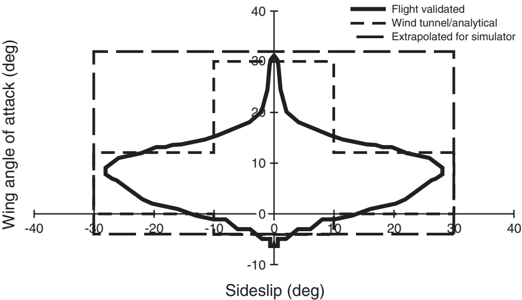
777 Alpha/Beta Envelope
