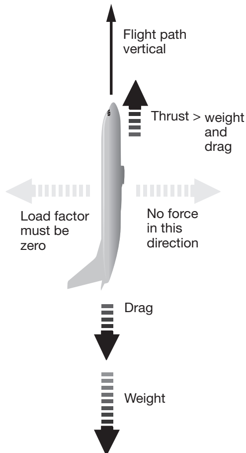
Figure 13a Airplane Vertical With Forces Balanced
