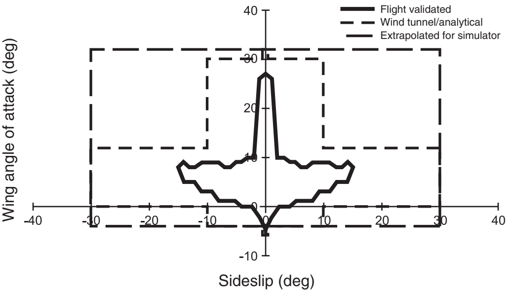
777 Flaps Up Alpha/Beta Envelope
