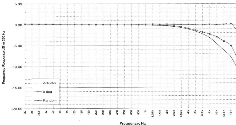
Microphone Frequency Response Type 4155 S/N 1138914 : Measured 31 Oct 2023
