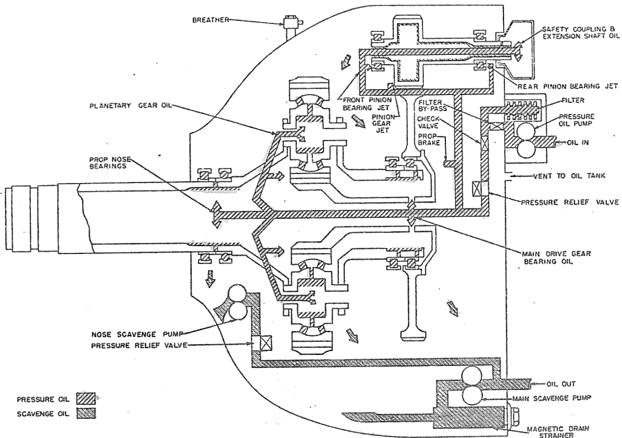
Reduction Gear Oil System Diagram
