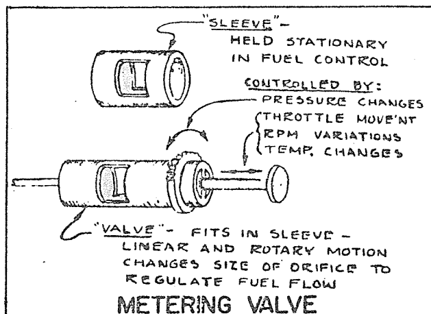
METERING VALVE
