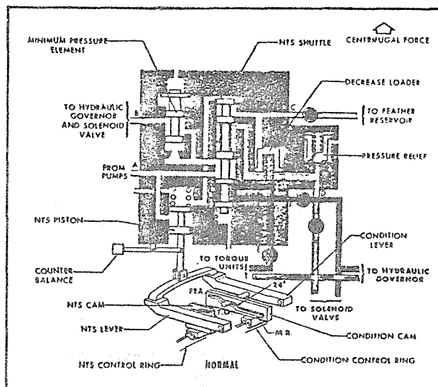
NTS FEATHER VALVE
