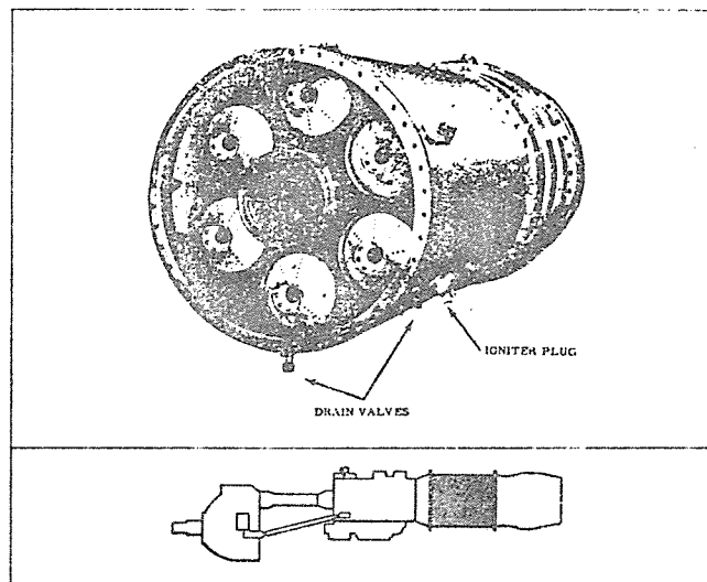
Combustion Chamber Assembly
