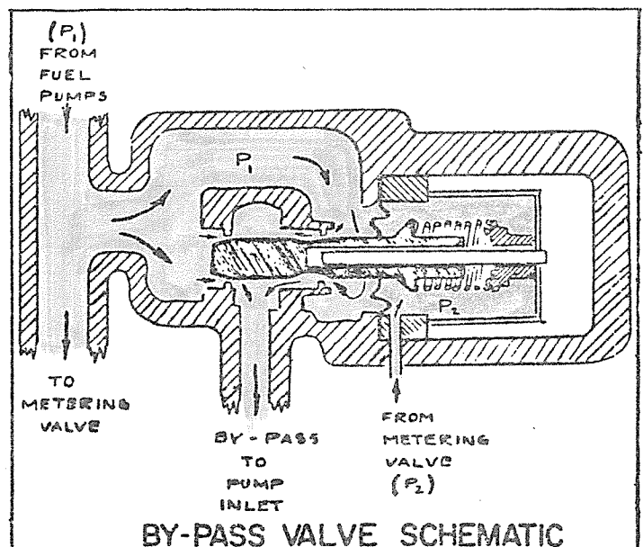
BY-PASS VALVE
