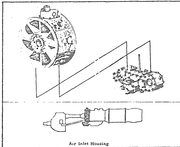
Air Inlet Housing
