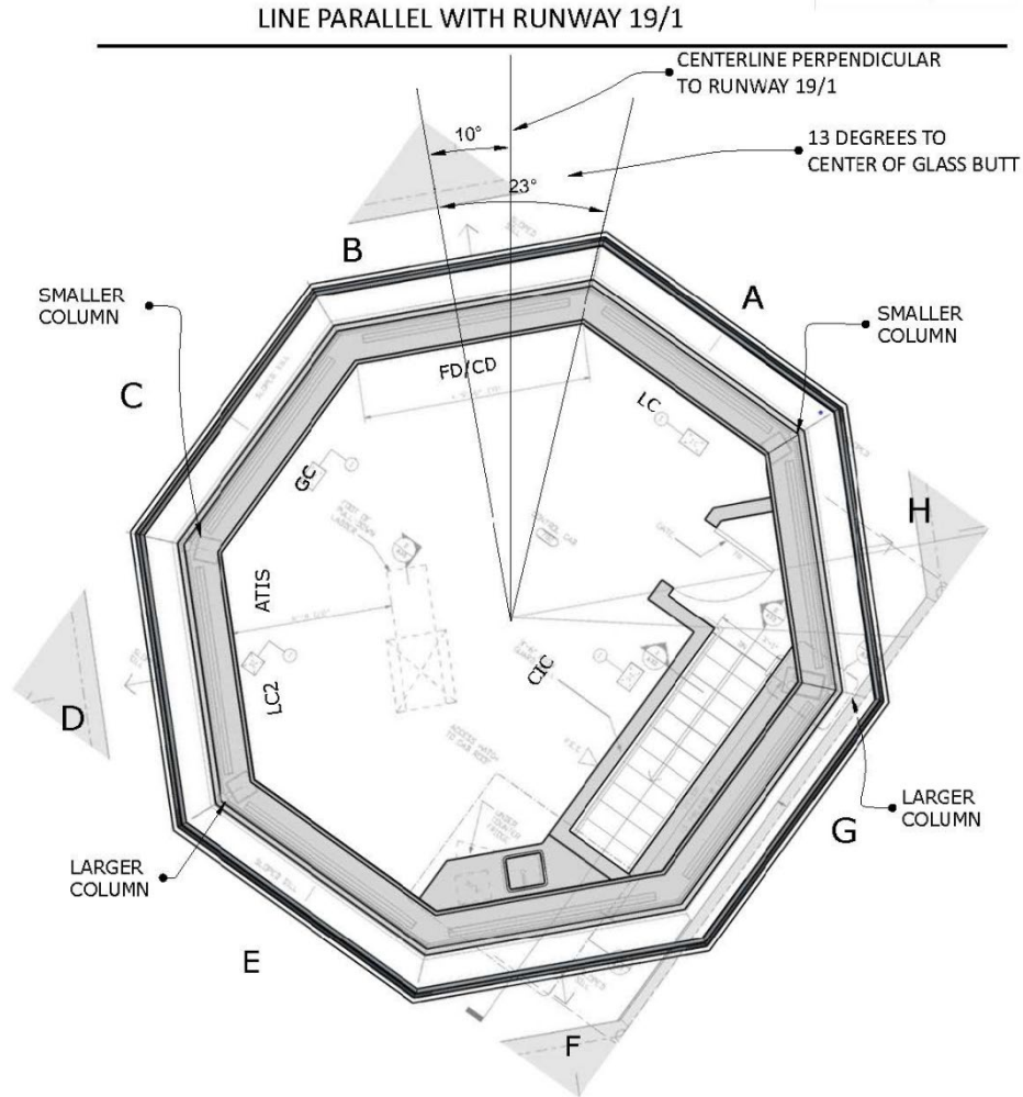
Figure 3-1. Proposed Layout of Replacement ATCT
